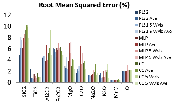
Figure 2: RMSE values for each combination of method and preprocessing steps for each major element.
