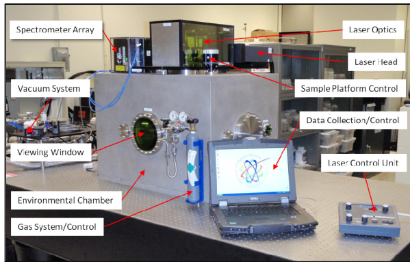
Figure 1: LIBS setup in the JSC Spectroscopy and Magnetism Lab.
