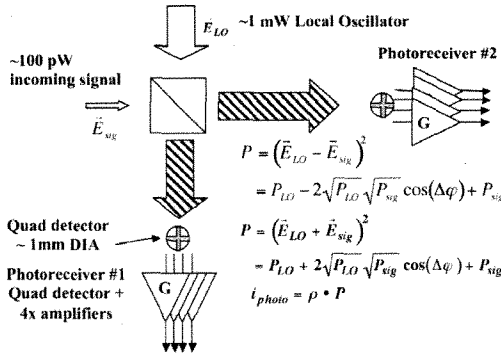
Figure 1. Descriptive diagram of laser heterodyne interferometric detection.
