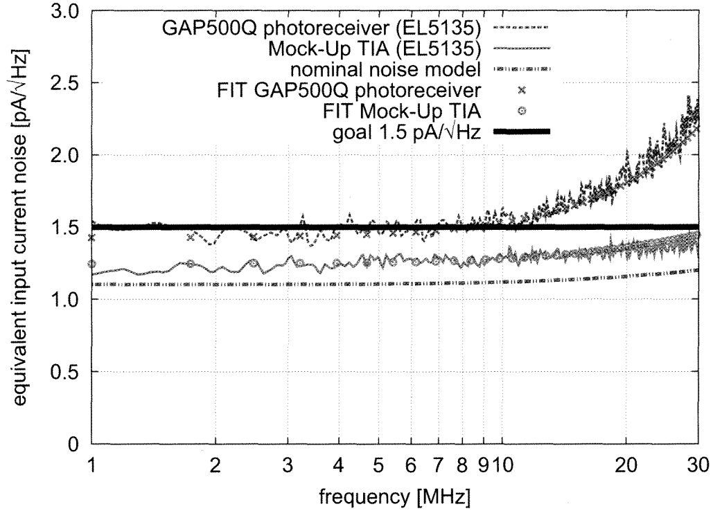
Figure 5. Input current noise measurements of photoreceiver prototypes. The dashed trace is the photoreceiver with one quadrant of the GAP500Q QPD and the EL5135 op-amp TIA. The solid trace is the mock-up test board (see Figure 4). The dashed-dotted trace is the photoreceiver noise model for a TIA design with an EL5135 op-amp and a quadrant capacitance of 2.5 pF (Equations 7). The traces with crosses and circles show the corresponding photoreceiver noise models using parameter values obtained from a fit to the data. The thick solid traced is our TIA input current noise goal of 1.5 \text{ pA}/\sqrt{\text{Hz}} in the measurement band 3-20 MHz.
