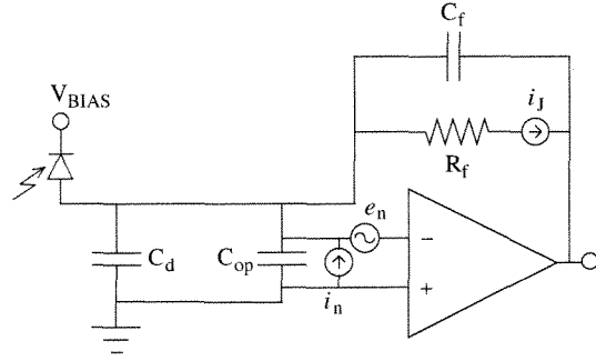
Figure 2. Topology and noise model of photoreceiver TIA.
