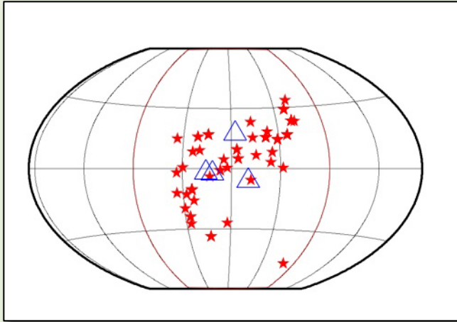
38 clusters with S picks
