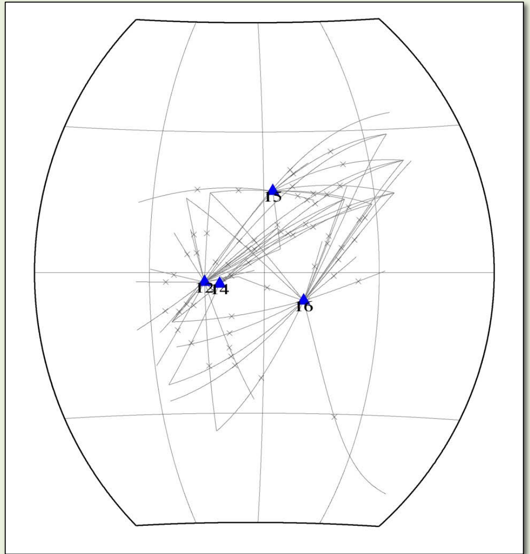
62 PcP ray paths for clusters with S picks bounce points shown for 300-km core
