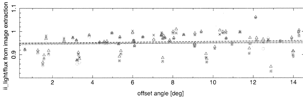
Figure 5: The ratio between averaged countrates for individual ScWs of the ii_light lightcurves with 10 s (triangle), (x) and 0.1 s (cicle) time resolution in the 20-40 keV energy band to the fluxes from the image extraction in dependency of the pointing offset angle of the science window.
