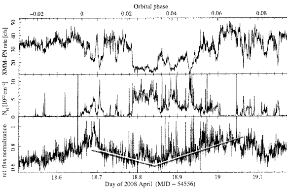
Figure 5: Absorption dips and scattering of X-rays as seen with XMM-Newton , EPIC-pn. a) The light curve in the energy band 0.3 – 10 keV shows absorption dips, which are identical to dips observed by Chandra shortly after \phi \approx 0 . b) Hydrogen column density of the neutral absorption model increases strongly when dips occur. c) Relative flux normalization constant, which is consistent with the scattering trough seen in hard X-rays (11).
