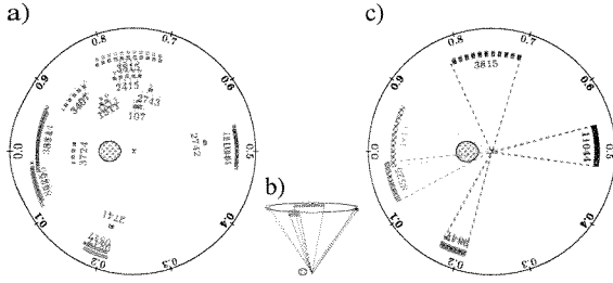
Figure 2: a) Polar view of the Cyg X-1 orbit and illustration of observation coverage with Chandra . Before 2010, January, there were 13 observations available, mostly covering the part of the orbit around phase \phi \approx 0 . Another observation (ObsID 11044) was obtained at \phi \approx 0.5 . A short observation (ObsID 2742) was the only one at this phase before, but since it was obtained in TE mode during the soft state of the source, it strongly suffered from pile-up. Full lines (dashed lines) display TE mode (CC mode) observations. Changes from blue to red colour correspond to changes from hard to soft state. b) Colorcoded orbital phases corresponding to lines of sight towards Cyg X-1 taking into account an inclination of \sim 35^\circ . c) Highlighted observations at phases of \phi \approx 0.0 (ObsID 3814 and ObsID 8525), 0.2 (ObsID 9847), 0.5 (ObsID 11044) and 0.75 (ObsID 3815), which are analyzed and compared in this work.
