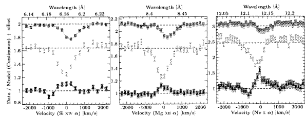
Figure 6: Absorption and P Cygni profiles of Si xiv, Mg xii and Ne x. While the observations at \phi \approx 0 and \phi \approx 0.75 show clear absorption profiles, although redshifted for \phi \approx 0.75 , the observation at \phi \approx 0.5 shows emission at v_{\text{rad}} \approx 0 and blueshifted absorption.
