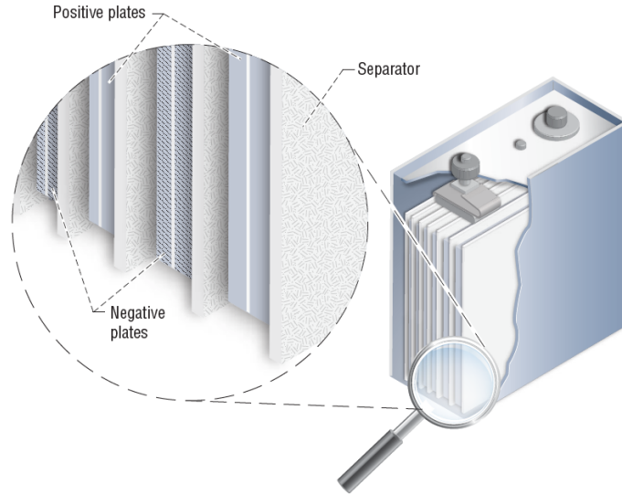
Figure 4.—Schematic showing components within a battery cell: negative plates (anode), positive plates (cathode), and separator. Electrolyte fills the void between electrodes.
