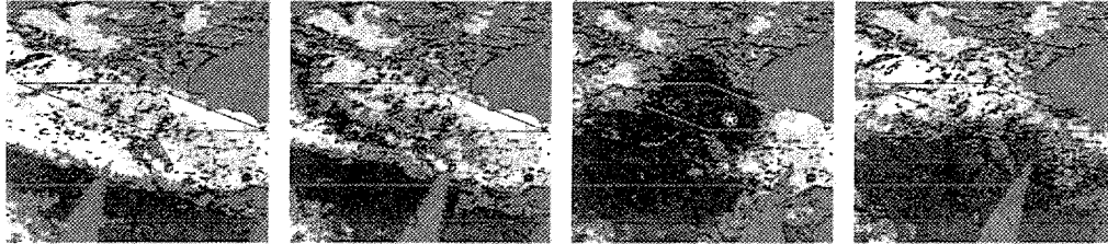
Figure 4. Sequence of AMSR-E SWE maps, 25 km resolution, of the boreal forest study area (black polygon) over the time of the probable wet snow event. (From left to right, A,B,C,D.) Dates shown are A) April 6, B) April 10, C) April 14, D) 19 April 2008, mapped in geographic projection. The star shows approximate location of Thompson Zoo, Manitoba weather station.
