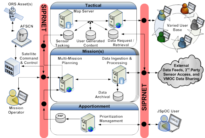
Figure 1.—VMOC system of systems.
