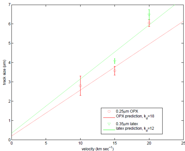
Figure 1 Track diameter as a function of projectile velocity. The fitting function used here is D_{\text{track}} = D_{\text{particle}} (K_d (v / 15 \text{ km/sec}) + 1) Note that this is a preliminary result of work in progress which will be updated on the conference.
