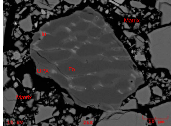
Figure 1. BSE image of 'Mg-Fragment 1' in 60016,93, composed of Fo 98 olivine (Fig. 2a), enstatitic pyroxene (Fig. 2b) and an interstitial component (In).
