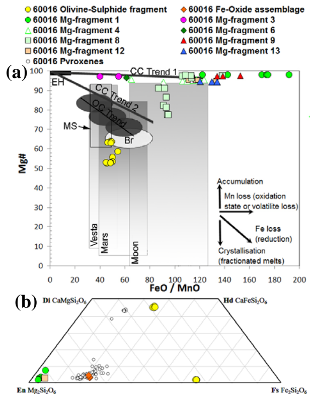
Figure 2. (a) Olivine FeO/MnO vs. Mg# of unusual clasts in 60016 (sections 83, 93 and 95) compared with olivines in Apollo samples and different meteorite groups. OC = ordinary chondrites, CC = carbonaceous chondrites, EH = enstatite chondrite, Br = brachinites, MS = mesosiderites. Meteorite data taken from range of sources including [6]. Mn values in several of the 60016 clasts are very low (<0.03 MnO), but long instrument count times (300 s) and high beam current (20 KeV, 40 nA) were used to analyse these phases to ensure low detection limits. Note that Mg-fragment 8 has a very magnesian core with zoned rim with more typical lunar olivine compositions. (b) Pyroxene compositions in unusual clasts in 60016. Key is the same in both diagrams.
