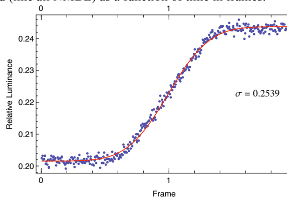
Figure 1. Example of NMBE (blue points) with fitted Gaussian (red curve). Luminance is in fractions of the peak display luminance. The estimate of sigma is shown. This particular waveform is from a transition between graylevels 139 and 150, for DUTID 001 and LMDID 616000.
