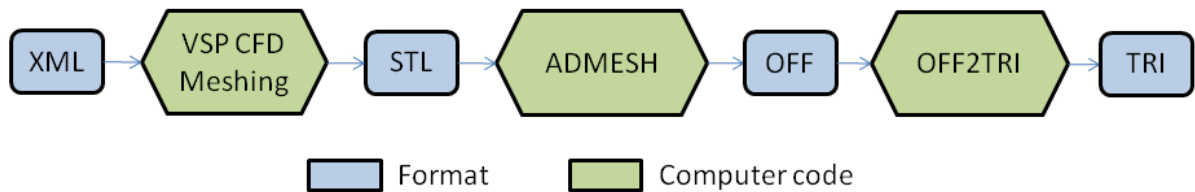
Figure 2. Geometry process to convert XML to Cart3D triangulated surface.
