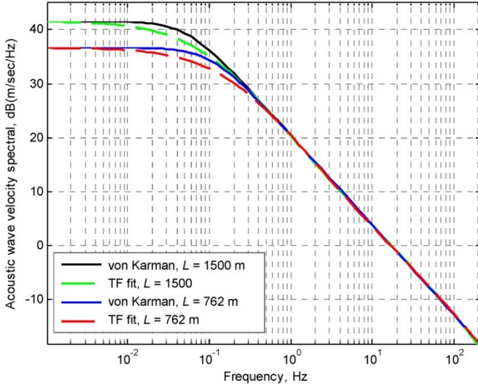
Figure C.9.—Von Karman acoustic wave velocity spectral due to temperature gust and its TF fits for different integral scale lengths ( \varepsilon = 8.6e-5 \text{ m}^2/\text{sec}^3 ).
