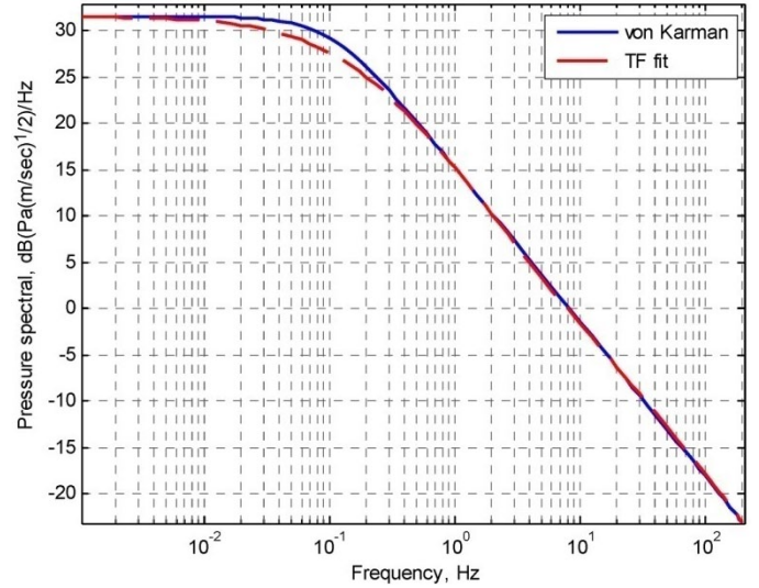
Figure C.11.—Pressure von Karman spectral and its TF fit ( \varepsilon = 8.6e-5 \text{ m}^2/\text{sec}^3 , L = 762 \text{ m} ).
