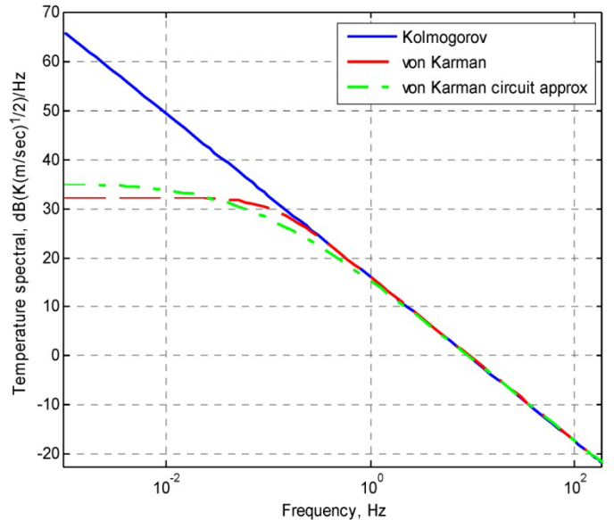
Figure B.7.—Kolmogorov and von Karman spectral for temperature and its von Karman circuit approximation ( \epsilon = 8.6e-5 \text{ m}^2/\text{sec}^3 , L = 762 \text{ m} ).
