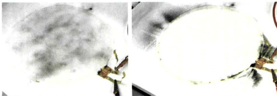
Fig. 6. Photographs of the 20-cm diameter transparent EDS for the PEM viewport during laboratory tests. JSC-1A simulant dust was deposited in a relatively uniform fashion, as shown on the left. The photograph on the right shows the EDS after activation. Dust has been removed to the region outside the electrode grid. These tests were performed with the EDS sitting horizontally in a glove box.
