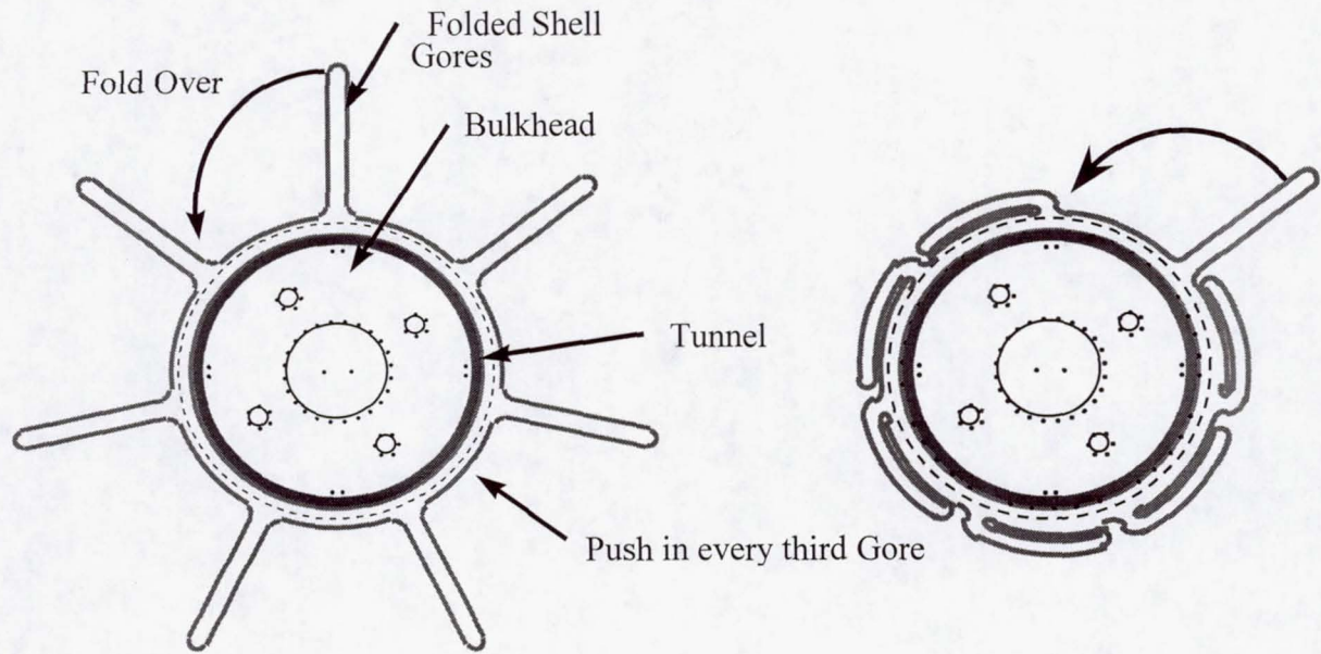
Figure 16: Folding Scenario
