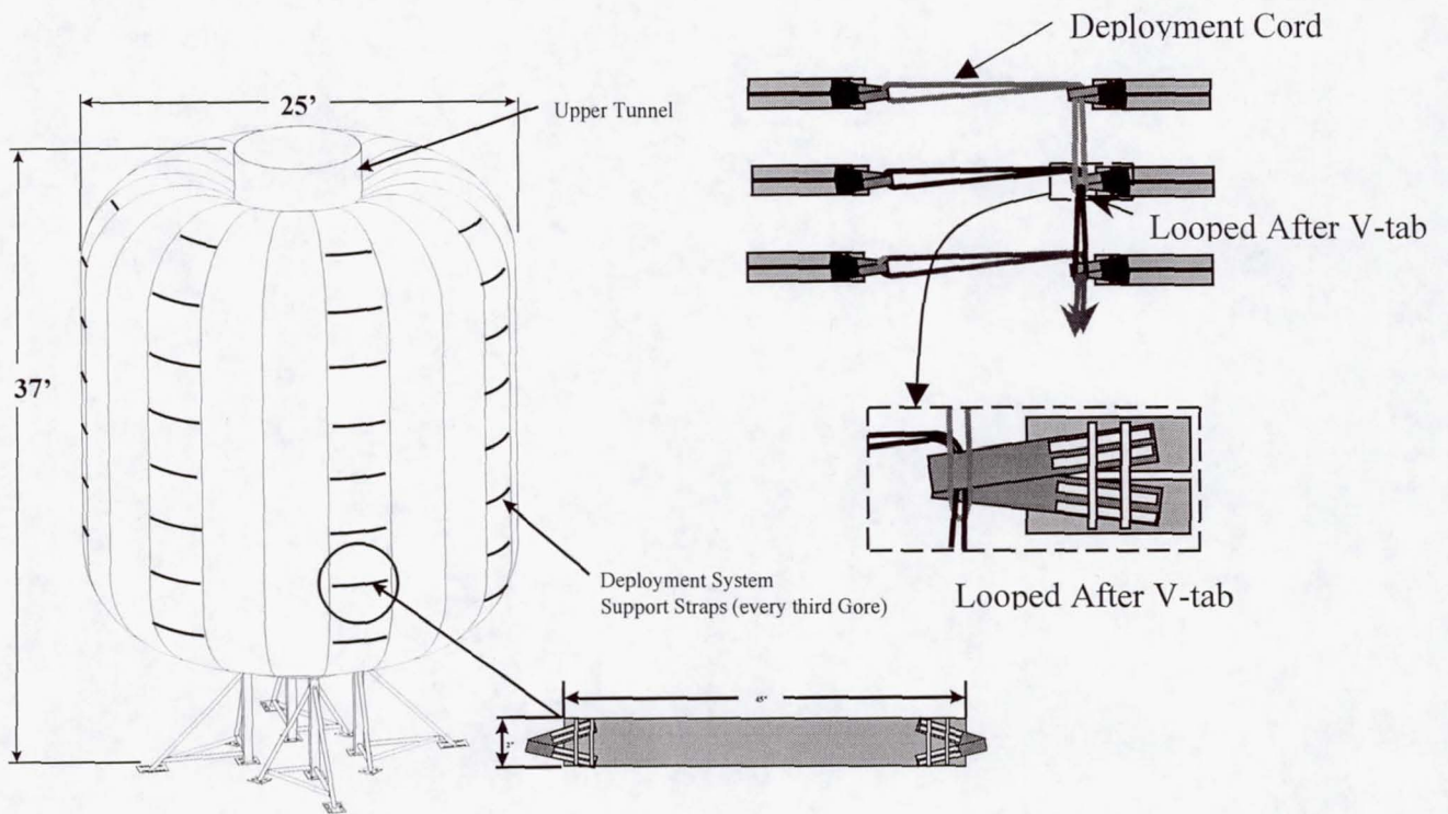
Figure 16: Folding Scenario
