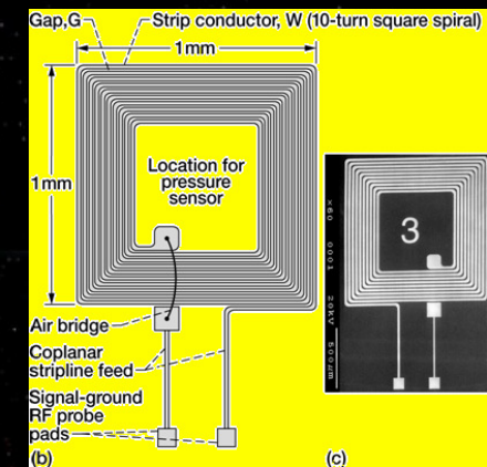
Schematic of miniature spiral inductor on SOG/HR-Si wafer and Photomicrograph of inductor/antenna.
