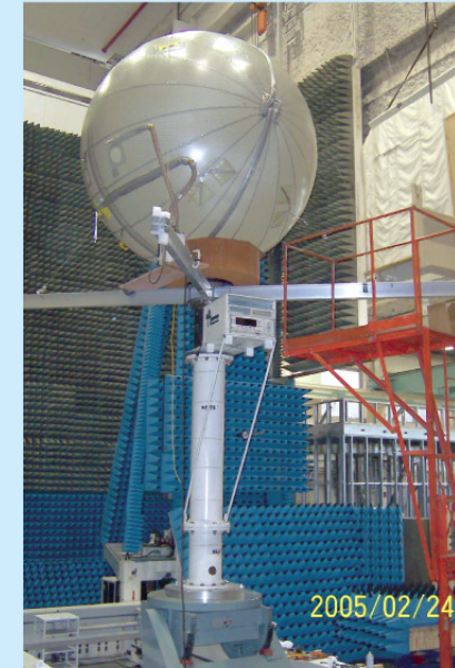
2.5-m inflatable membrane antenna in inflatable radome for ground applications
