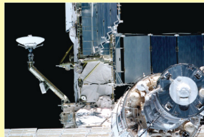
Backup 2-m inflatable Cassegrain reflector for ISS Ku-band system
