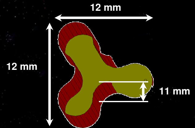
Compact Microstrip Monopole Antenna
