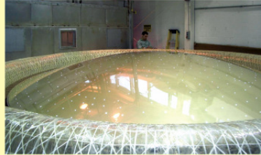
4- by 6-m inflatable offset parabolic membrane antenna inflation test (human in the background)
