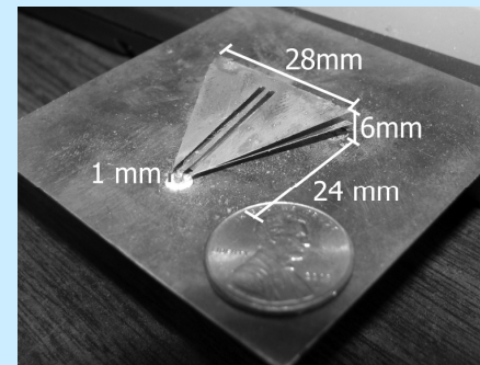
Prototype Miniaturized Antenna
