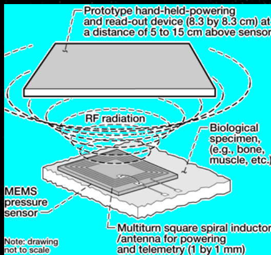
Contact-less powering and telemetry concept
