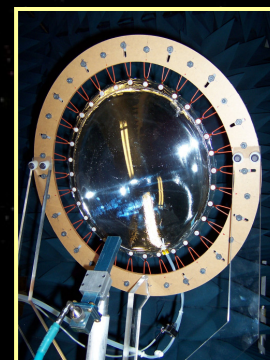
4 x 6 m offset parabolic
