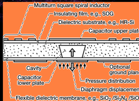
Schematic of a capacitive pressure sensor.
