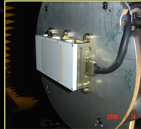
32 element breadboard proof-of-concept
