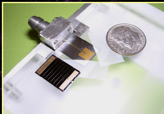
X-band Integrated antenna/solar cell
