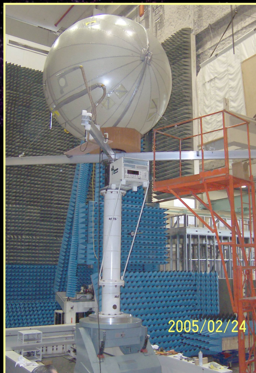
2.5 m "Beach Ball" Antenna
