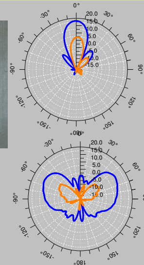
Reconfigurable antenna array (with 16 shorting wire switches)
