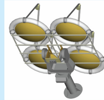
Low-cost tracking ground station experiment in collaboration with Goddard Space Flight Center planned for May 2005
