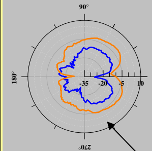
Single element on cube
