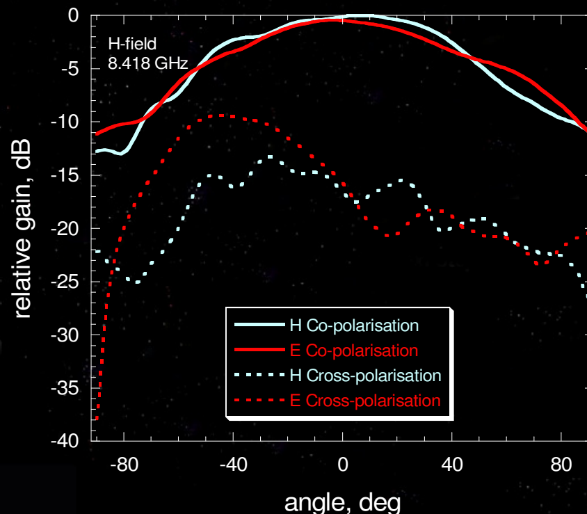
X-band Integrated antenna/solar cell
