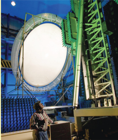
4- by 6-m inflatable offset parabolic membrane antenna test in GRC near-field facility
