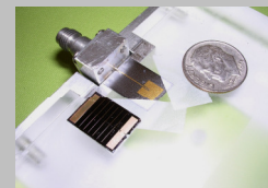
Solar Cell Integrated Antenna
