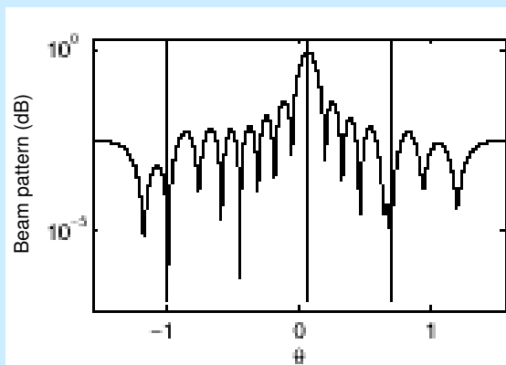
Simulated Beam forming Achieved Using Bayesian Estimation Method For a Random Sensor Array
