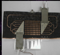
Multibeam Antenna
