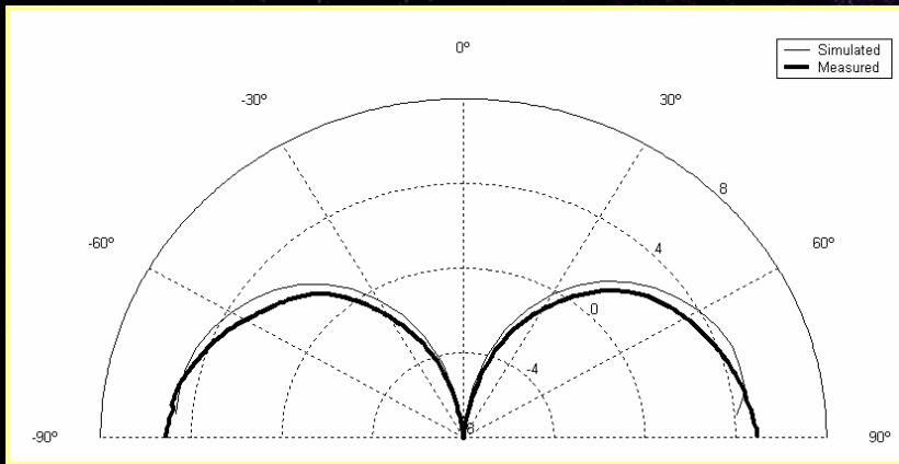
E-plane Pattern
