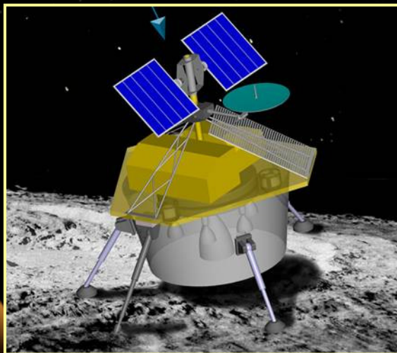
Robotic Lunar Lander
