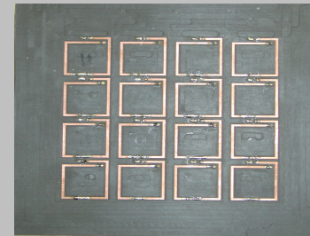
Reconfigurable antenna array (with 16 shorting wire switches)
