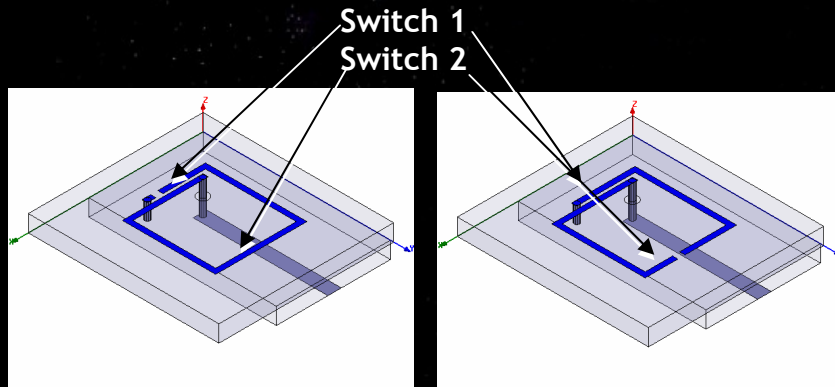
Single element on cube
