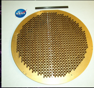
Reflectarray Antenna SCDS 615 Element Prototype + Ka-Band Space Qualifiable
