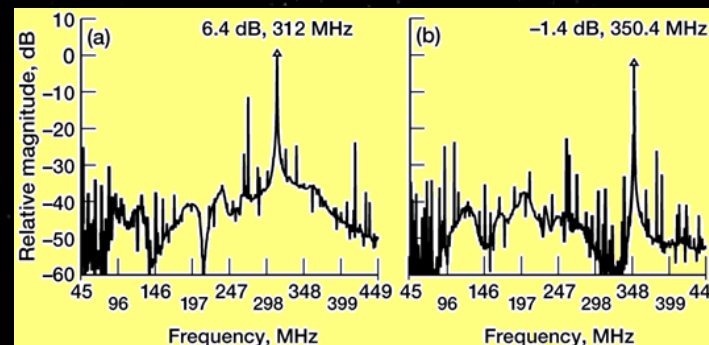
Measured received relative signal strength as a function of frequency. (a) Pick-up antenna at a height of 5 cm. (b) Pick-up antenna at a height of 10 cm.
