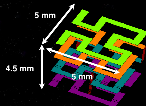
Folded Hilbert Curve Fractal Antenna
