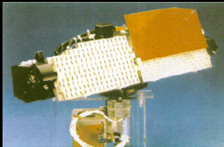
Mechanically steered Array proof-of-concept
