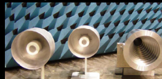
TDRS C Candidate Cup Waveguide
