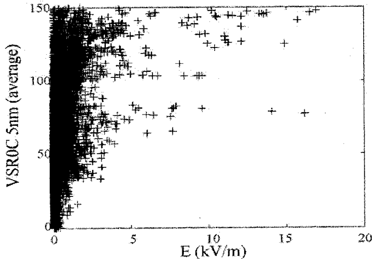
Figure A4-2. Scattergram of 'VSR0C' averaged within 5 n mi vs. measured electric field
