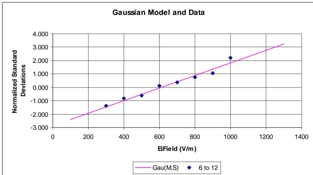
Figure A8-2. Probability distribution based on Fig. A8-1, from the Merceret Memo
