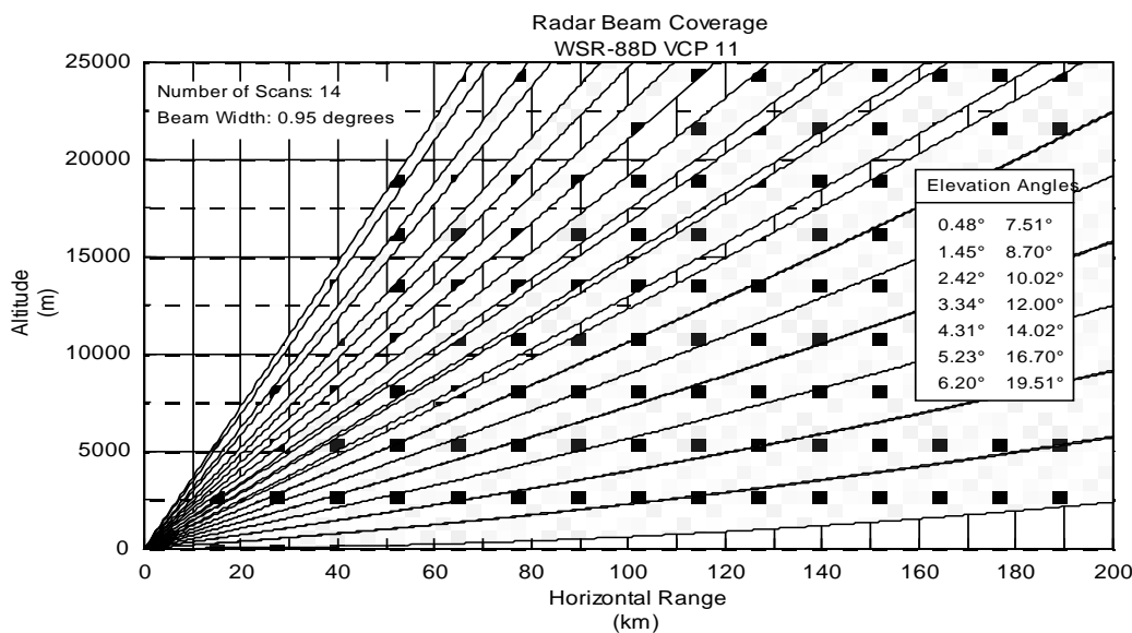
Figure A9.1. Radar beam coverage for 'Volume Coverage Pattern 11' of the WSR-88D radar
