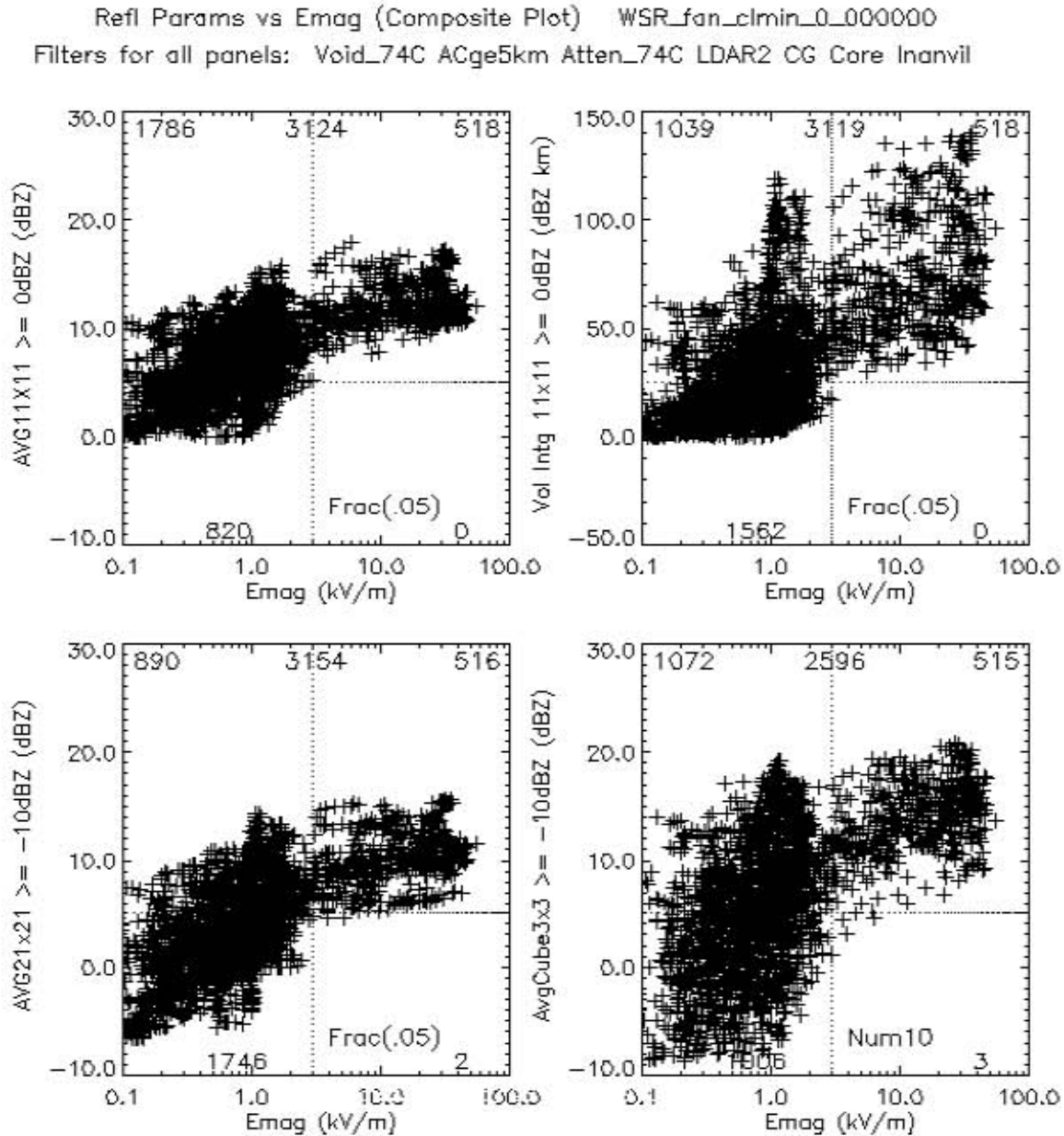
Figure A7-2. Scattergrams of electric field magnitude (Emag) vs. four different radar-reflectivity parameters
