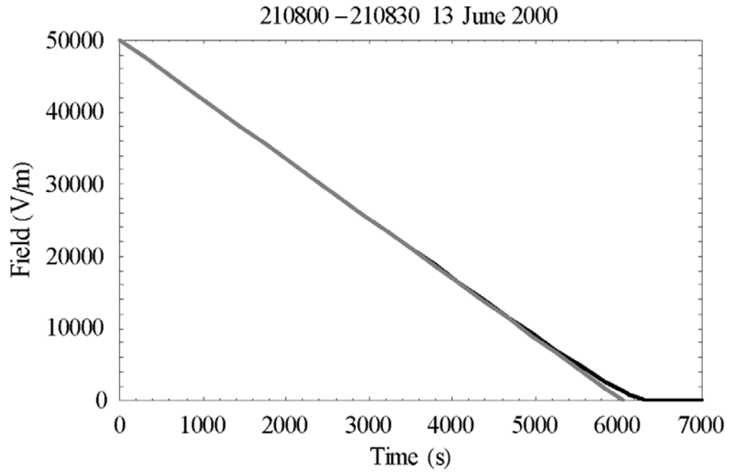
Figure A6-3. Model electric-field decay from 50 kV/m
