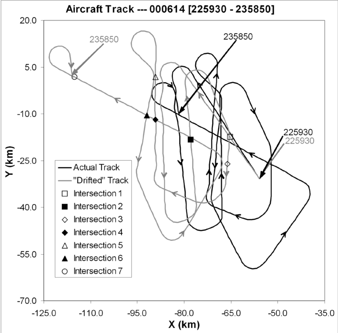
Figure A6-9. Actual (black) and "drifted" (gray) aircraft tracks
