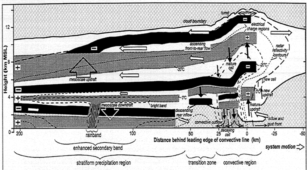
Figure A3-13. Sketch of the charge structure in an idealized MCS (from Stolzenburg et al., 2001)
