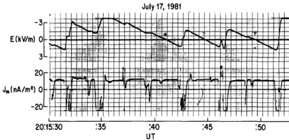
Figure A1-17. Surface potential gradient and total Maxwell current density
