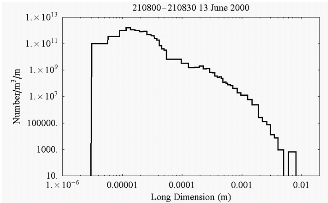
Figure A6-2. Composite particle-size distribution in a dense anvil
