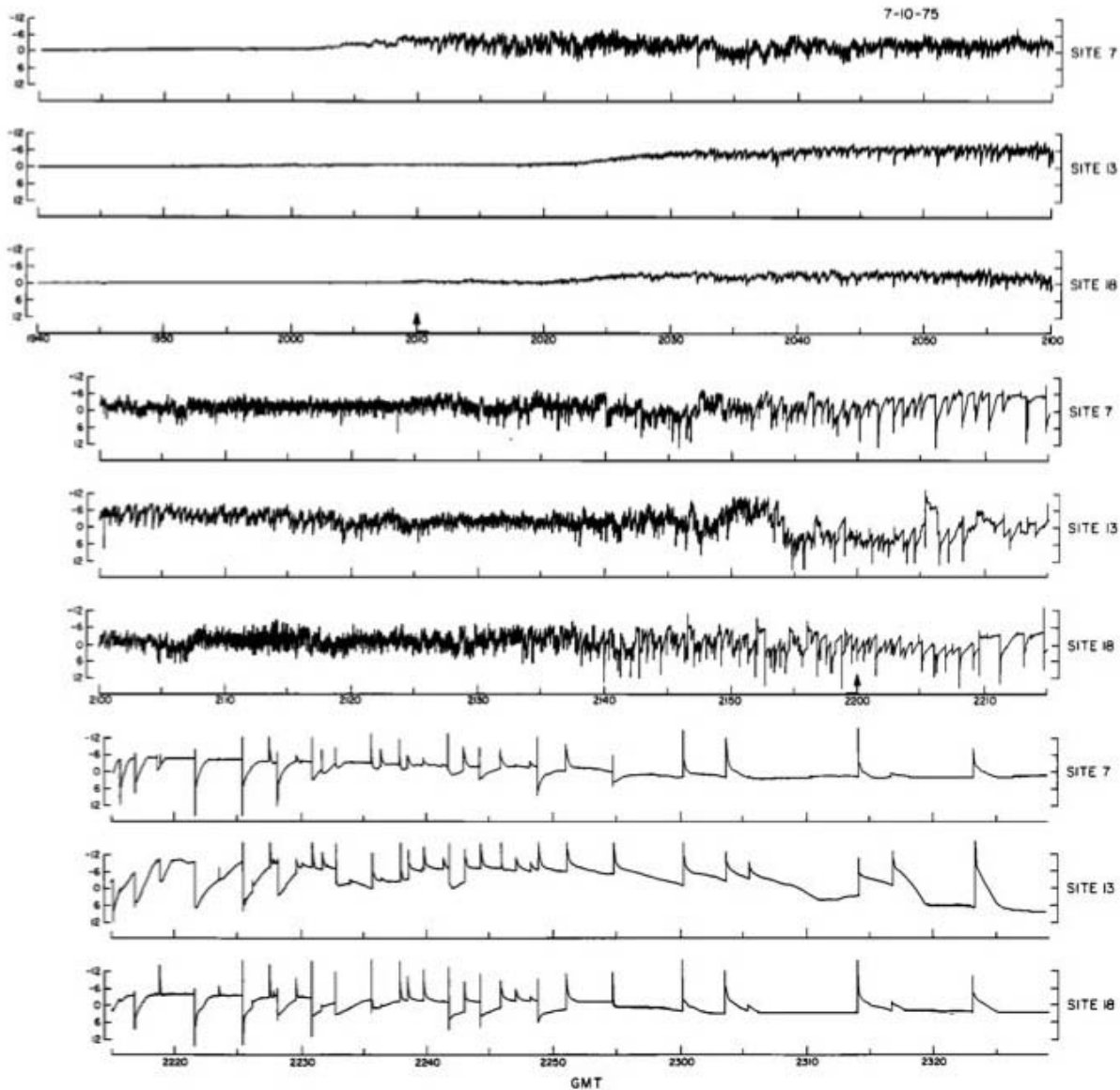
Figure A1-12. Evolution of potential gradients during a very large storm
