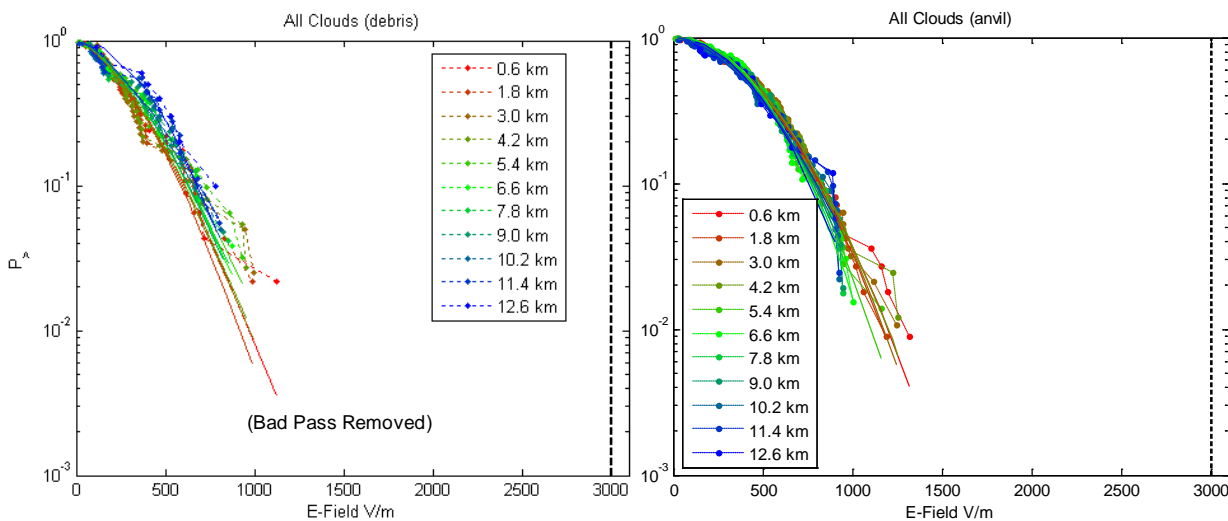
Figure A8-3. Probability distributions from Fig. A8-1, with extreme value analysis
