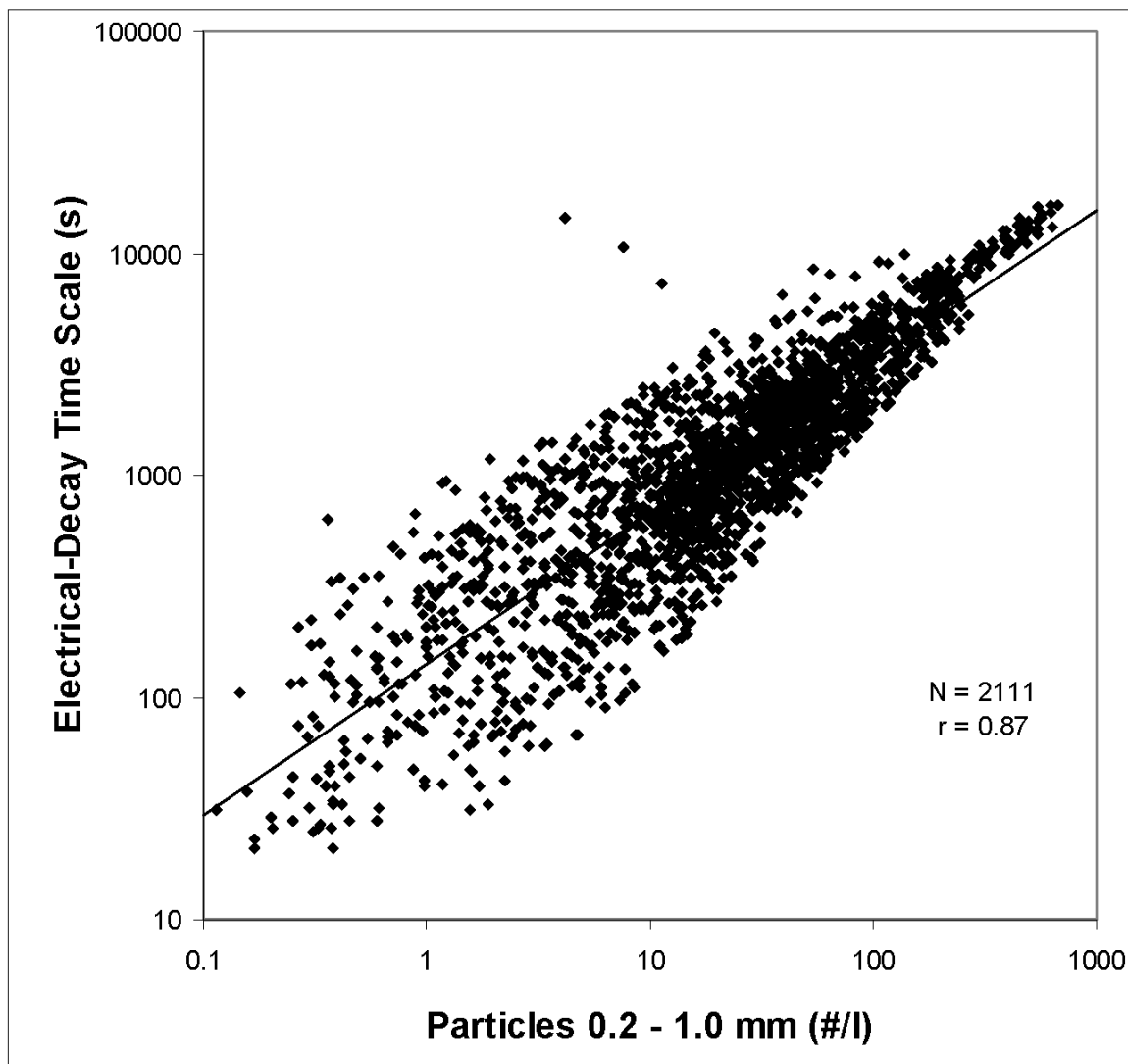
Figure A6-5. Scattergram of 'electrical decay time scale,' \tau_E , vs. particle concentration
