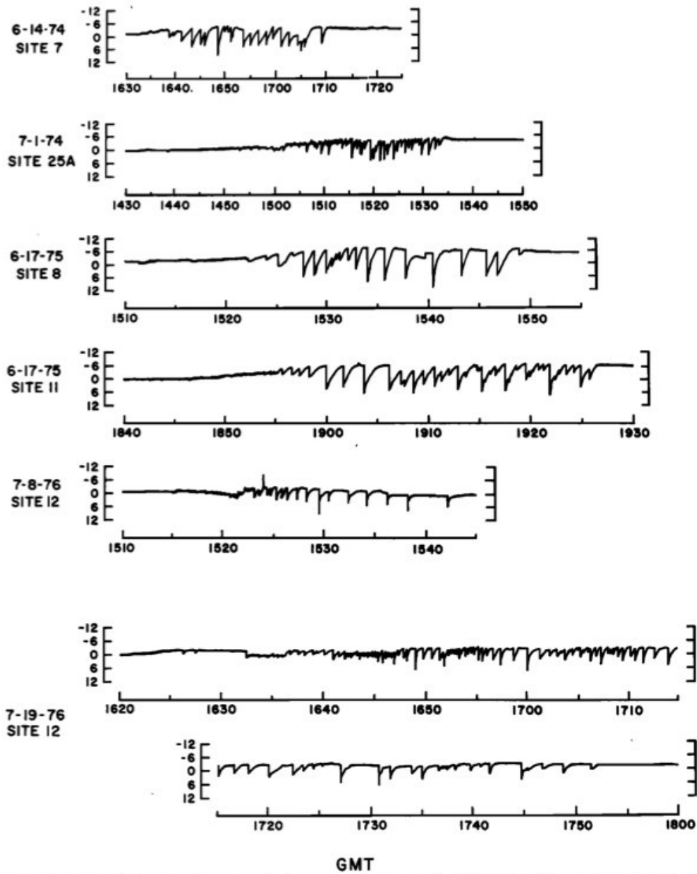
Figure A1-10. Potential gradients beneath six small storms
