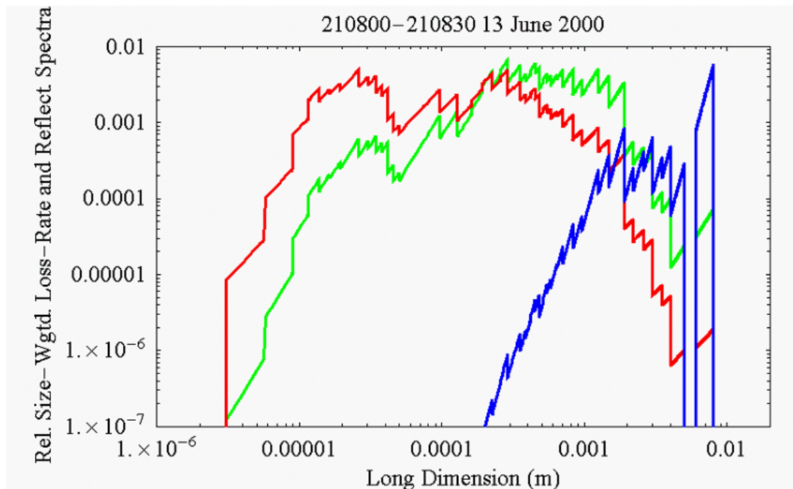
Figure A6-2. Comparison of diffusive and electrical small-ion loss rates with radar reflectivity as functions of particle size
