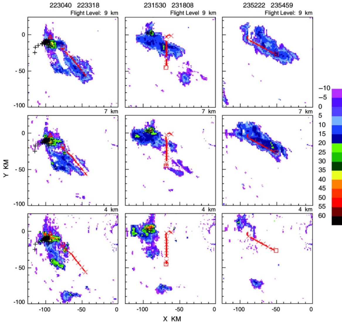
Figure A6-8. WSR-74C CAPPIs with lightning from the NCAR Web site
