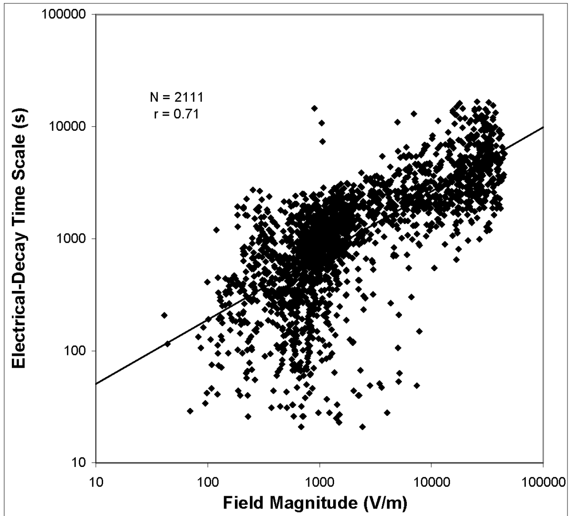
Figure A6-6. As in Figure A6-5 for \tau_E vs. the magnitude of electric field, |E|
