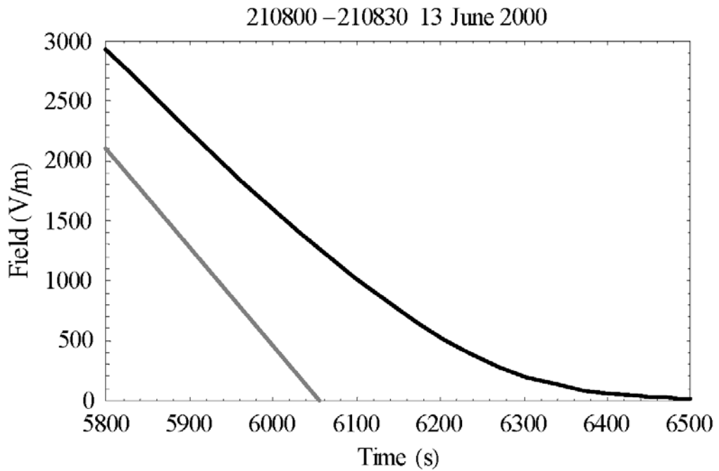
Figure A6-4. Enlargement of final decay shown in Fig. A6-3
