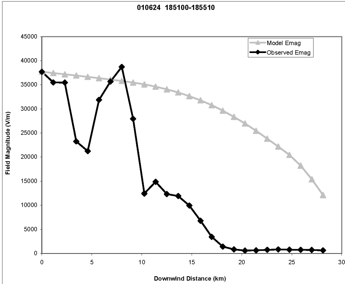
Figure A6-11. Observed vs. calculated field decay downwind
