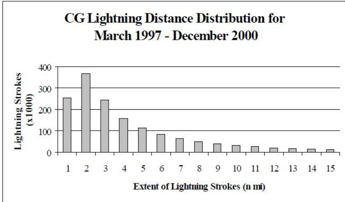
Figure A2-1. Histogram of horizontal distances between initial LDAR sources and ground strike points
