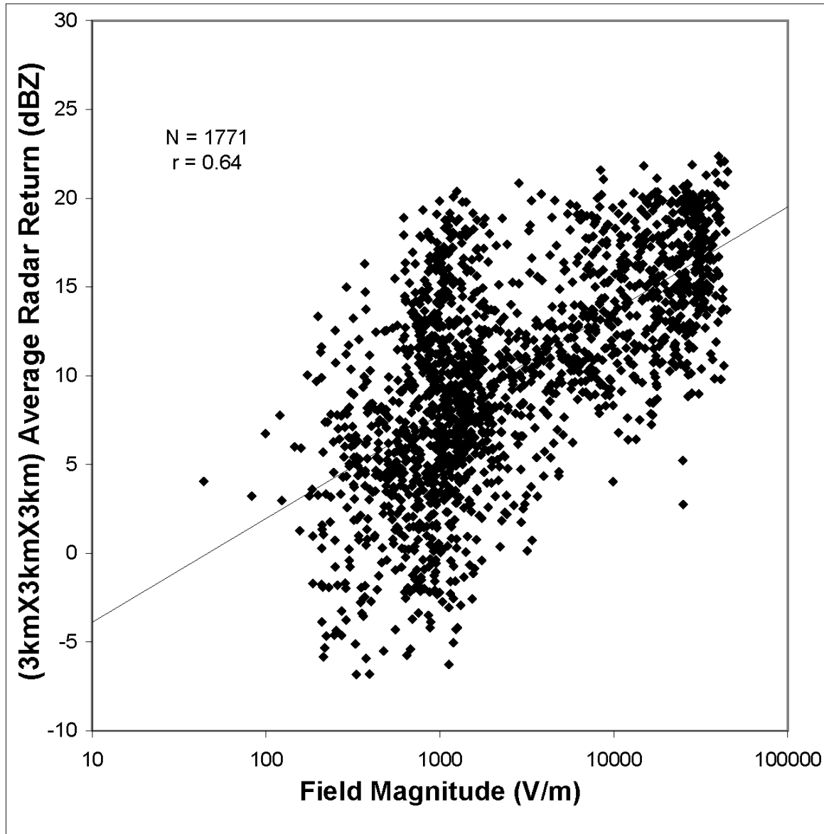
Figure A6-7. As in Figure A6-5 for (3 \text{ km})^3 average radar reflectivity vs. |E|
