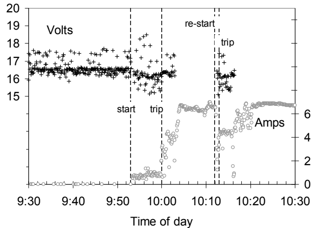
Figure 21.—Battery JPL2-1 voltage history on I-Suit.
