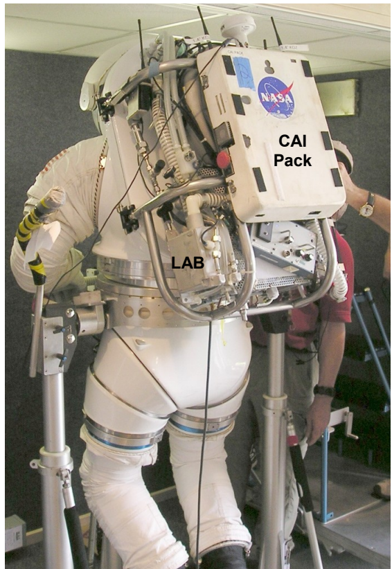
Figure 14.—LAB and CAI pack on Mark III suit.
