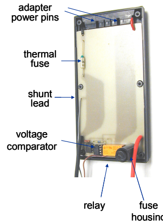
Figure 4.—Adapter plate with safety-system elements.
