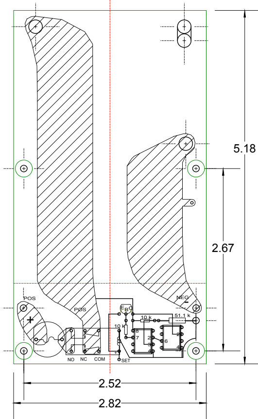
BOTTOM VIEW (copper side)
