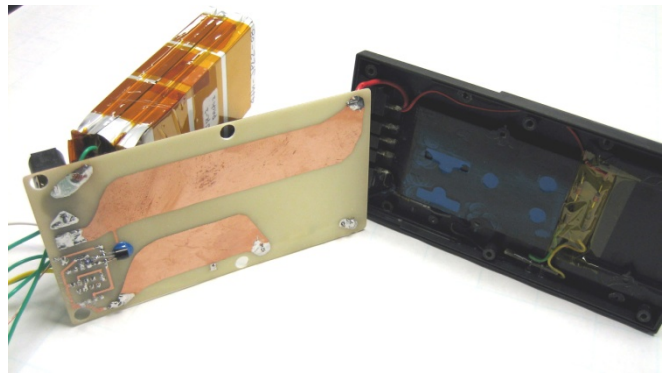
Figure 7.—Battery components soldered together.
