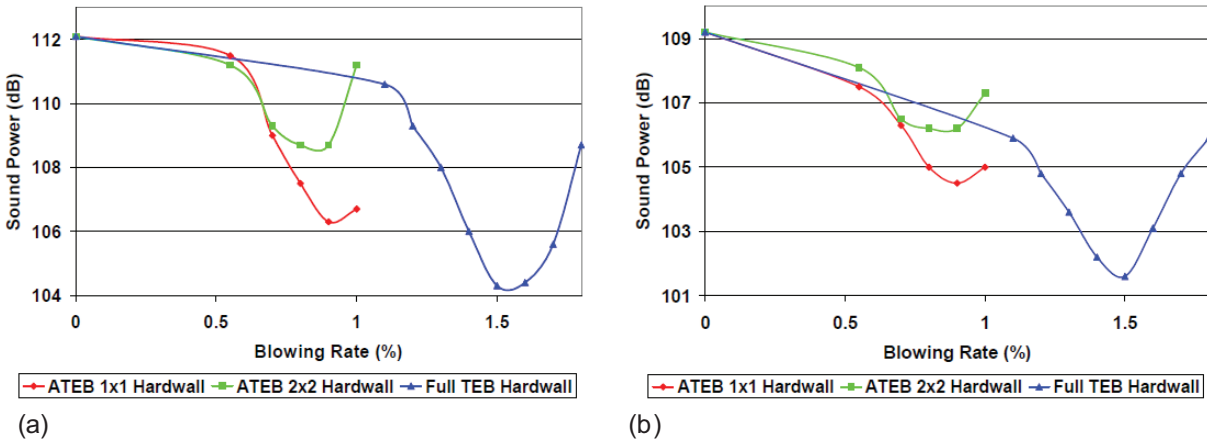
Figure B-1. Sound Power vs. Blowing Rate (% Inlet Flow Rate) for (a) Inlet Duct and (b) Aft Duct [Ref. 139]
