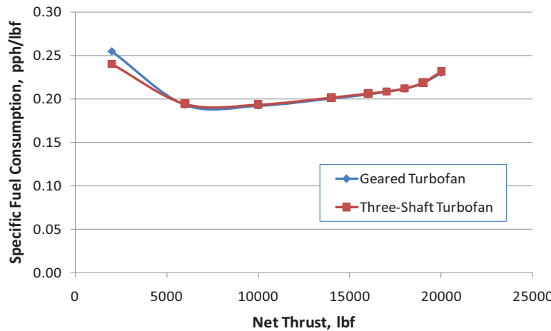
Figure 5-6. Geared Turbofan and Three-Shaft Turbofan SLS SFC Hook Comparison at Comparable Technology Level
