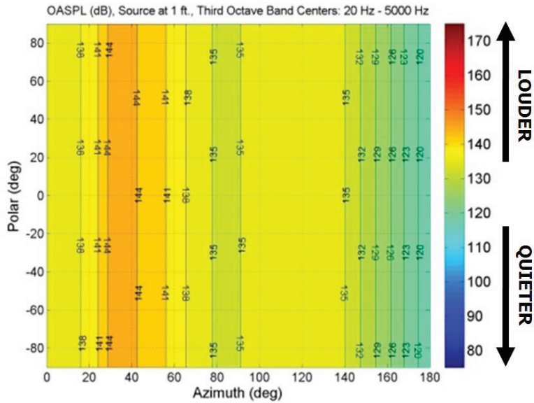
Figure D-1. OASPL Example Source Plot
