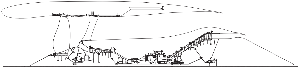
Figure 5-3. Three-Shaft Turbofan Mechanical Profile Diagram
