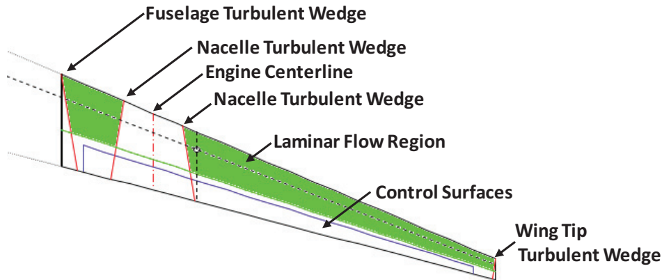
Figure 5-25. Laminar Flow Regions Visualization for High Aspect Ratio Wing
