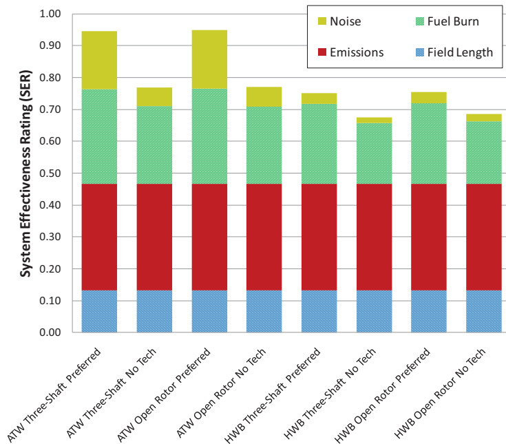
Figure 6-13. System Effectiveness Rating Comparison Between Candidate Configurations
