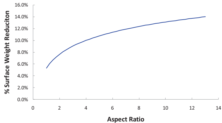
Figure 5-28. Surface Weight Reduction Through Aeroservoelastic Structures as a Function of Aspect Ratio
