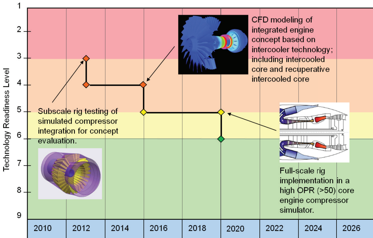
Figure 7-13. TMP for Intercooled Compressor Stage
