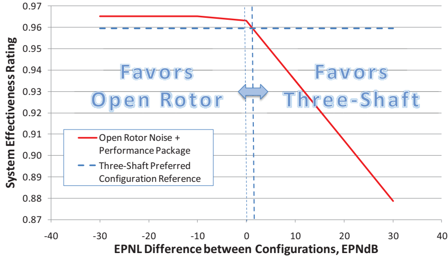
Figure 6-14. Effect of Configuration \Delta EPNL on System Effectiveness Rating
