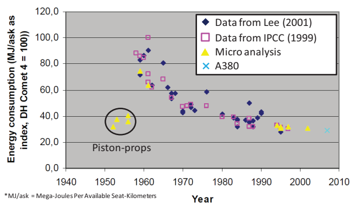
Figure 4-13. Commercial Aircraft Fuel Efficiency Historical Data Indicating Piston-Prop Performance [Ref. 26]
