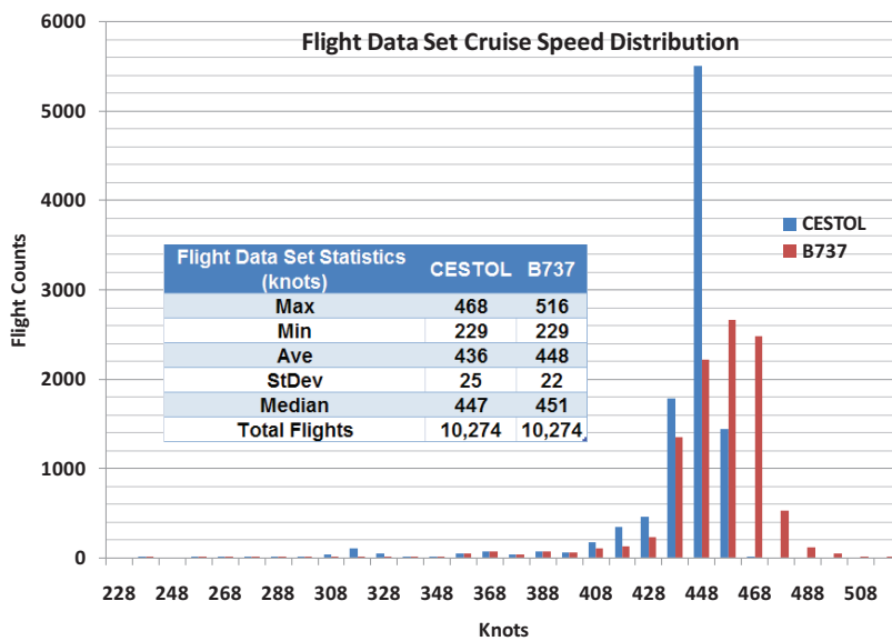
Figure 4-23. Cruise Speed Distribution Shift for an N+2 NAS Simulation Compared to Baseline 737 Distribution
