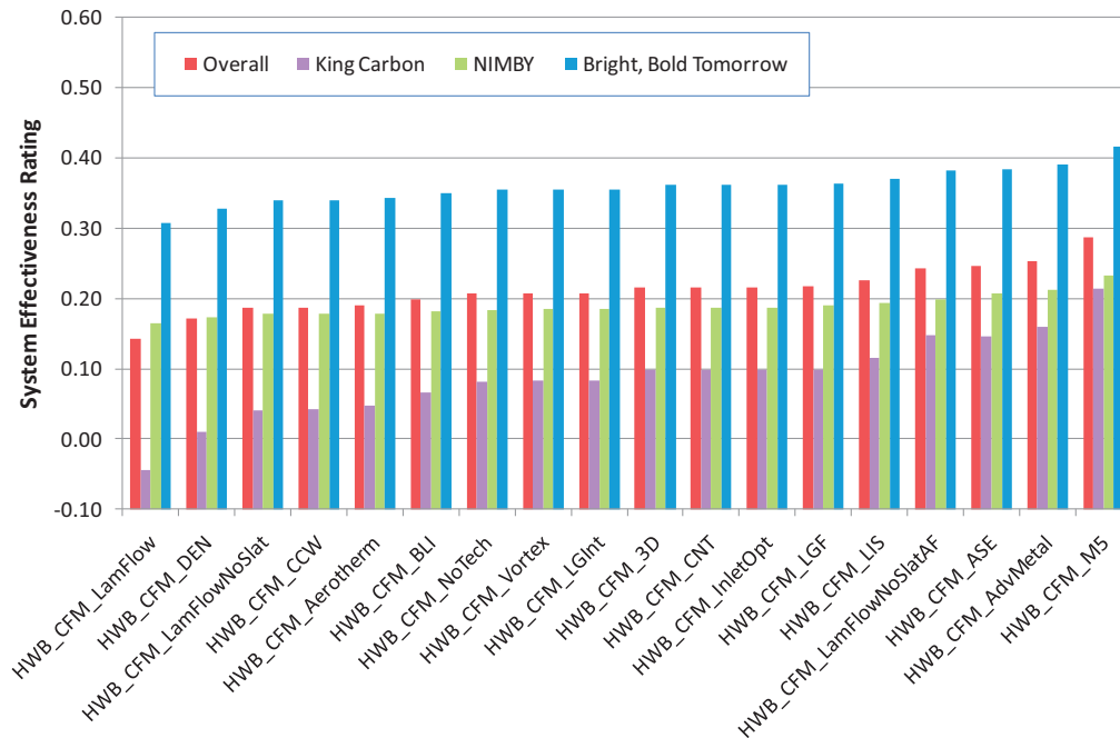
Figure 6-12. HWB Individual Technology Assessment
