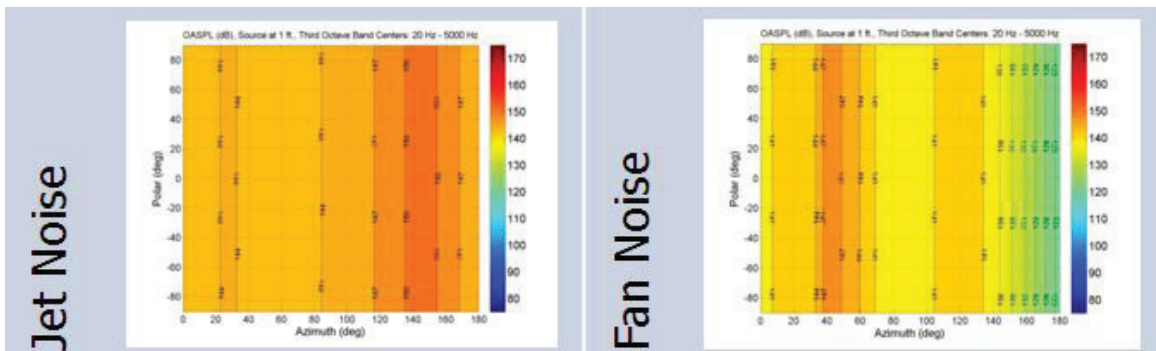
Figure D-5. Noise Source Levels ATW, Scaled CFM56-3B1, No Advanced Technologies at 250 feet Altitude [Takeoff-Climb]
