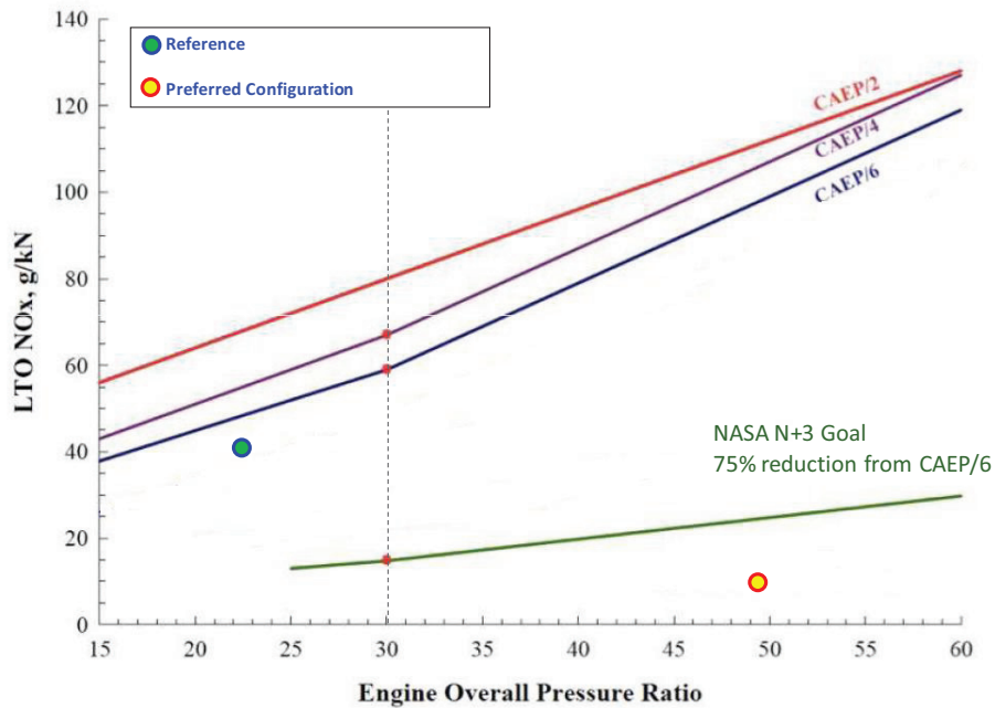
Figure 6-18. CAEP/6 LTO NOx Emissions Requirement and N+3 Achievements
