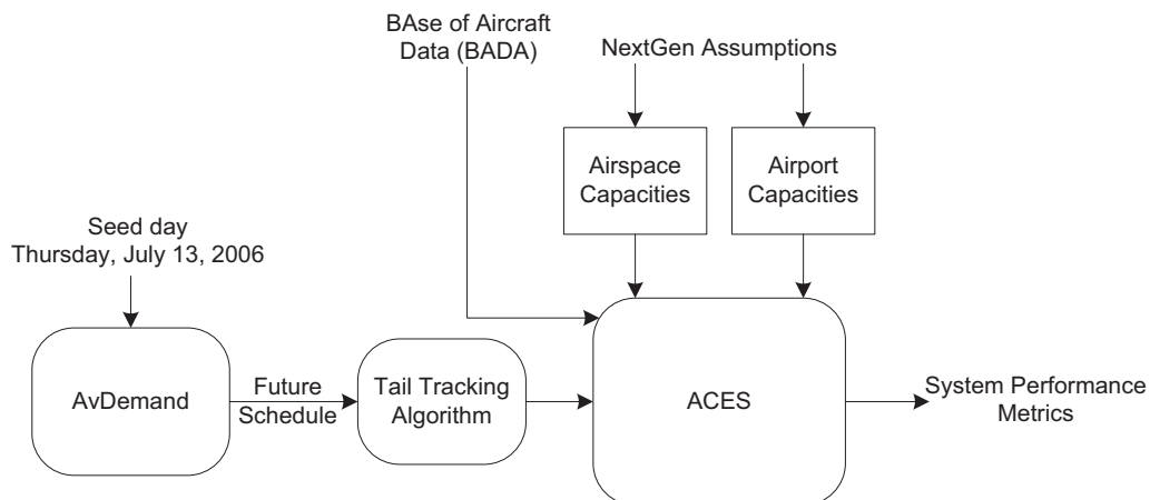
Figure 4-11. Simulation and Modeling Approach for This Analysis
