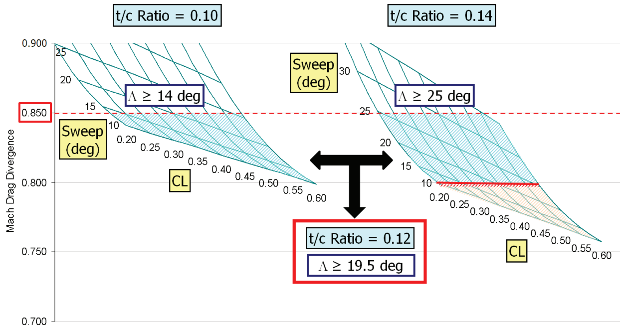
Figure 6-7. Initial Sizing Tube-and-Wing M_{DD} Sensitivity Study
