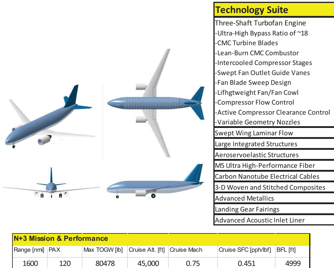
Figure 1-1. N+3 Preferred Configuration 3-View and Mission Performance
