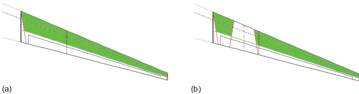
Figure 6-3. Wing Laminar Flow Extent for (a) Aft Fuselage Mounting, (b) Under-Wing Mounting
