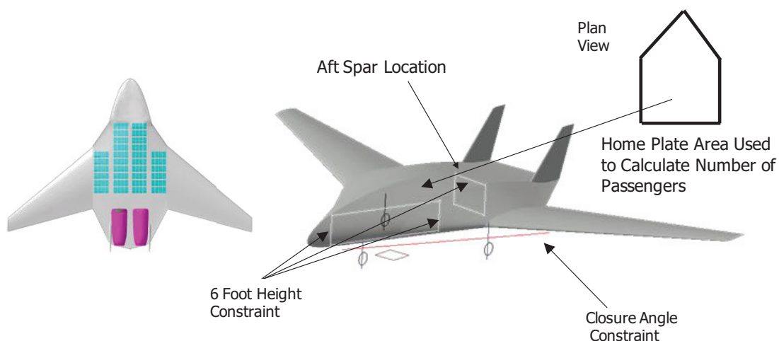
Figure 5-13. HWB With Embedded Propulsors Configuration
