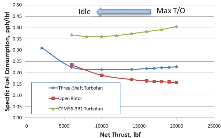
Figure 5-7. Engine Architecture SLS SFC Hook Comparison, Advanced Technology Level
