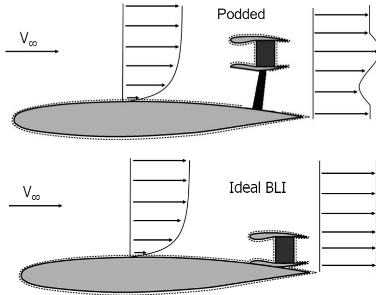
Figure 5-27. Aft Velocity Profile for Ideal BLI and Podded Propulsion Configurations
