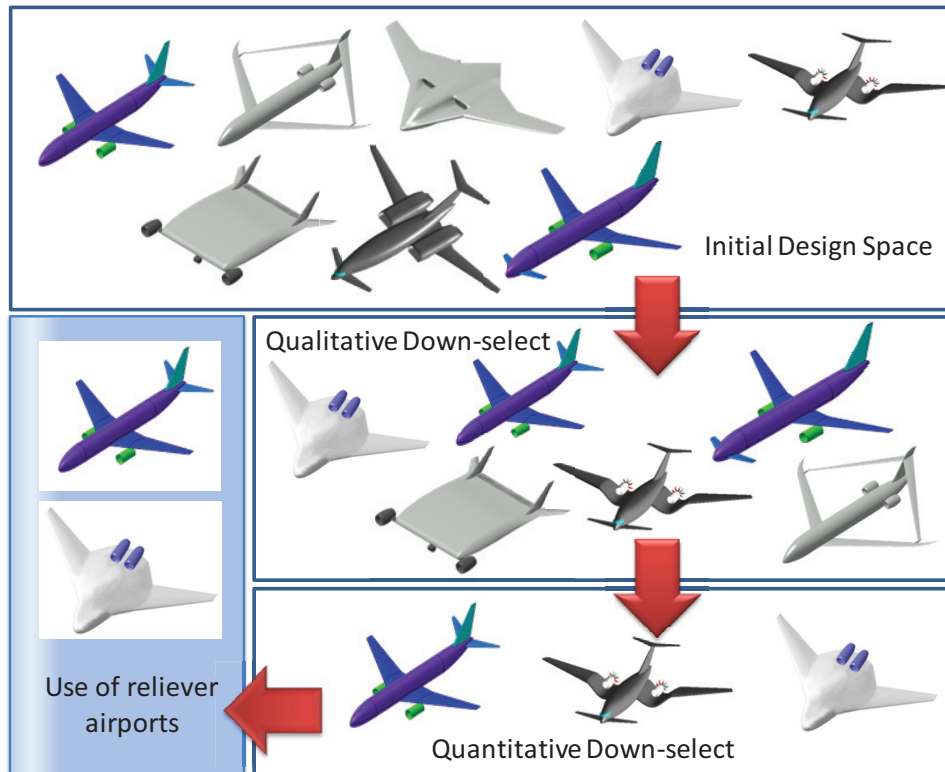
Figure 5-8 .Airframe Configuration Downselection Process
