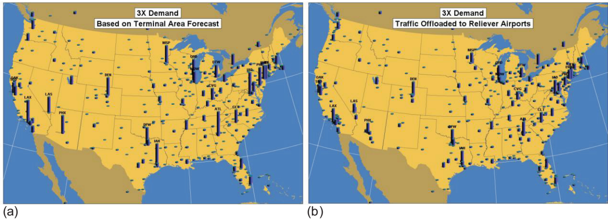
Figure 4-22. (a) Baseline Three Times Traffic Delay Distributions; (b) Metroplex Operations Delay With >5,000 foot Airfields
