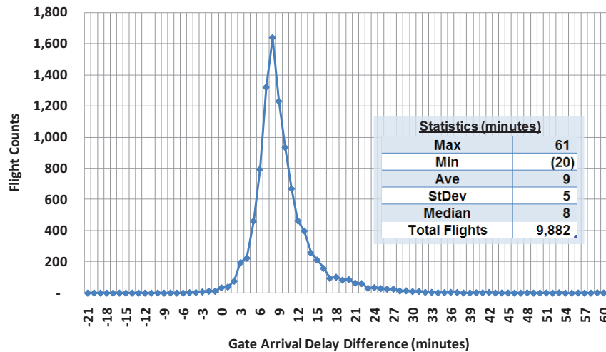
Figure 4-24. Aircraft Delay Distribution for a Cruise Speed Decrease of 12 Knots Compared to 737 for an N+3 Vehicle Study
