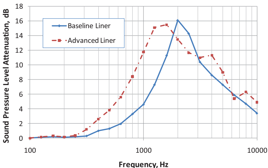
Figure 6-2. Baseline and Advanced Fan Duct Liner Sound Pressure Level Reduction
