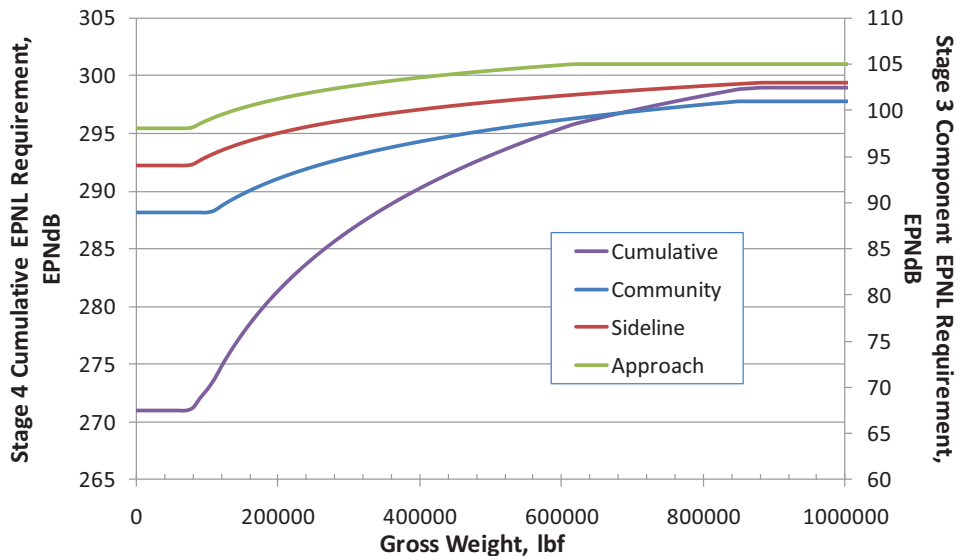
Figure 6-10. FAR Part 36 Stage 4 Cumulative EPNL Noise Requirements
