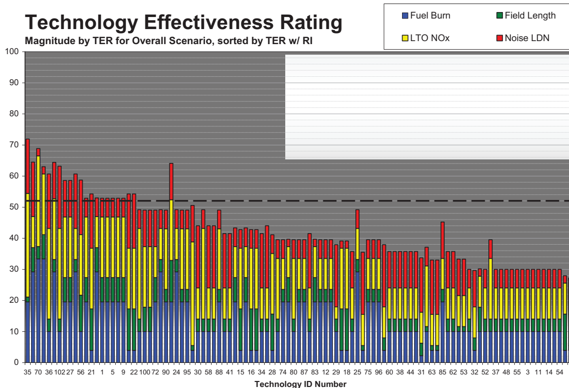
Figure 5-23. Technology Effectiveness Ratings for Overall Scenario
