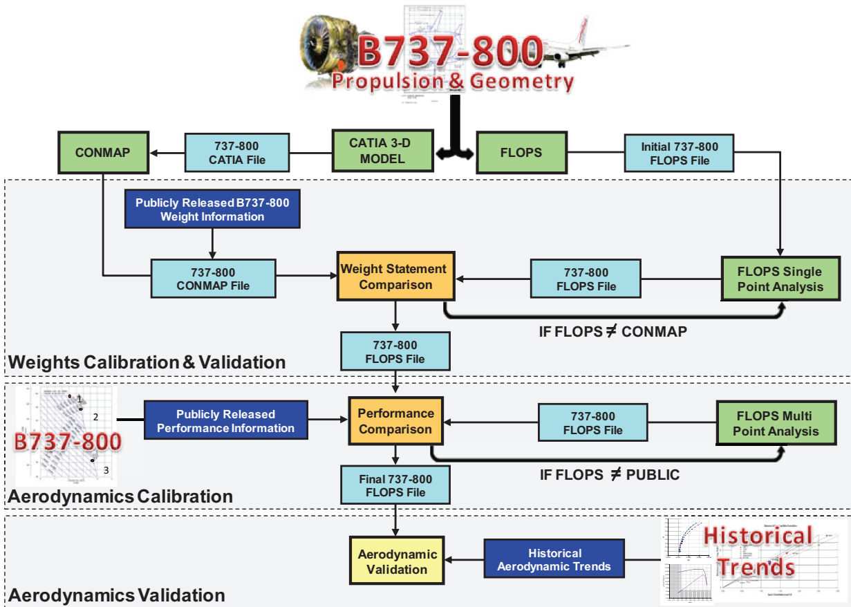
Figure 3-1. FLOPS Calibration Process With the 737-800
