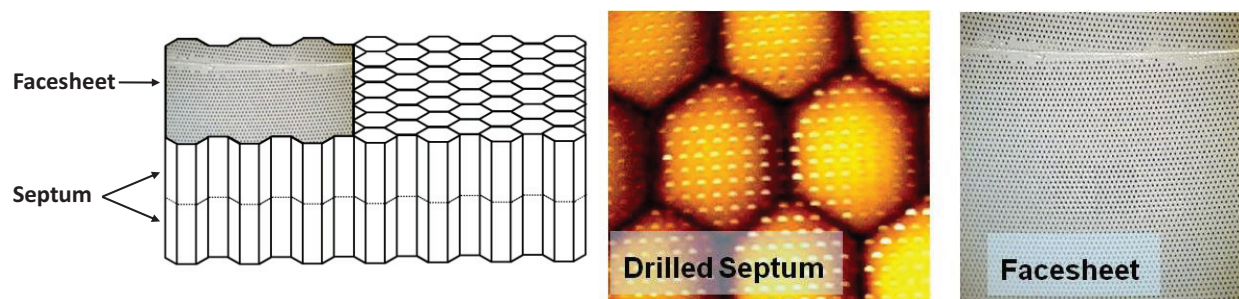
Figure 3-6. Acoustic Liner Conceptual Design Examples
