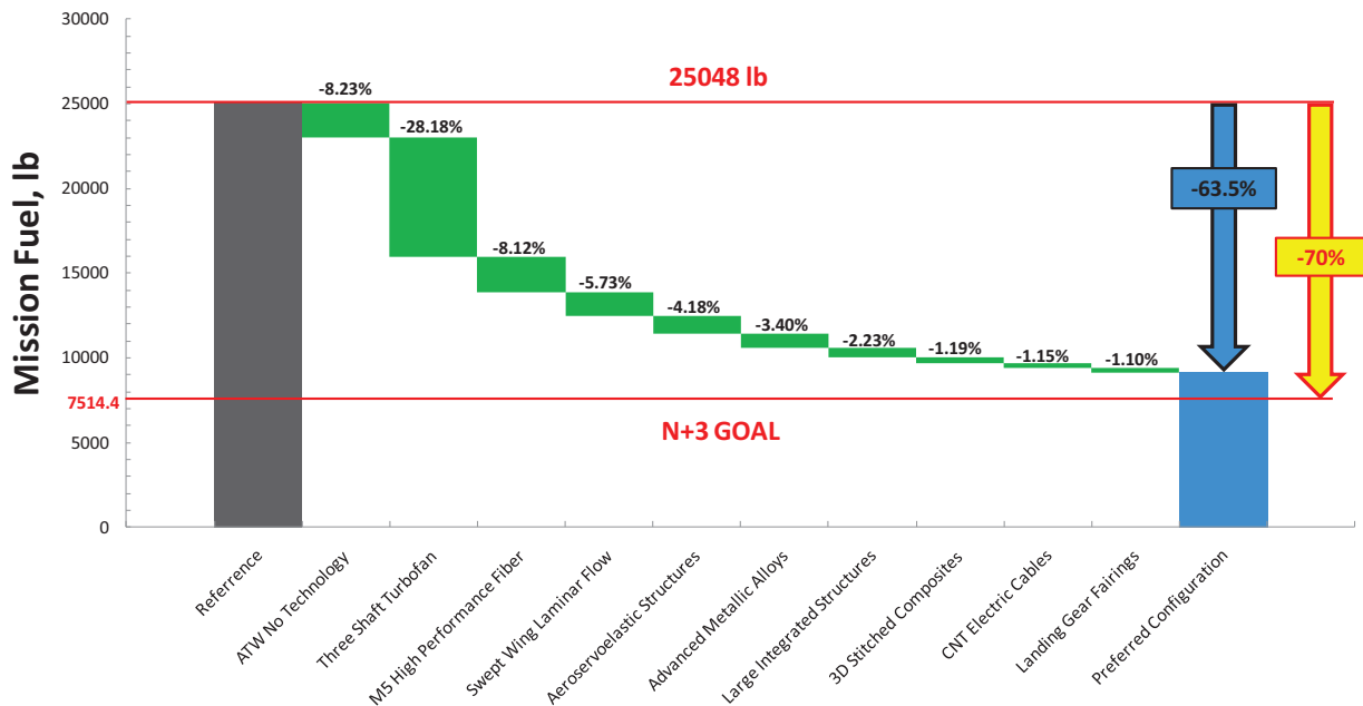
Figure 6-16. Preferred Configuration Planform and Technology Contributions to Mission Fuel Burn Reduction
