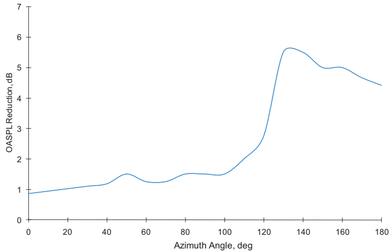
Figure 5-31. Inverted Flow Nozzle Noise Reduction
