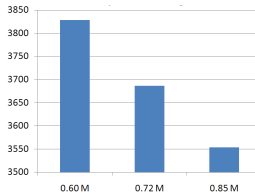
Figure 4-25. Effect of Varying Cruise Mach Number on Number of Airframes Required to Complete 8,000 Flights
