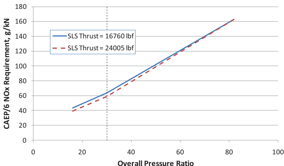
Figure 6-9. CAEP/6 LTO NOx Requirements.
