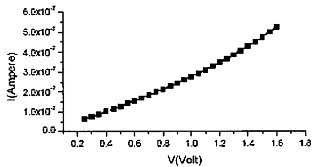
Figure 25: Bolometer IV characteristic
