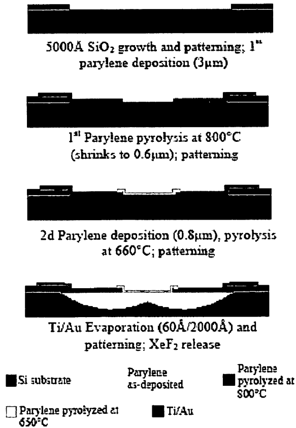
Figure 23: Process flow
