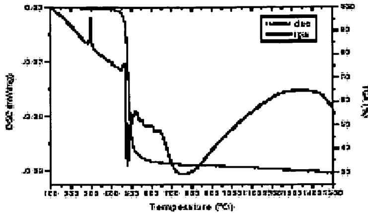
Figure 16: Simultaneous thermal analysis data for parylene C (heating rate = 5°C/min, in flowing Ar at 100mL/min)
