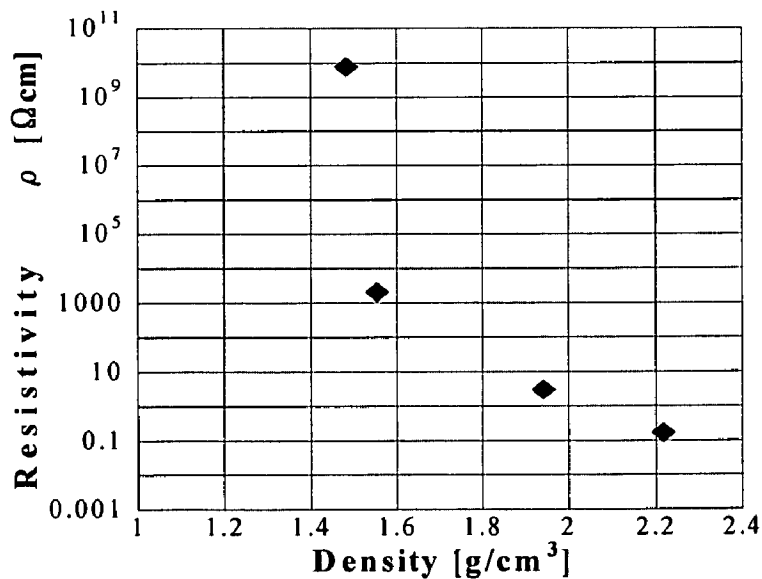
Figure 11: Resistivity vs. density.
