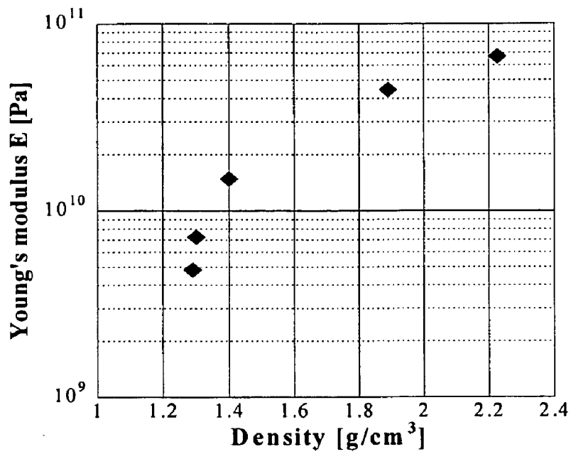
Figure 12: Young's modulus vs. density.
