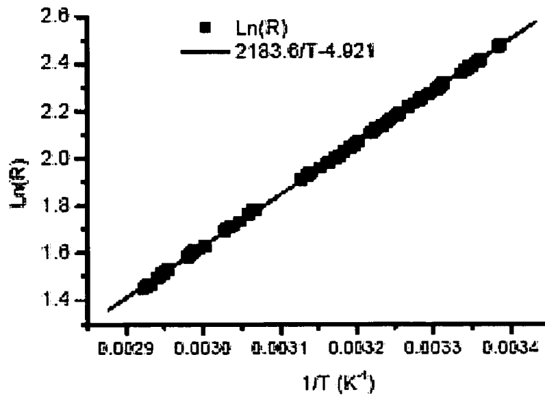
Figure 20: Resistance temperature dependence for pyrolyzed parylene
