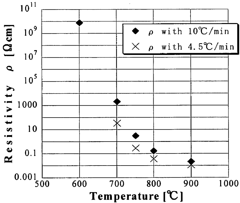
Figure 9: Resistivity of films vs. pyrolysis temperature.
