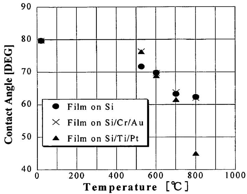
Figure 8: Contact angle according to pyrolysis temperature.
