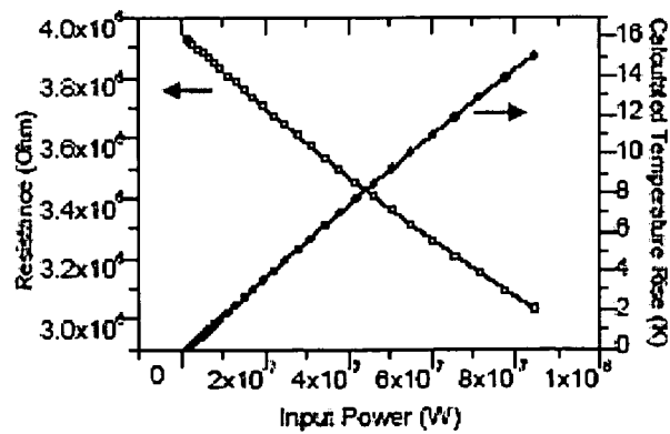
Figure 26: Pixel Resistance and temperature rise as a function of input power
