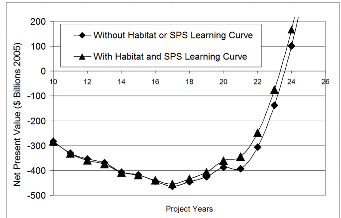
FIGURE 5. The effects of learning curves on the economics of 5 Man Year 384 person habitats (2005 costs and efficiencies)
