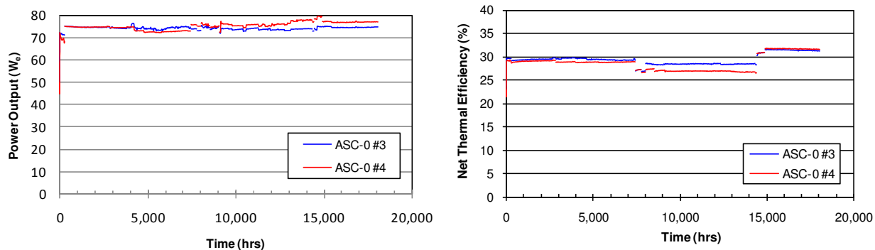
Figure 9. Power output and efficiency performance data from ASC-0 #3 and #4 through 18,600 hr of operation.
