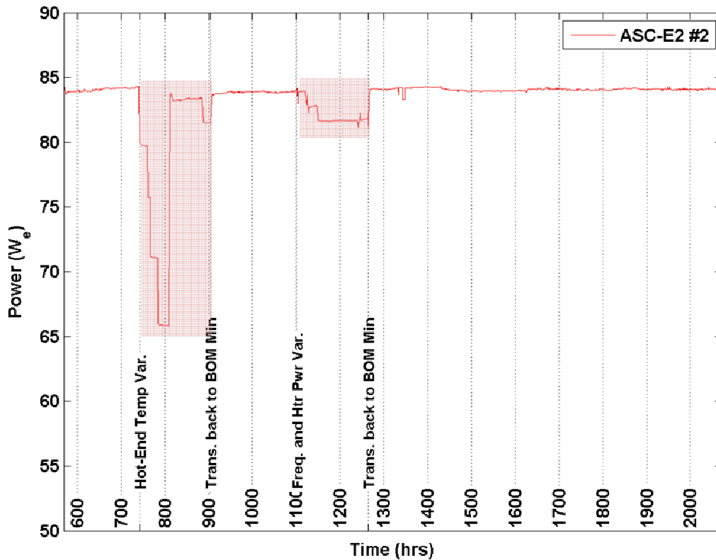
Figure 7. Power output performance data from ASC-E2 #2.
