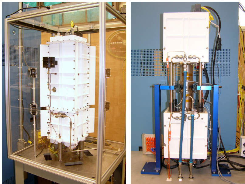
Figure 6. ASRG-EU containing ASC-E #2 and #3 (left) and ASC-E #1 and #4 (right).
