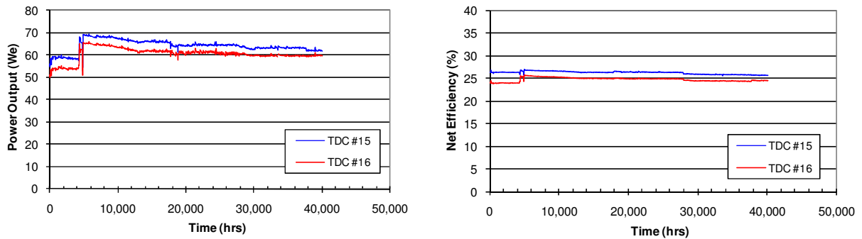
Figure 11. Power output and efficiency performance data from TDC #15 and #16 through 40,000 hr of operation.
