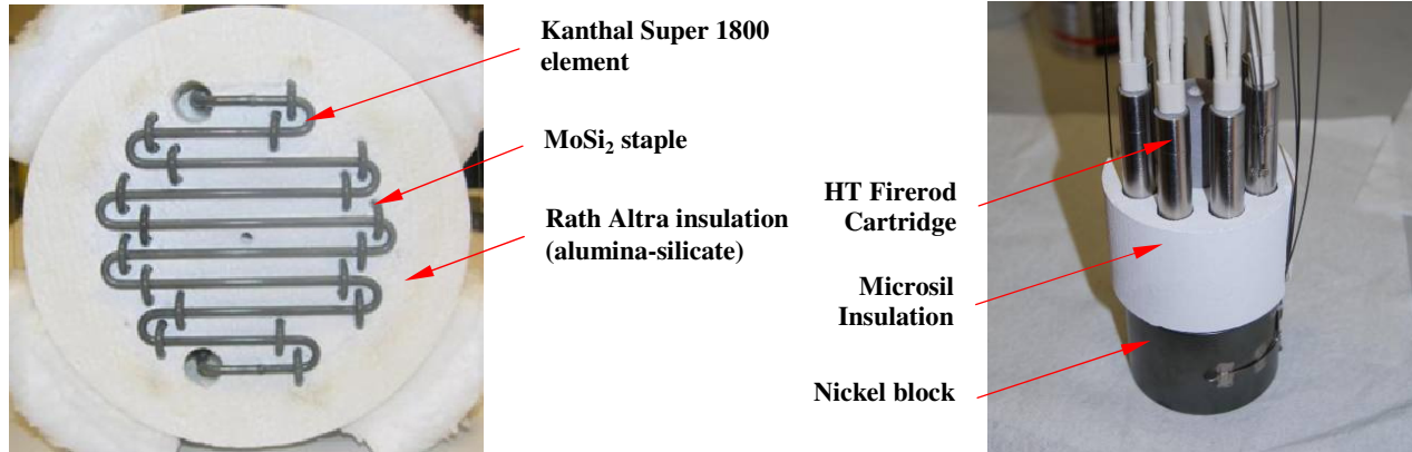
Figure 1. Kanthal Superthal 1800 heating element assembly (left) and Firerod Cartridge Heater (right). The serpentine-shaped MoSi 2 element of the Kanthal Radiant heater is attached to the solid insulation with staples also made of MoSi 2 .
