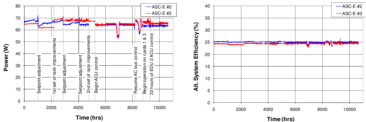
Figure 4. Power output and efficiency performance data from ASRG-EU (ASC-E #2 and #3) through 10,500 hr of operation.
