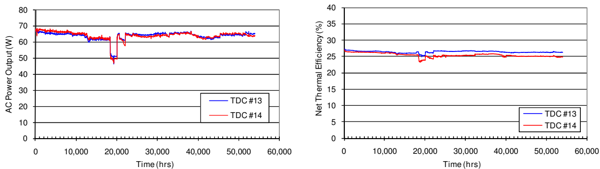
Figure 10. Power output and efficiency performance data from TDC #13 & #14 through 54,000 hr of operation.
