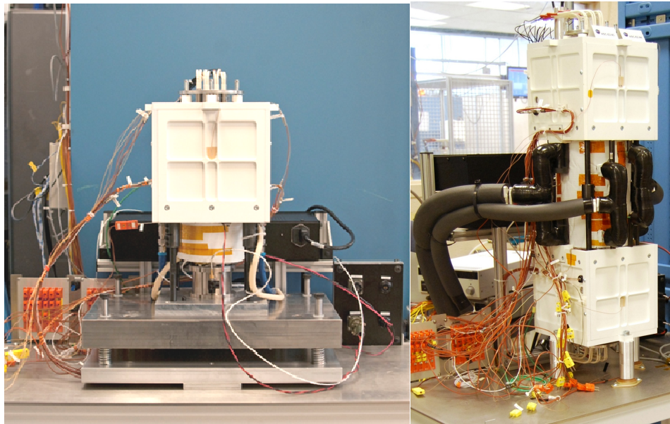
Figure 8. ASC-E2 #2 (left) and ASC-E2 #3 and #4 (right).
