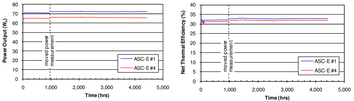
Figure 5. Power output and efficiency performance data from ASC-E #1 and #4 through 4300 hr of operation.
