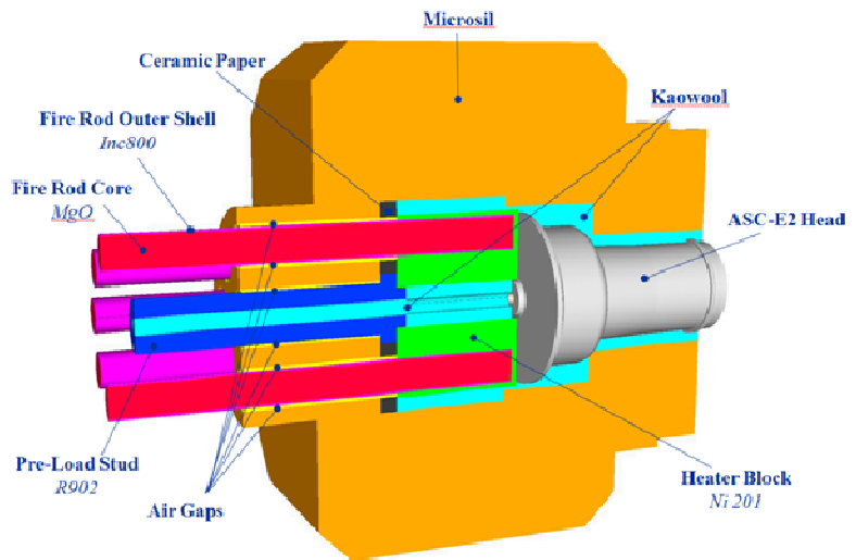
Figure 2. ASC-E2 Microporous insulation package.
