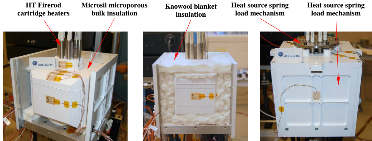
Figure 3. Insulation package for ASC-E2 testing. ASC-E2 #4 shown.
