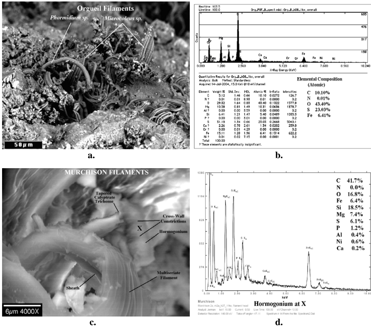
Figure 4. Filamentous microfossils in carbonaceous meteorites. a. FESEM image of mat of uniseriate (cf. Phormidium sp.) and multiseriata (cf. Microcoleus sp.) filaments in Orgueil CI1 meteorite with b. EDS data of overall field showing Nitrogen at trace levels; c. Murchison tapered uniseriate filament with calyptate apical cell and multiseriata filaments (cf. Microcoleus sp.) with delaminated sheath and hormogonium with cross-wall constrictions and d. elemental composition at spot X showing missing nitrogen.
