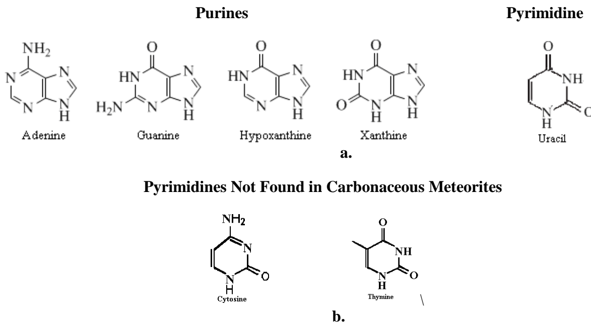
Figure 3. Life-critical nitrogen heterocyclic bases of nucleic acids include perinea and the pyrimidine a.) Present in carbonaceous meteorites and b.) missing RNA and DNA pyrimidines ( cytosine and thymine ) that have never been detected in meteorites.
