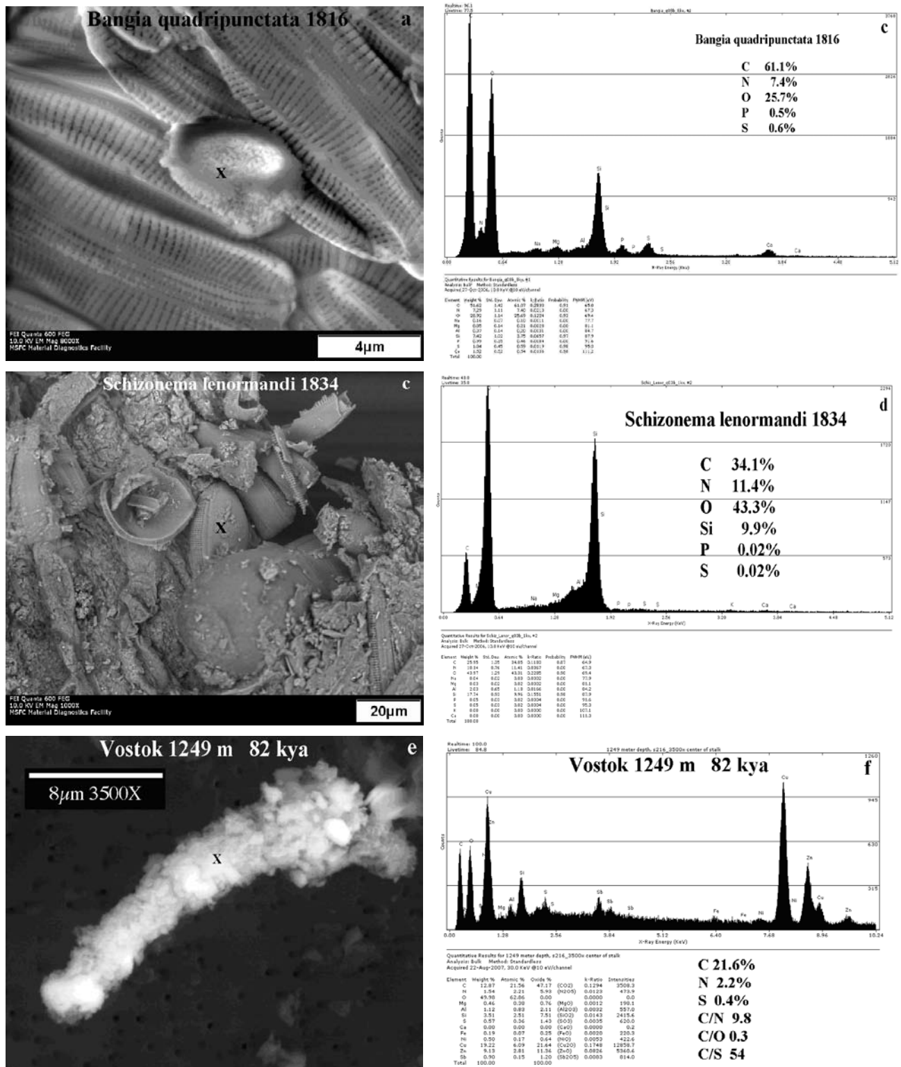
Figure 5. FESEM images of and EDS spectra taken at spots marked by the X for diatoms collected (a, b) in 1816 and (c, d) in 1834 and for a cyanobacterial filament ( Limnothrix sp.) from 82,000 year old ice from Vostok, Antarctica.
