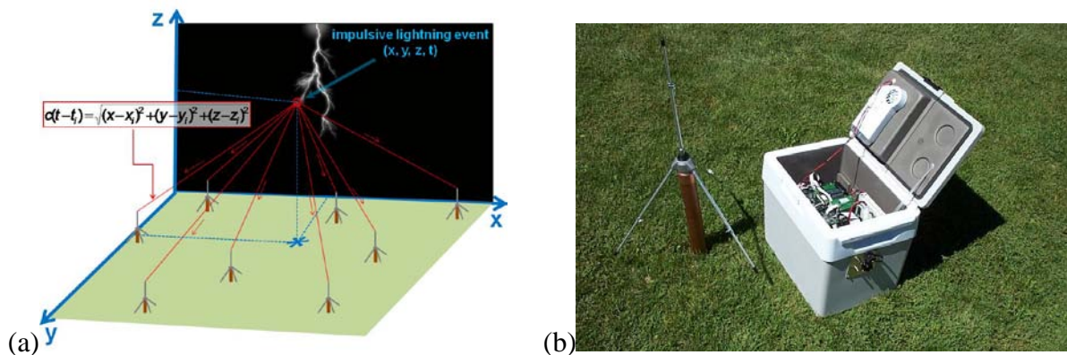
Figure 1 – (a) Illustration of the time-of-arrival technique used by the LMA system. The times ( t_i ) when a signal is detected at N \geq 4 stations are used to solve for the 3D source location ( \underline{x} , y , z , t ) of the impulsive breakdown processes associated with a discharge. (b) Portable LMA station electronic box and antenna.
