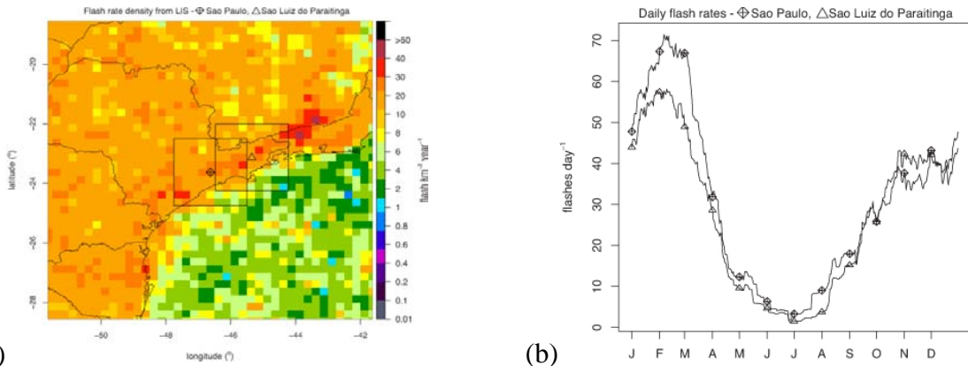
Figure 2 – (a) Lightning flash rate density ( \text{fl km}^{-2} \text{ yr}^{-1} ) for Southeast Brazil. (b) Daily flash rate (flashes per day) around São Paulo and São Luiz do Paraitinga (i.e., flash rate over black squares ( 2 \frac{1}{4}^\circ ) around these cities on item (a)). Lightning data is from LIS climatology from 1 January 1998 to 31 December 2008 in \frac{1}{4}^\circ of resolution.
