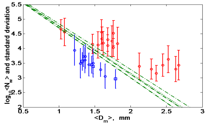
Fig. 1: The average value of \log_{10}(N_w) with \pm 1\sigma (standard deviation) bars versus D_m (mm) from discrometer (open circles) and as retrieved from dual-polarization radar (open squares) for various rain climatologies. The green lines represent the separation equation determined independently from the Darwin observations, for \mu values of 2, 0, 3 and 5, where \mu is used to convert from D_0 to D_m .
