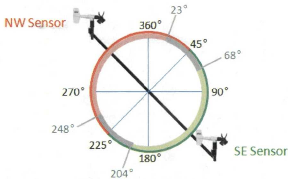
Figure 6. Dual sensor configuration on Towers 0002, 0006 and 0110. Sensors are mounted on the northwest and southeast side of each tower. The northwest sensor is always selected when the winds are between 249° and 22° (light red arc) and the southeast sensor is always selected when the winds are between 69° and 203° (light green arc). Either sensor can be used in the two gray regions when the winds are between 23° and 68° or 204° and 248°.
