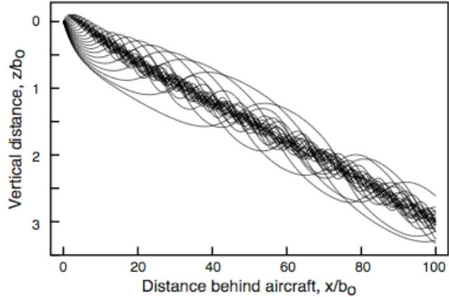
Fig. 3 Point-vortex representation of roll up of vortex sheet shed by span loading designed by R. T. Jones for minimum induced drag and wing root bending moment for a given lift and span [19].
