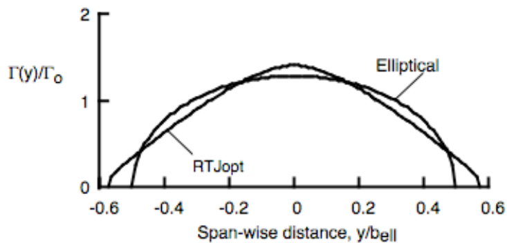
Fig. 2 Comparison of span loading used in present study as designed by R. T. Jones with elliptic span loading [17-19].
