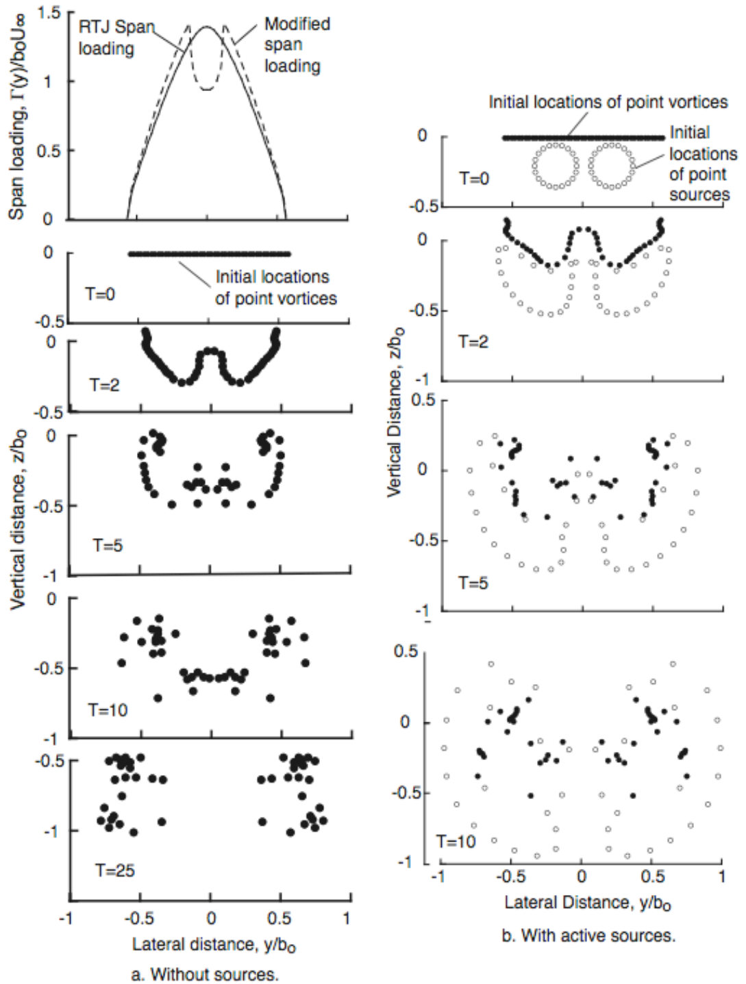
Fig. 4 End views of wake dynamics computed for cases when centerline value of lift carry over in fuselage-shrouded region is reduced by 40%. The computations indicate that the loss of lift near the centerline of the wing is not large enough to cause a segment of the vortex sheet to depart from the flow field in an upward direction.
