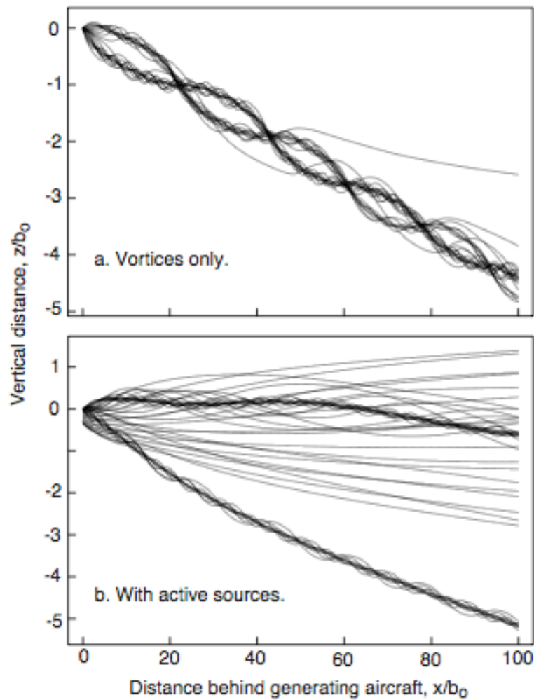
Fig. 9 Side view of two 40% enhanced-loading cases to help visualize wake behavior illustrated in Fig. 8.
