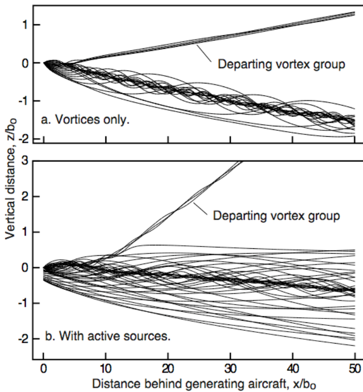
Fig.7 Side views of the two 70% reduced-loading cases presented in Fig. 6 to show overview of motion of departing vortex groups relative to wake dynamics of primary group of singularities.
