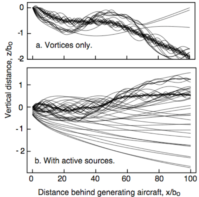
Fig. 5 Overview of wake dynamics in side view of the two cases shown in Fig. 4 (i.e., 40% reduction in centerline lift). Vortex pairs do not depart from main body of wake.
