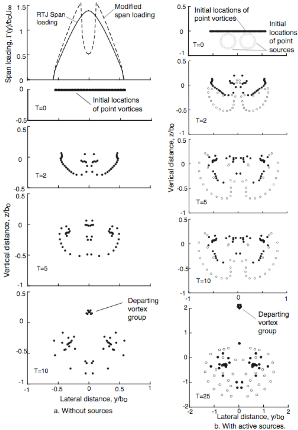
Fig. 6 End views of wake dynamics computed for cases when centerline lift in fuselage-shrouded region is reduced by 70%. These design considerations do cause a vortex pair to depart from the flow field of the bulk of the wake in an upwardly direction both with and without active sources in the flow field.
