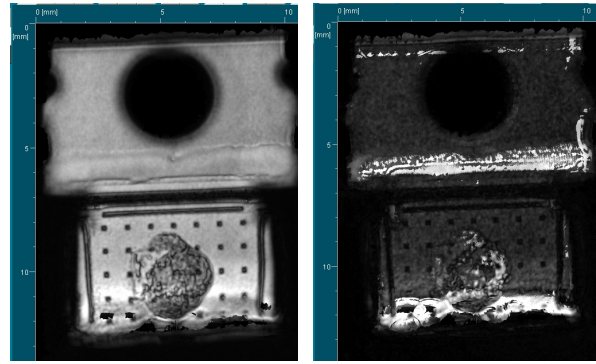
Figure 13. CSAM analysis of the power MOSFET.
