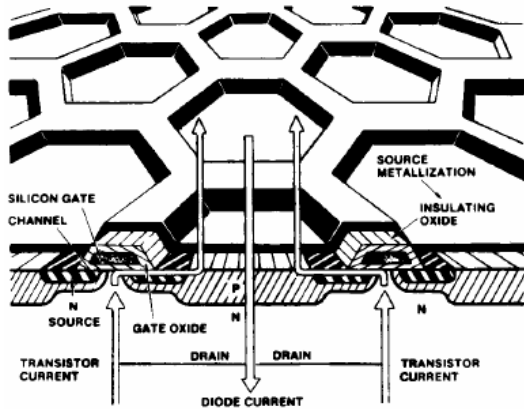
Figure 1. HEXFET power MOSFET structure from (Haran et al. 2007).
