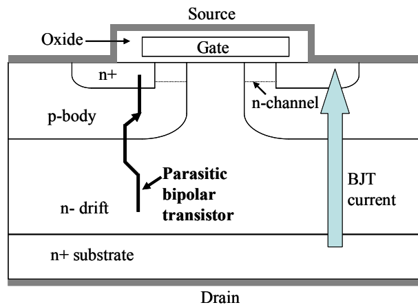
Figure 14. BJT activation leading to loss of gate control
