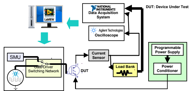
Figure 3. High-level schematic of experiment test bed for aging via thermal cycling.
