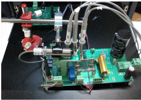
Figure 4. Test board for experiments with thermal cycling.
