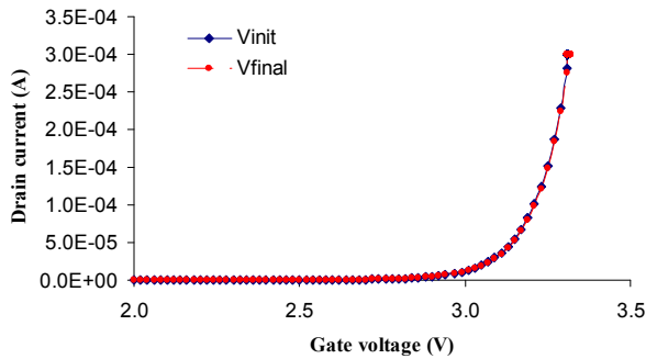
Figure 11. Threshold voltage comparison between first and third aging cycle.
