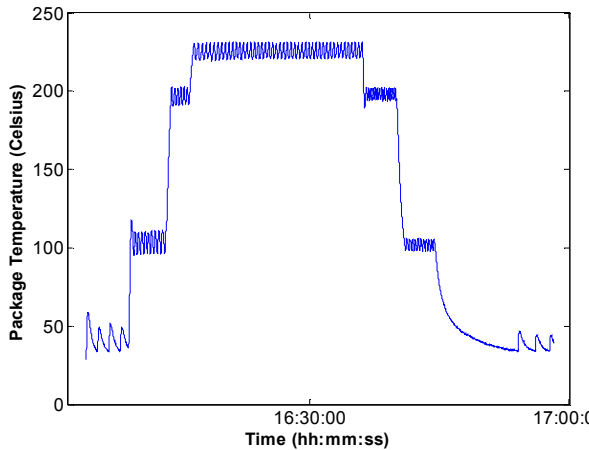
Figure 8. Stepped load temperature profile.
