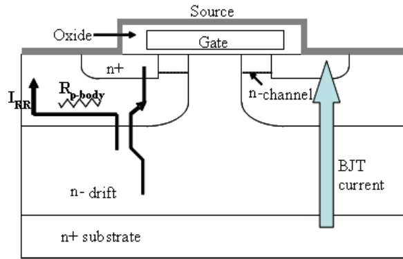
Figure 2. BJT activation due to diode reverse recovery current.
