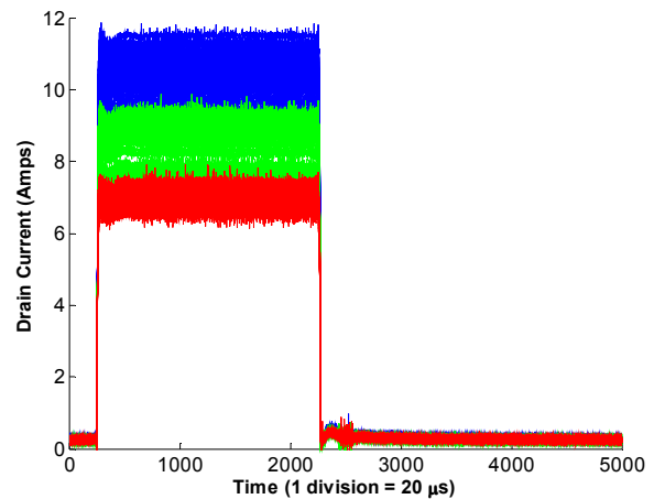
Figure 10. Drain current at failure.
