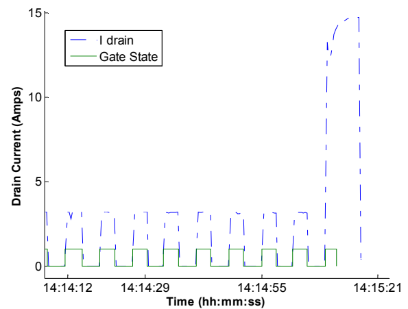
Figure 6. Latch-up failure of the power MOSFET.
