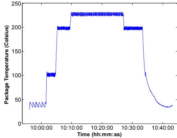
Figure 9. Temperature profile at failure.
