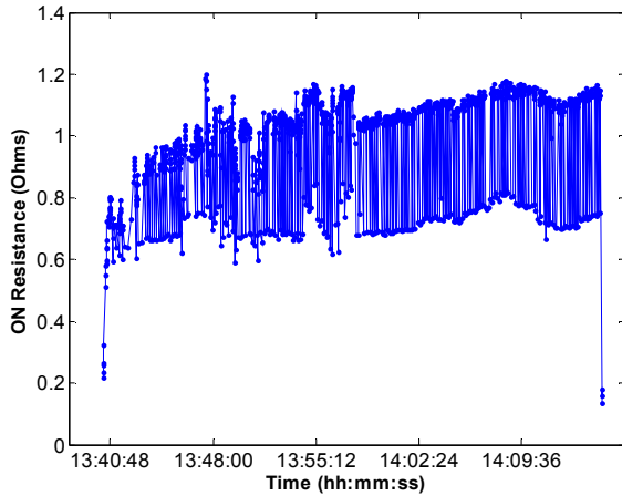
Figure 7. Power MOSFET resistance profile with time.
