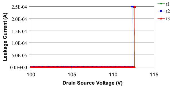
Figure 12. Breakdown voltage comparison for the three aging cycles.
