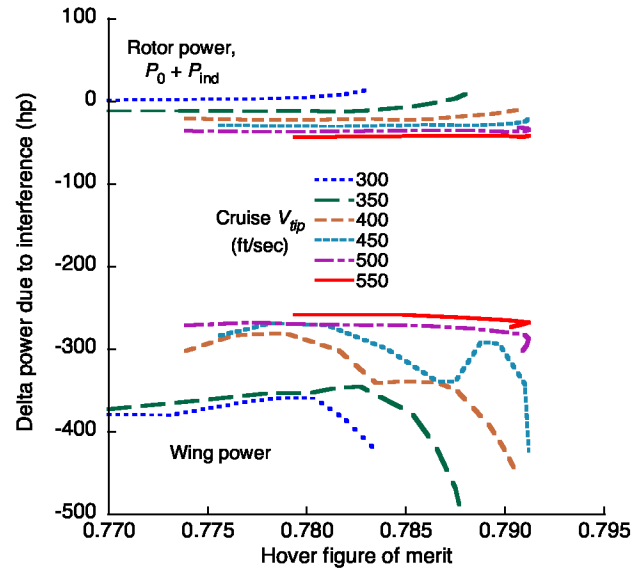
Fig. 6. Changes in wing and rotor power due to interference.
