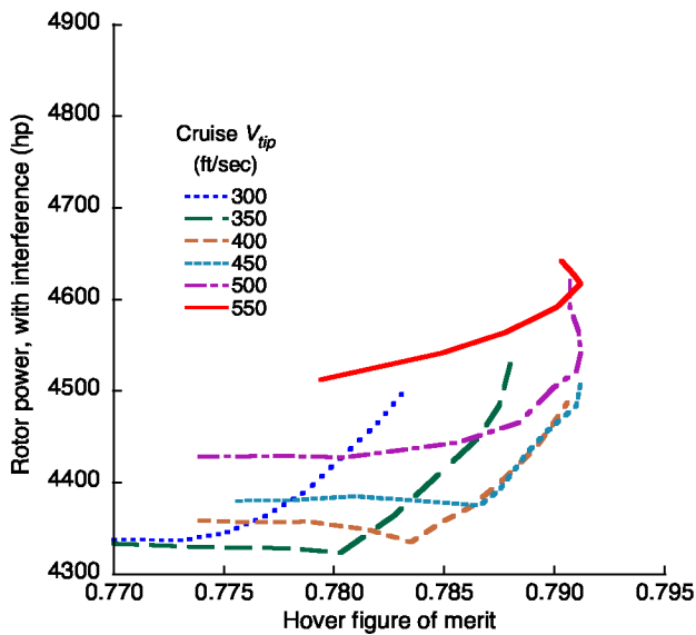
Fig. 5. Rotor power in cruise with wing/rotor interference.
