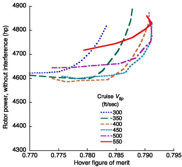
Fig. 4. Rotor power in cruise without wing/rotor interference.
