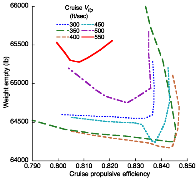
Fig. 10. Weight empty, with wing/rotor interference.
