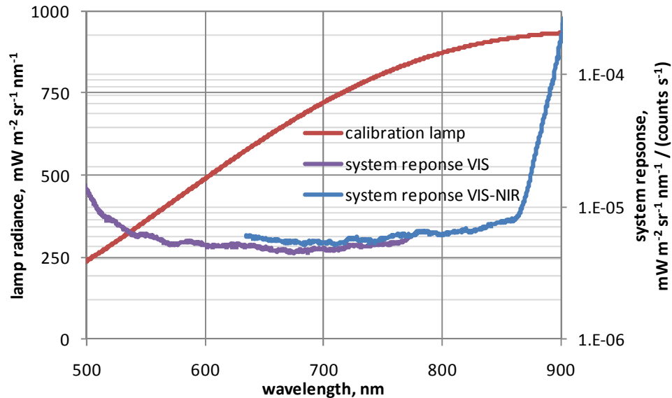
Figure 6. Calibration lamp radiance and system response for the two wavelength ranges with the calibration lamp positioned on the segment axis.
