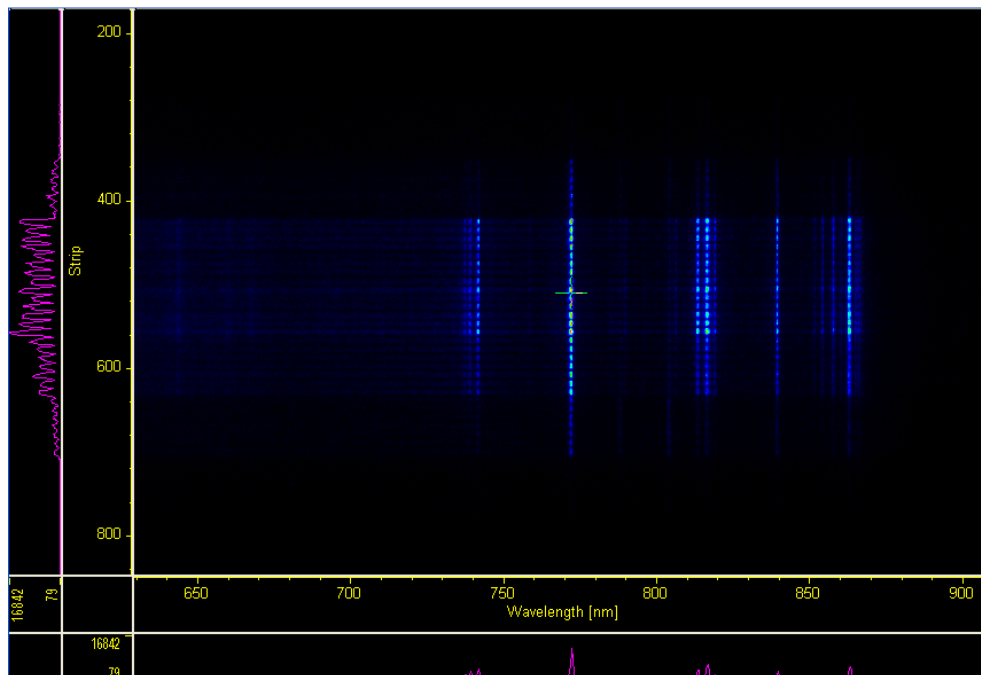
Figure 4. Raw data of a typical plasma showing the coupling of the fibers to spectrometer and CCD.
