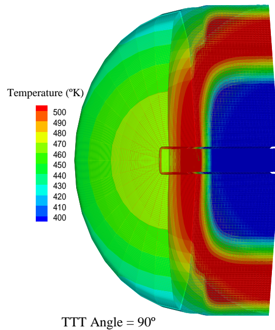
Figure 14d. Temperature contours at time = 400 s.
