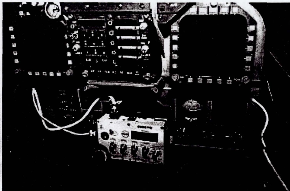
Figure 3. The SWUIS-A PIB installed in the rear cockpit of a NASA F/A-18B. Mounted just above the PIB is a Citizen LCD monitor used to verify camera pointing and to monitor image quality. The white cable connected to the top of the PIB carries camera power and control/video data. The cable connected to the left side of the PIB is routed to aircraft power and VTR connections on the right side of the cockpit.
