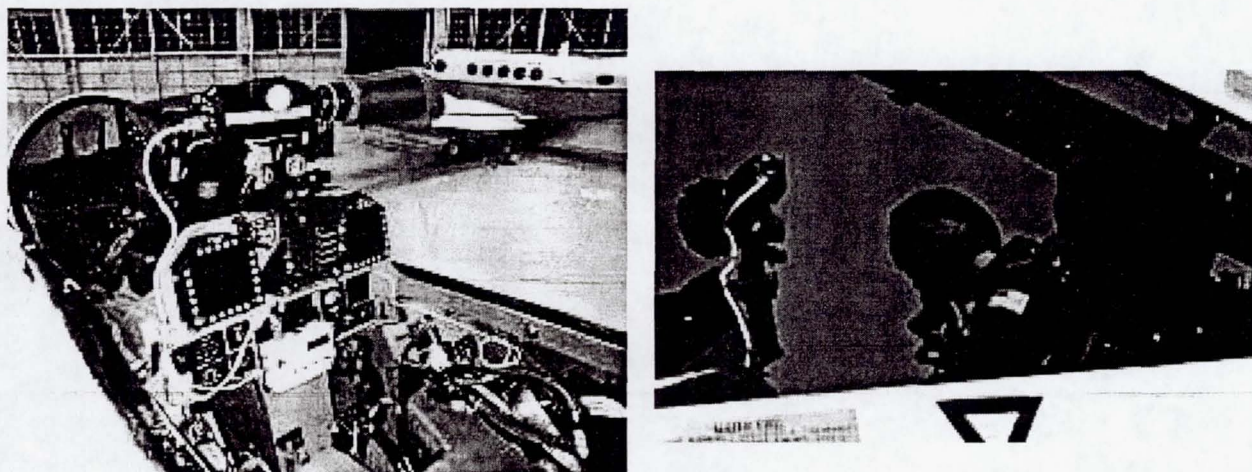
Figure 2. (Left) SWUIS-A flight hardware installed in the rear cockpit of a NASA F/A-18B. The SWUIS-A Xybion intensified CCD camera is mounted above the instrument glare shield on a Bogen bracket, allowing ALT/AZ pointing capability with image stability. The SWUIS-A camera control electronics and power interface box (PIB) is the white box mounted just forward of the stick, and is connected to the Xybion camera by the white cable harnesses. (Right) Author Durda preparing for takeoff to flight test the SWUIS-A system in a NASA F/A-18B (March 1999). The intensified CCD camera is visible with its light baffle installed on the foreoptic.
