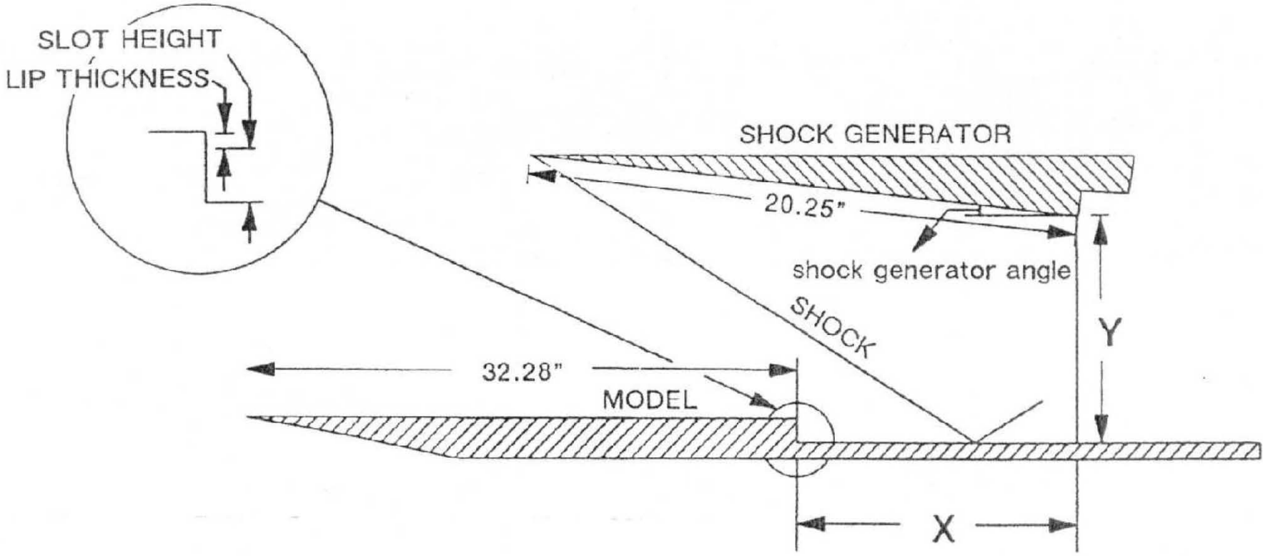
Figure 8 SHOCK GENERATOR DIAGRAM
