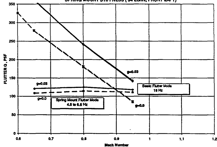
FIG 7.3.6 EFFECT OF MACH NUMBER AND MOUNT STIFFNESS ON FLUTTER (TCA AIRPLANE SCALED) SPRING MOUNTED MODEL)
