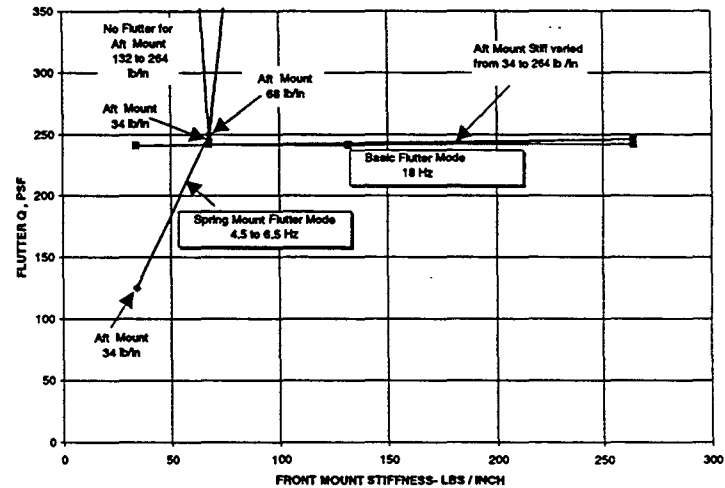
EFFECT OF MOUNT STIFFNESS ON FLUTTER TCA SCALED SPRING MOUNTED MODEL, M=0.80 , g=0.03 damping
