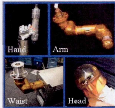
Figure 2. Robonaut Subsystems
