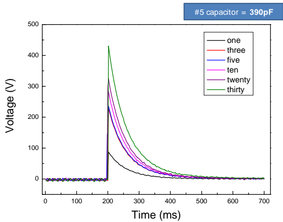
Figure 10. Charge collections by 390pF capacitor and gradual decays according to the exposure time of simulant to a 25kV and 0.391 mA e-beam flux.
