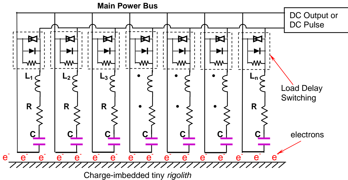
Figure 5. Equivalent Circuits for Differential Power Drain
