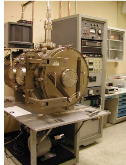
Figure 6. Experimental setup for electrostatic power generation from electro-statically charged lunar regolith simulant.
