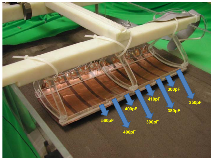
Figure 7. A home-made capacitor array was used for charge collection from simulant.
