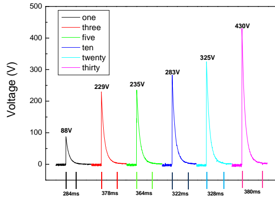
Figure 11. Charge collections and discharge decay diagrams of 390pF capacitor.
