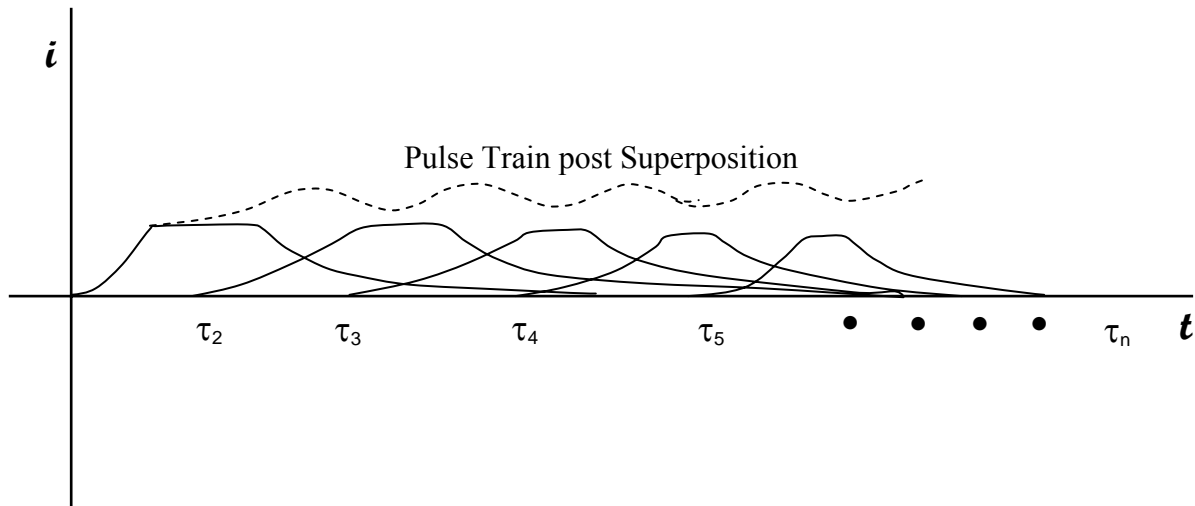
Figure 4. Example for pulse mode modulation of delay circuit.
