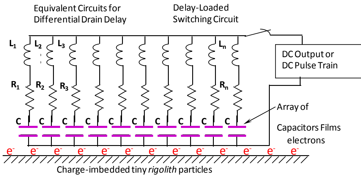
Figure 1. Equivalent circuit of power collection and conversion device from negatively charged Lunar soil.
