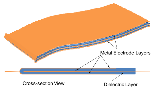
Figure 2. Electrodes and dielectric layers of a customized flexible capacitor strip.
