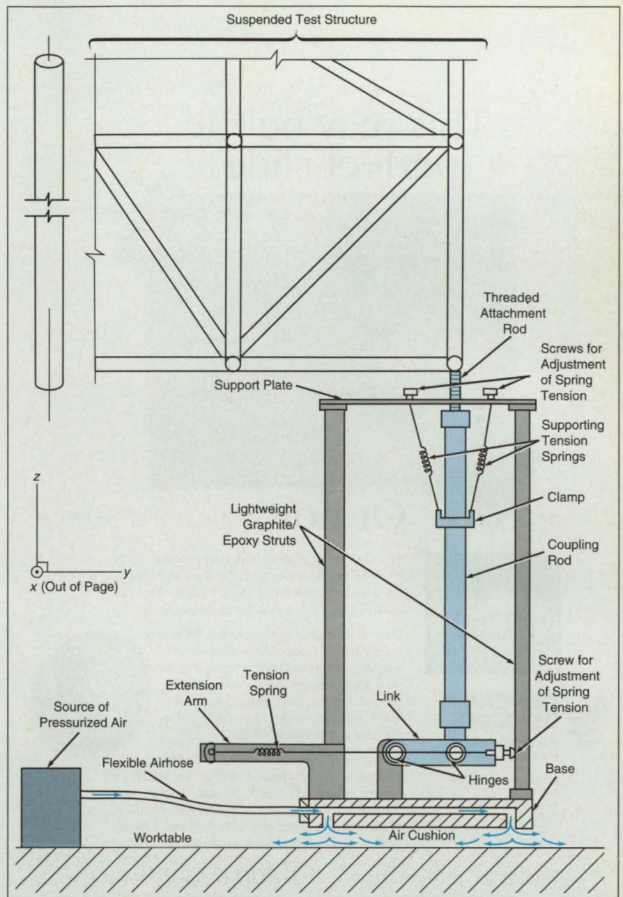
This Spring- and Air-Suspension Mechanism supports the weight of one end of the test structure, yet allows that end to move almost completely unhindered as though it were weightless and not attached to a suspension.
