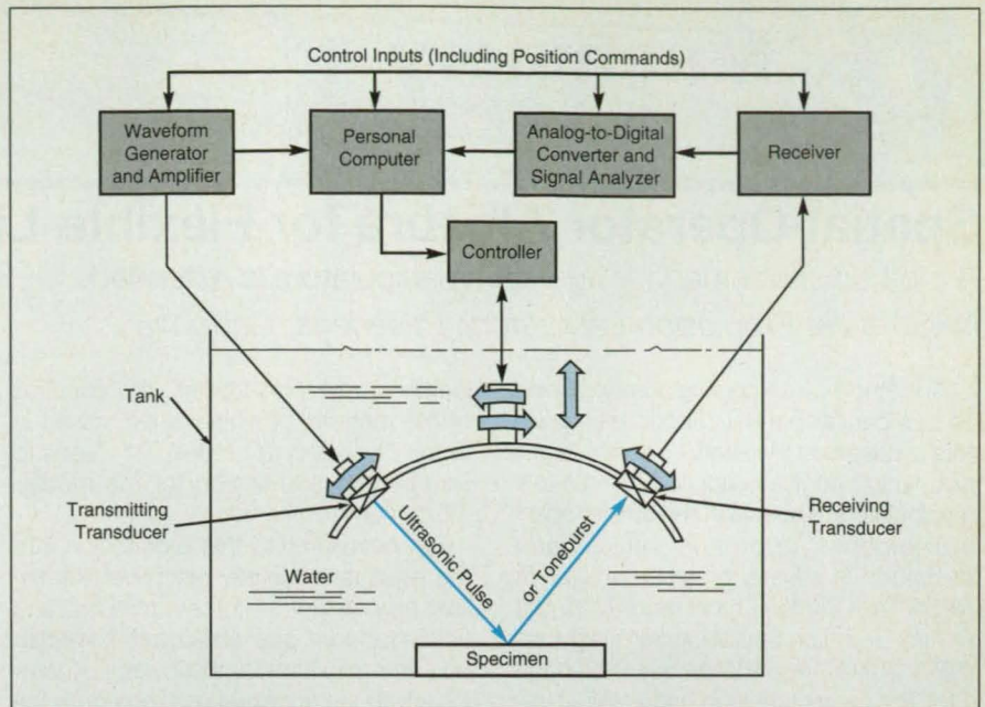
This Ultrasonic Testing System performs measurements that yield data on the five elastic constants of a specimen of orthotropic material.
