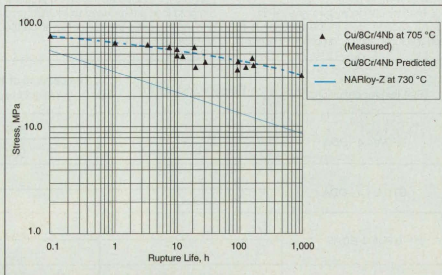
Figure 2. The Stress-Rupture Life of Cu/8Cr/4Nb exceeds that of NARloy-Z.
