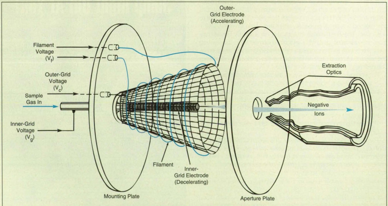
This Miniature Reversal Electron-Attachment Ionizer is equipped with a conical outer grid electrode and a cylindrical inner grid electrode. Alternatively, the outer electrode could be a cylindrical grid, and/or the inner electrode could be porous.
