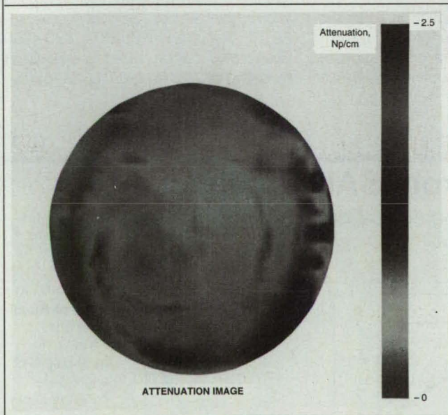
Figure 2. Precision Acoustic Scanning, combined with video and digital techniques, can yield video images like this one, which shows the cloudlike distribution of porosity inside a silicon carbide disk 4 cm in diameter.
