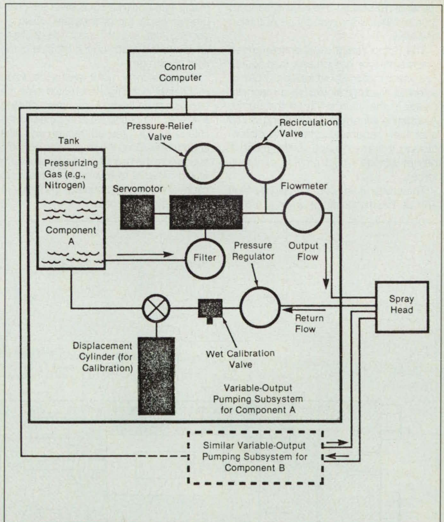
The Variable-Output Pumping System produces metered recirculating or nonrecirculating flows of two liquids (Component A and Component B) that are to be mixed in the spray head to make spray-on foam insulation.
