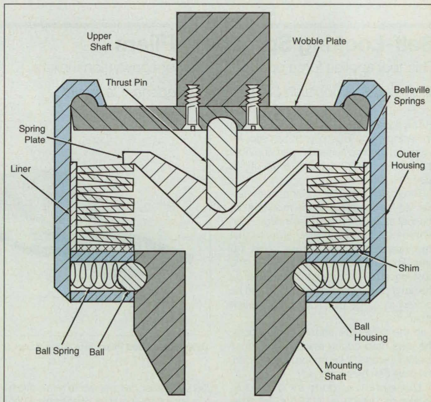
Torsion and Bending Loads between the upper and mounting shafts are relieved in the coupling by the ball springs and Belleville springs, respectively. Both sets of springs can be adjusted so as not to relieve loads below preset limits.
