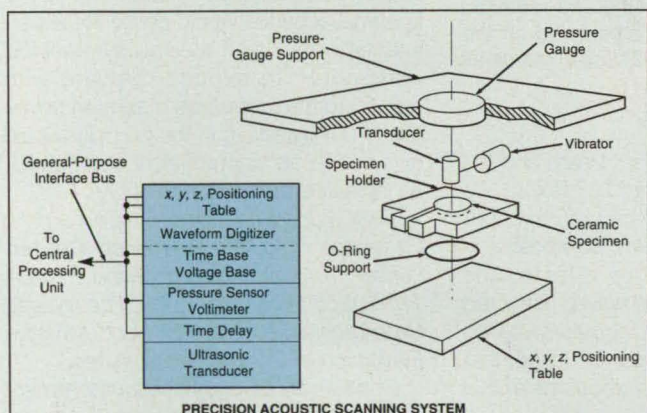
PRECISION ACOUSTIC SCANNING SYSTEM
