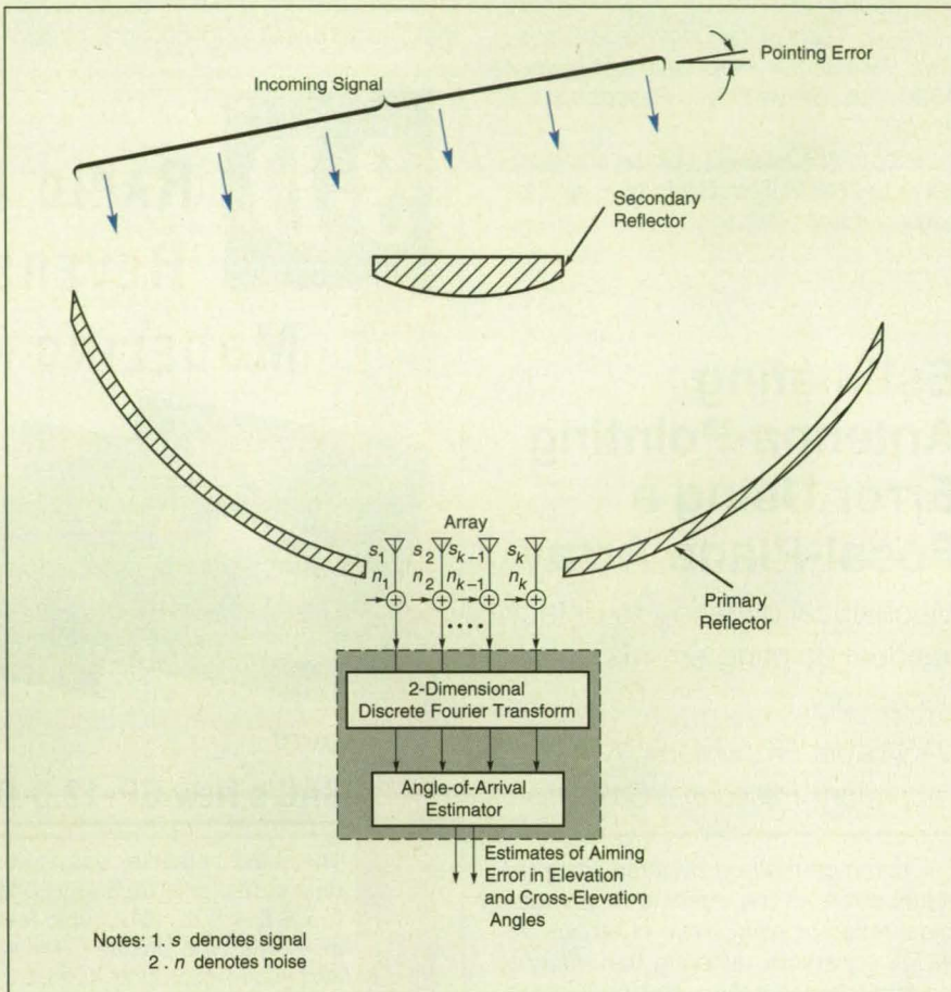
The Outputs of Multiple Receiving Feed Horns are processed to extract phase information indicative of the direction of arrival of a signal received from a distant source.
