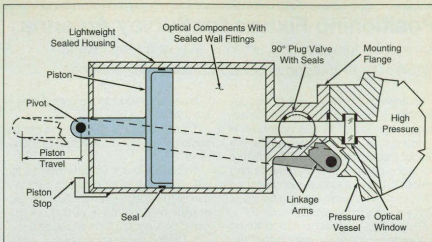
The Piston Slides to the Left as pressure builds in the housing. By the time the piston reaches the piston stop, it has turned the crank linkage and closed the plug valve. Parts of the pressure vessel and mounting flange are shown cut away to give a clearer view of the linkage arms.
