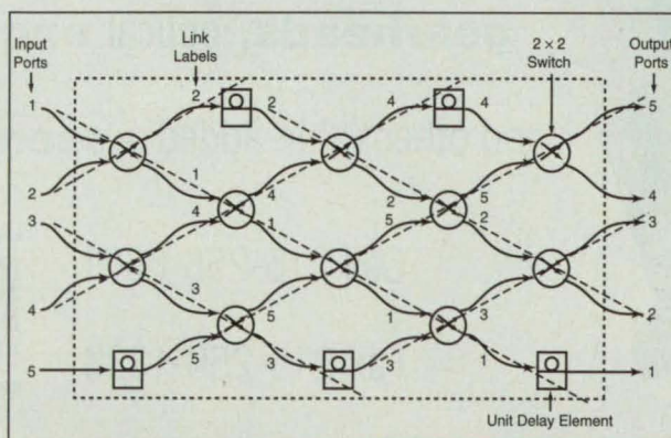
Figure 1. Each Packet Is Routed Up or Down in each column of this 5-input/5-output permutation engine. The routing algorithm ensures that each packet arrives at its designated output port without blocking any other packet that does not contend for the same output port.
