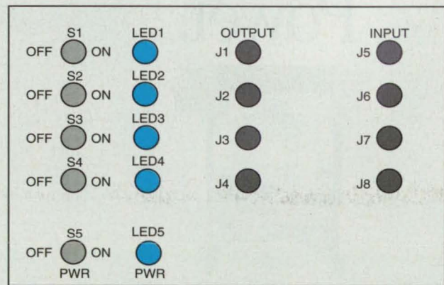
PANEL LAYOUT
