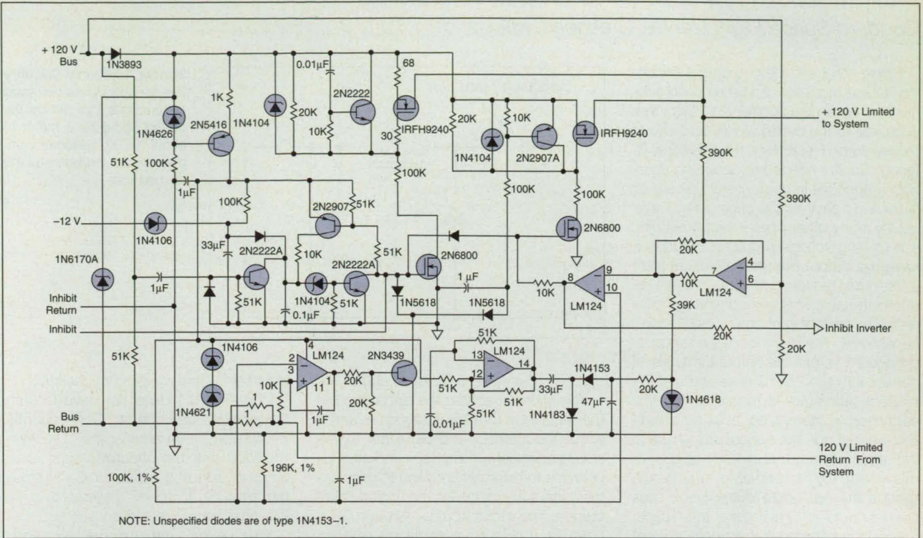
This Inrush-Current Limiter and Bus Isolator protects a power bus against excessive current demands imposed by a pulsed-current load.
