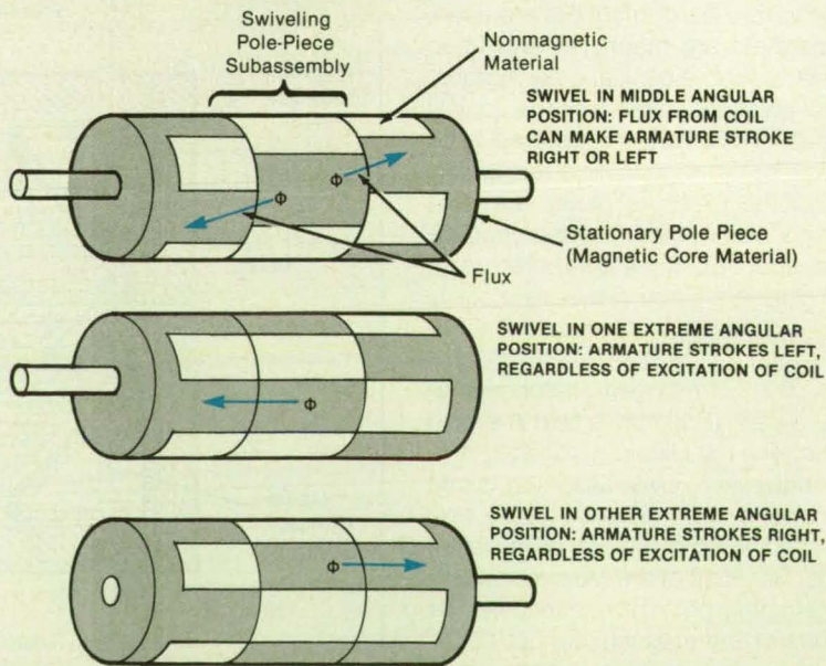
SIMPLIFIED VIEW SHOWING SWIVELING POLE-PIECE SUBASSEMBLY IN THREE SELECTABLE ANGULAR POSITIONS
