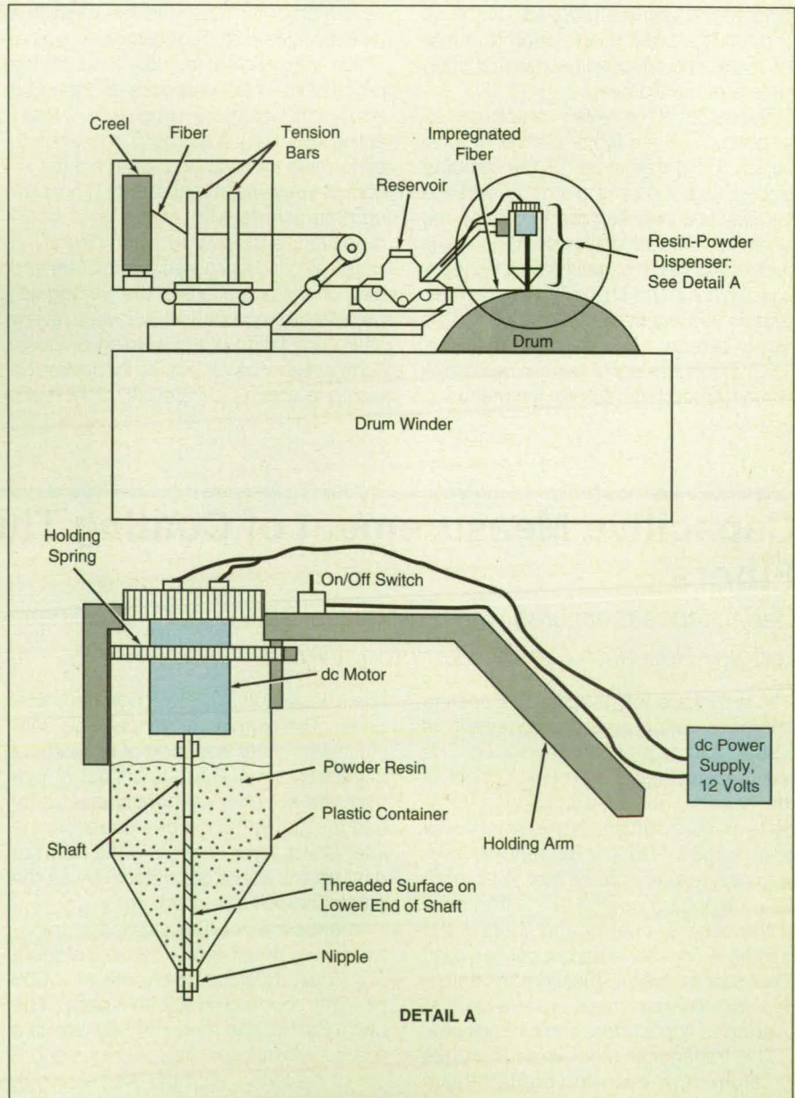
Resin Powder Is Metered through the opening in the nipple by a rotating threaded shaft.
