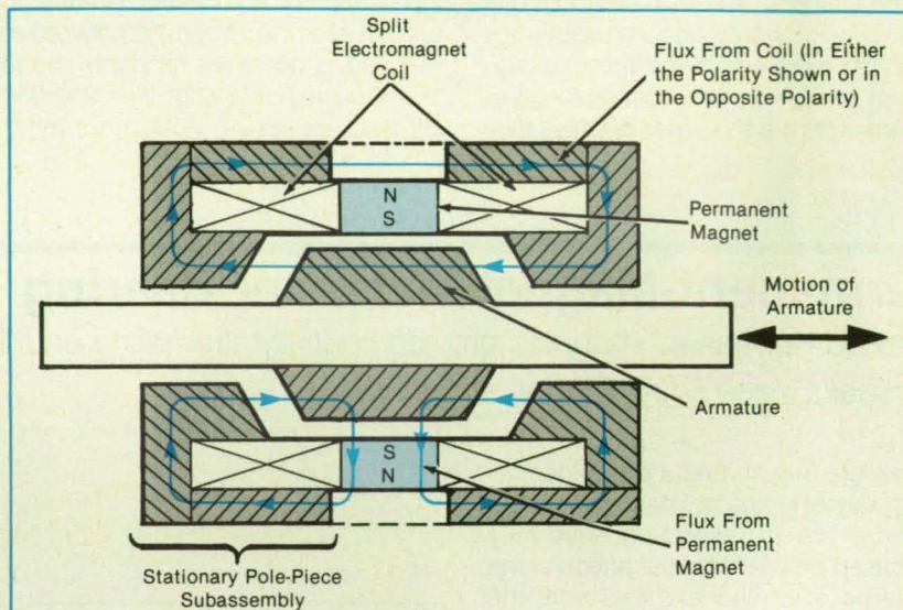
CROSS SECTION SHOWING FLUX PATHS
