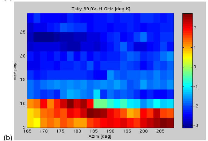
Figure 12.—NNMSR derived LWP (a), [ \text{gm}^{-2} ], 89 GHz V-H (b), [ ^{\circ}\text{K} ] at 22:28Z on September 21st.
