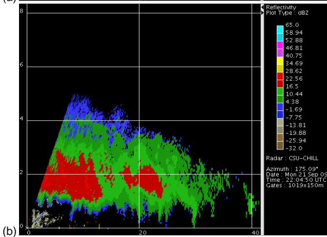
Figure 9.—CHILL RHI views from 175° azimuth of radial velocity (a), [ \text{ms}^{-1} ] and reflectivity (b), [dBZ] at 22:04Z on September 21st.
