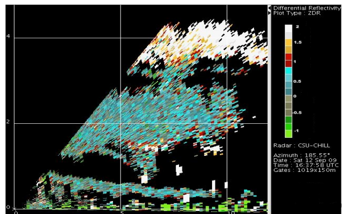
Figure 15.—CHILL RHI views from 185^\circ azimuth of differential reflectivity [dBZ] at 16:37Z on September 12th.
