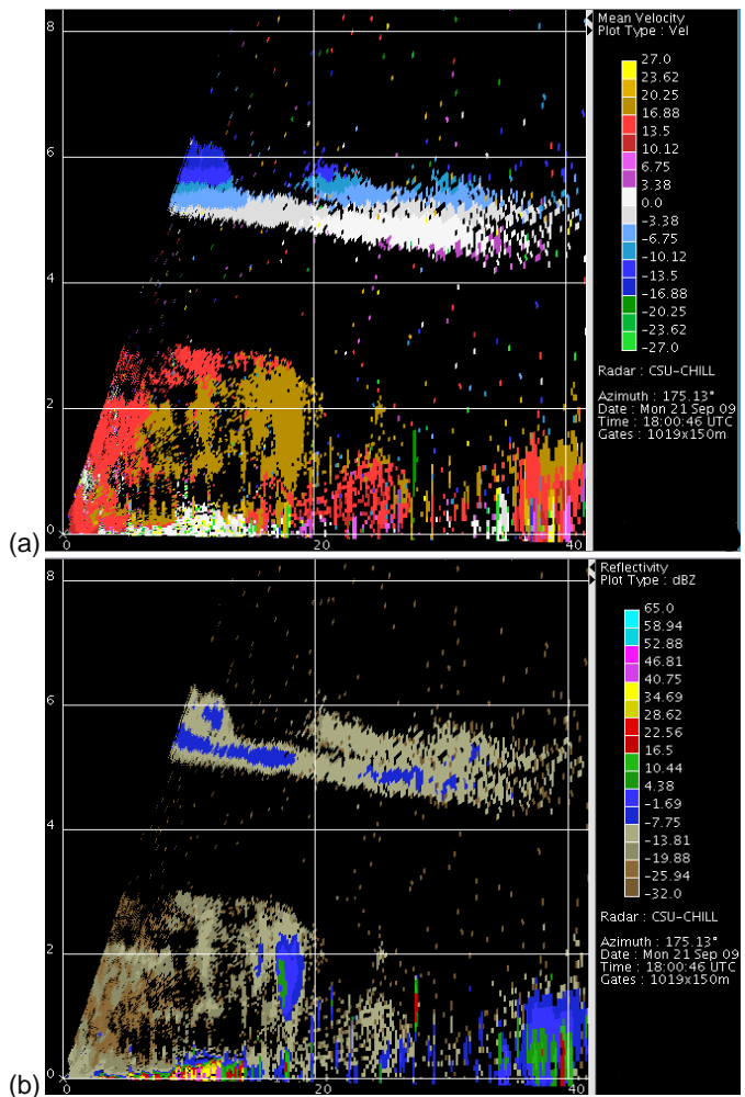
Figure 4.—CHILL RHI views from 175° azimuth of radial velocity (a), [ \text{ms}^{-1} ] and reflectivity (b), [dBZ] at 18:00Z on September 21st. Vertical and horizontal ranges are in kilometers.
