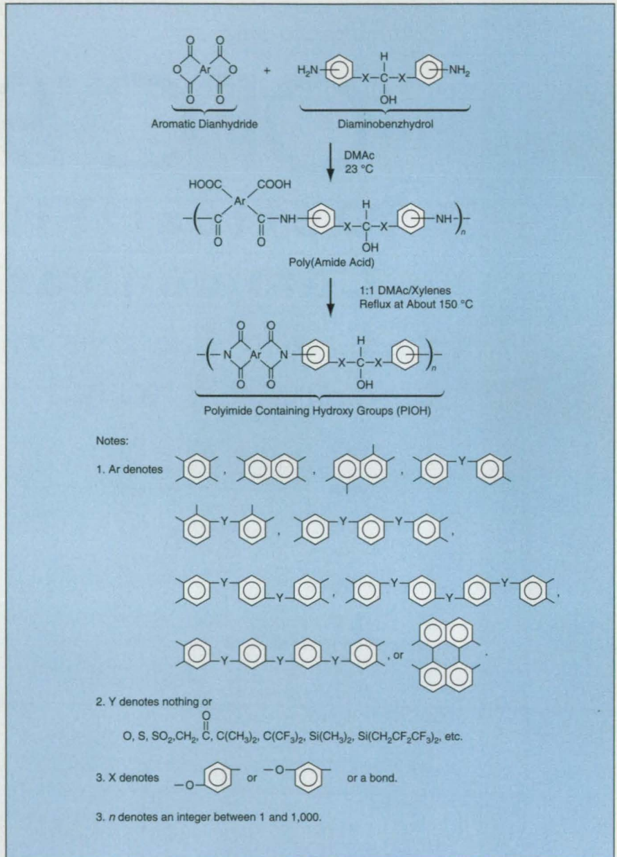
Figure 1. Polyimides Containing Hydroxy Groups (PIOH) are synthesized as soluble precursors to polyimides that will contain pendent siloxane groups.
