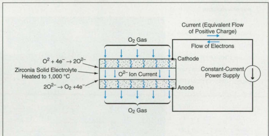
Oxygen Ions Would Be Transported through heated zirconia by the applied electric current. One oxygen molecule would be pumped through the zirconia membrane for every four electrons pushed around the circuit by the power supply.
