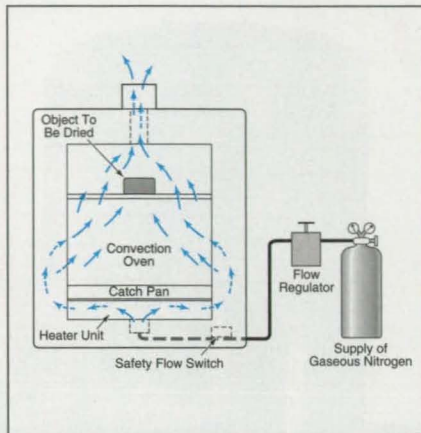
Nitrogen-Purge Equipment and safety interlocks are added to a convection oven to prevent explosive ignition of flammable solvent evaporating from the object to be dried.
