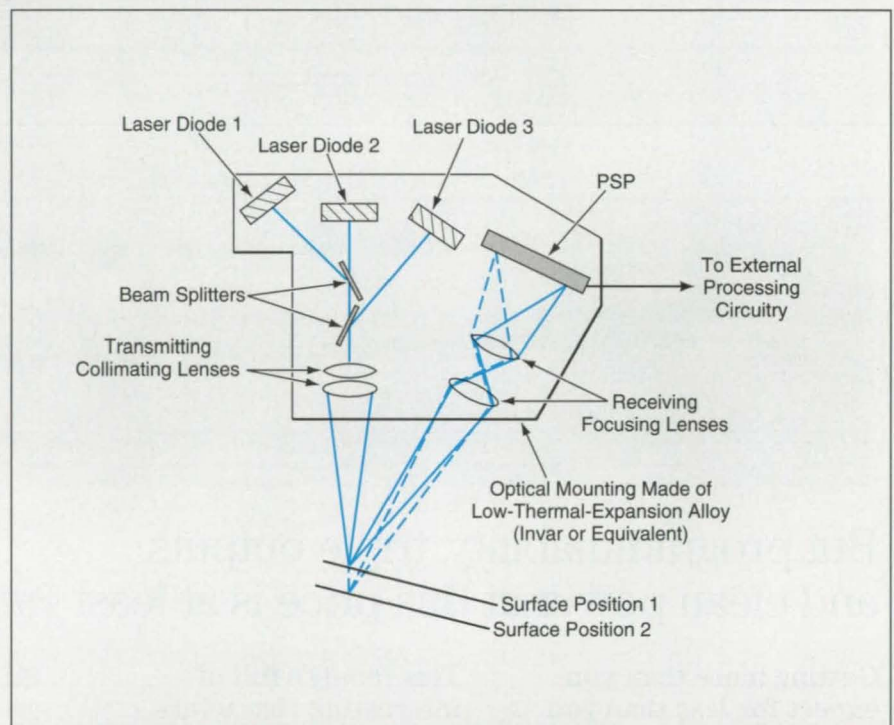
An Advanced Triangulation Sensor is typically 1/100 to 1/10 the size of triangulation sensors that have been used until now.
