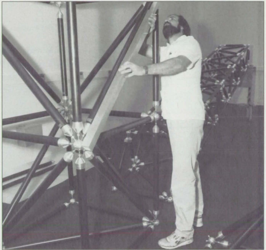
Figure 2. The Technician Holds the Reference Bar, which functions similarly to the reference plate shown in Figure 1.
