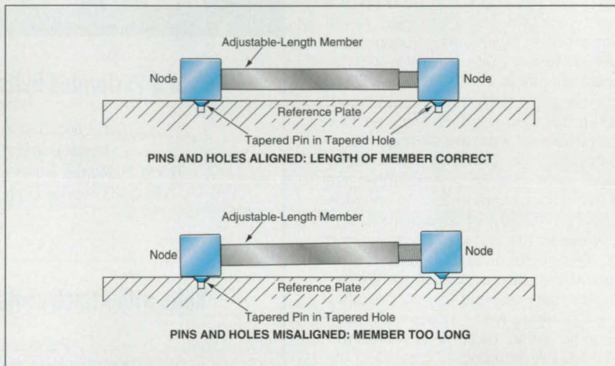
Figure 1. Misalignment Between One or More Pin(s) and Hole(s) is clearly visible as an indication that the length of the member deviates from the precise design value.
