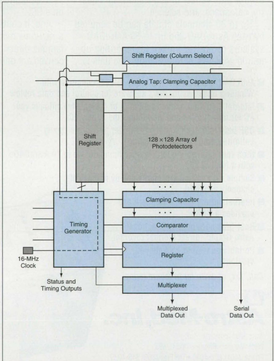
This Image-Sensing Integrated-Circuit Chip generates most of its internal control and timing signal from an externally supplied 16-MHz clock signal. The chip also produces chip-status and frame-timing signals. The short lines at the right and left sides of the figure indicate various control and bias connections.
