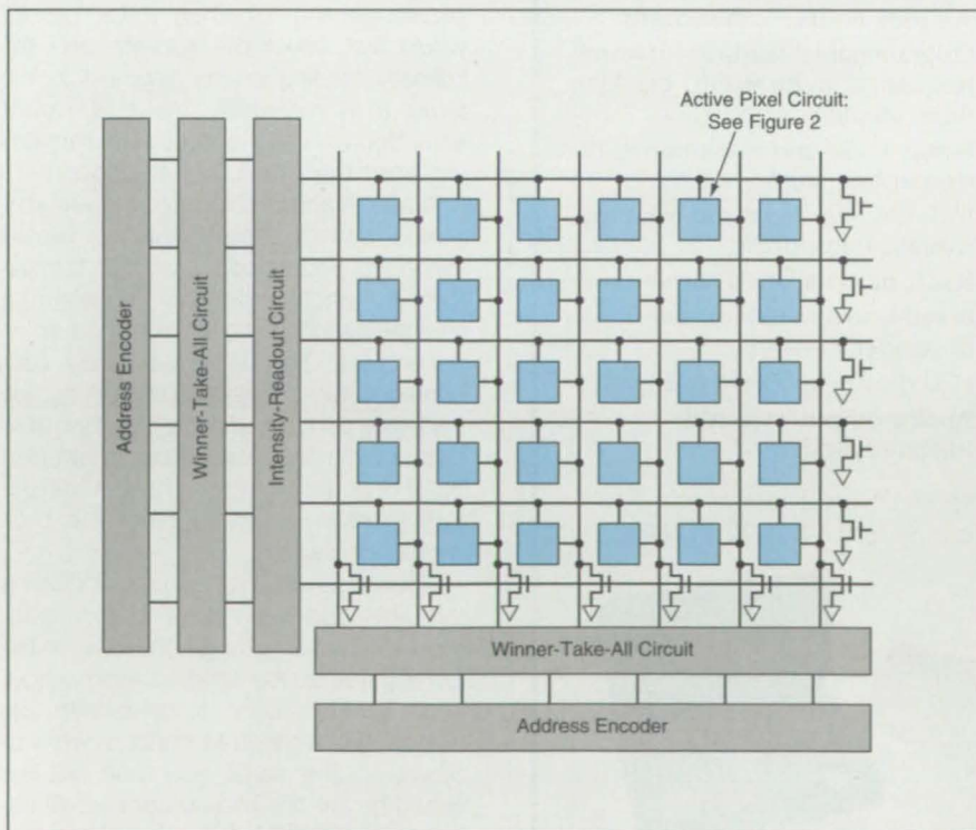
Figure 1. This CMOS Integrated-Circuit Image Sensor would provide readouts from pixels in order of decreasing intensity.
