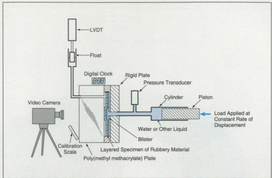
Growth of a Blister is tracked by a video camera, digital clock, pressure transducer, and a piston-displacement sensor. Cylinder pressure is controlled by a hydraulic actuator system. The linear variable-differential transformer (LVDT) and float provide a second, independent measure of change in blister volume that can be used as more precise volume feedback in a low-growth-rate test.
