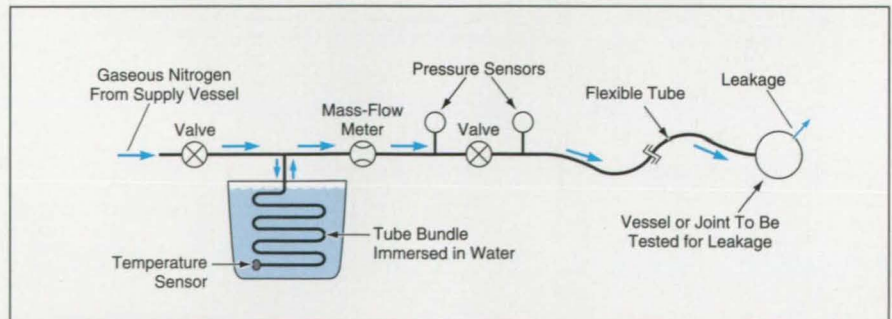
Nitrogen Is Supplied at Regulated Pressure to a sealed joint or vessel to be tested for leakage. Rate of flow indicated by the mass-flow meter serves as a measure of the size of the leak.
