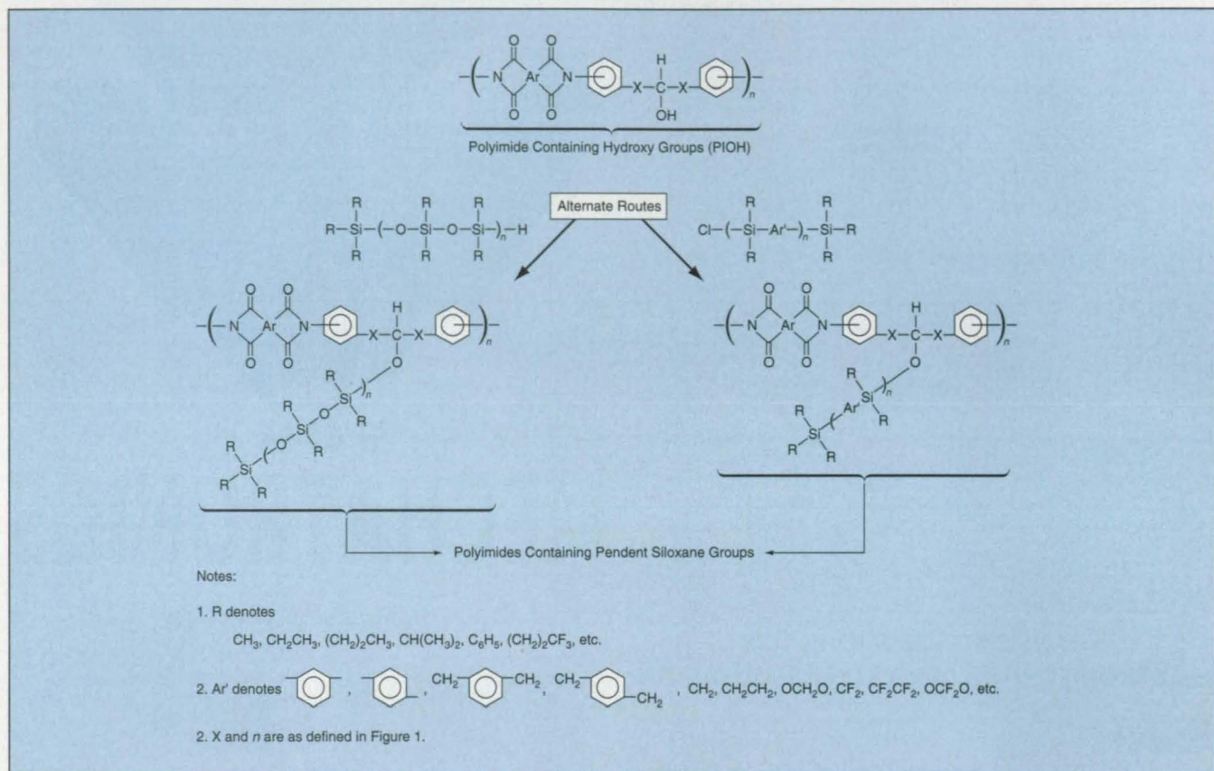
Figure 2. Pendent Siloxane Groups of two different types are incorporated according to two alternative approaches.
