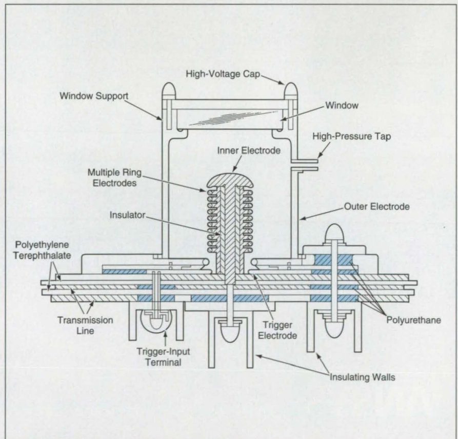
The Plasma Switch would feature an inverse-pinch configuration to prevent constriction of current sheets into filaments, plus a multiple-ring-electrode structure to resist high-voltage breakdown.
