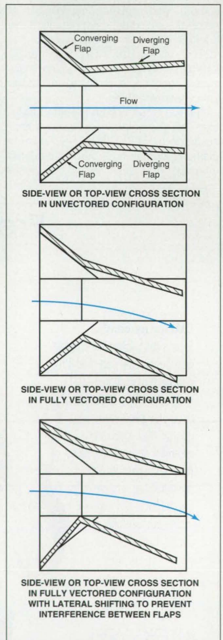
Figure 2. The Flaps Are Positioned and Oriented to control the direction of flow of the exhaust and thus the direction of thrust.
