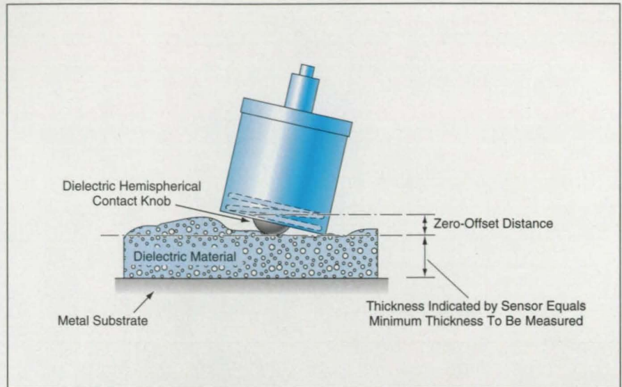
Figure 2. The Sensor Indicates the True Thickness when equipped with a hemispherical contact knob that ensures the correct zero-offset distance at the measurement location.
