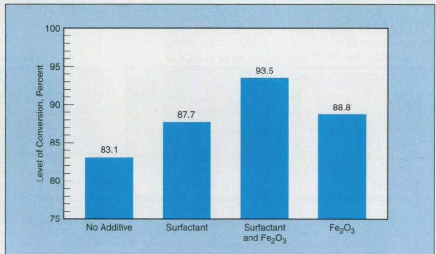
The Level of Conversion achieved by addition of both the surfactant and the catalyst is greater than that achieved by addition of either alone.
