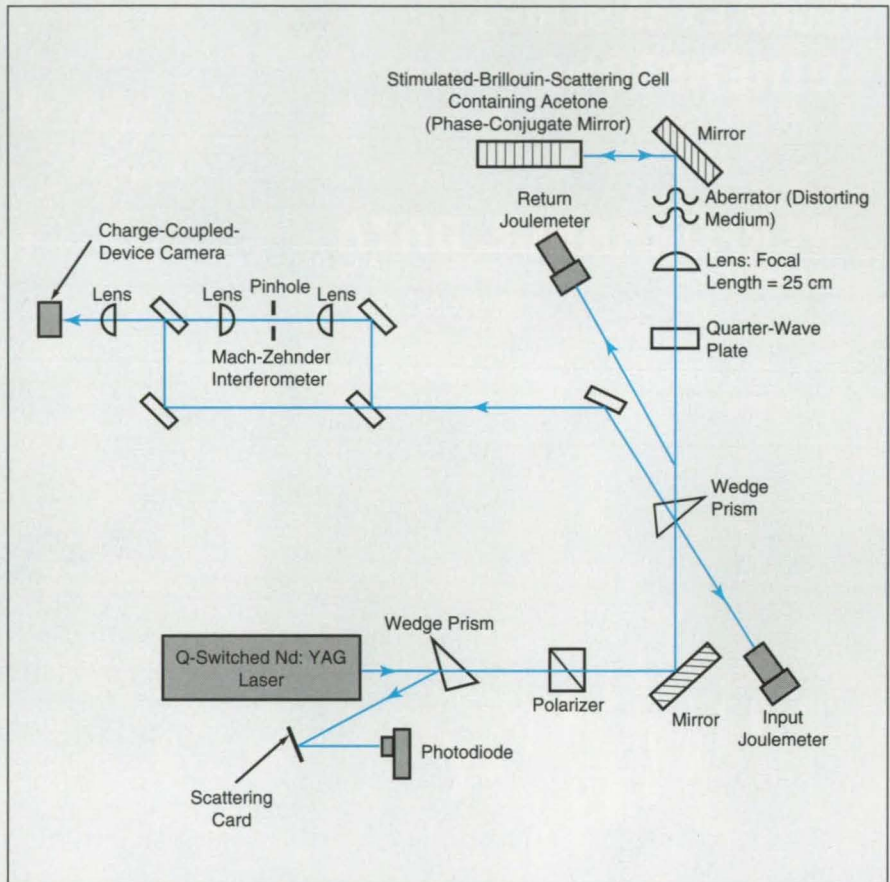
Figure 1. This Laboratory Setup can be used to demonstrate a phase-conjugate mirror.
