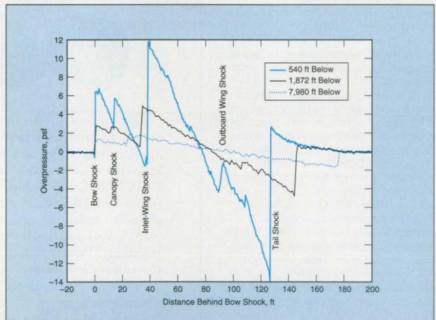
Figure 2. These Sonic-Boom Signatures are based on preliminary measurement data acquired by flying the F-16XL at several distances below the SR-71. The SR-71 was flying at mach 1.25 and an altitude of 31,000 ft (9.4 km).
