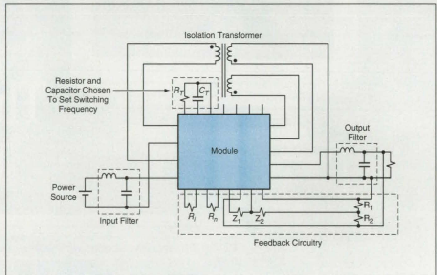
The Power Hybrid Module is a general-purpose power-switching module that provides flexibility in design and application. A complete dc-to-dc power converter can be constructed by adding the input/output filters and feedback circuitry to this module to suit the specific application.
