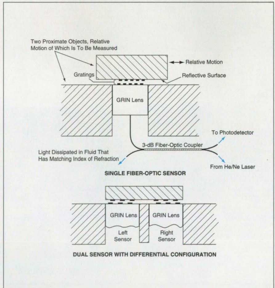
In this Fiber-Optic Differential Displacement Sensor, the differential configuration doubles (in comparison with a single sensor) the sensitivity to displacement and cancels the effect of a change in temperature.
