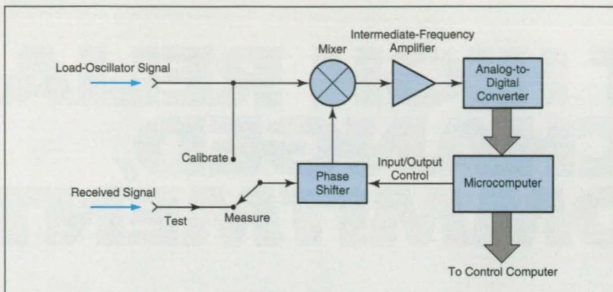
Figure 2. This Automatic Phase-Conjugation Submodule is a prototype of identical units that would be incorporated into the automatic amplitude-controlling and phase-shifting modules of Figure 1.
