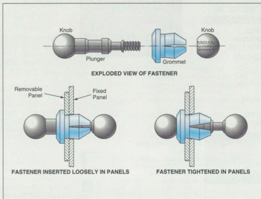
The Modified Fastener is tightened by pushing the left knob rightward and loosened by pushing the right knob leftward.
