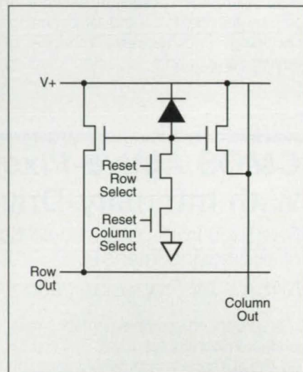
Figure 2. An Active-Pixel Circuit like this one would be located at the intersection of each row and column.
