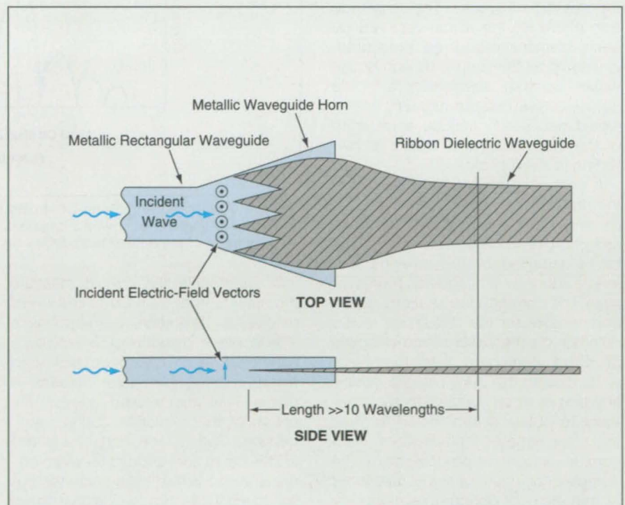
The End of a Dielectric Waveguide Would Be Tapered to a wide, thin, flattened section to enhance coupling of electromagnetic waves from a metal waveguide (or from free space).
