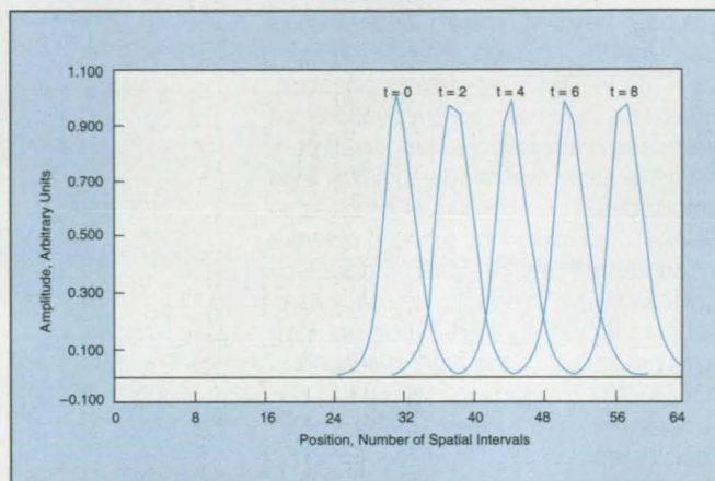
Figure 2. The Numerical Solution obtained by the neural simulation overlaps the exact solution so closely that one cannot distinguish the two solutions from each other on this plot.
