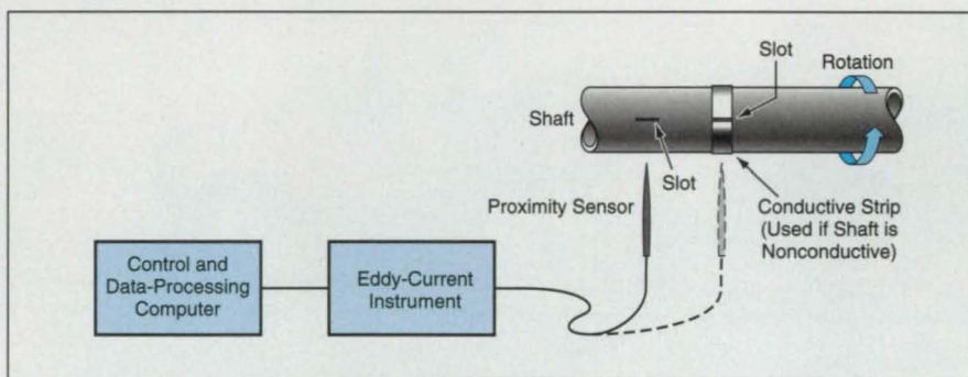
A Noncontact Proximity Sensor — preferably an eddy-current liftoff probe — provides a real-time indication of the wobble of a motor shaft in its bearings.
