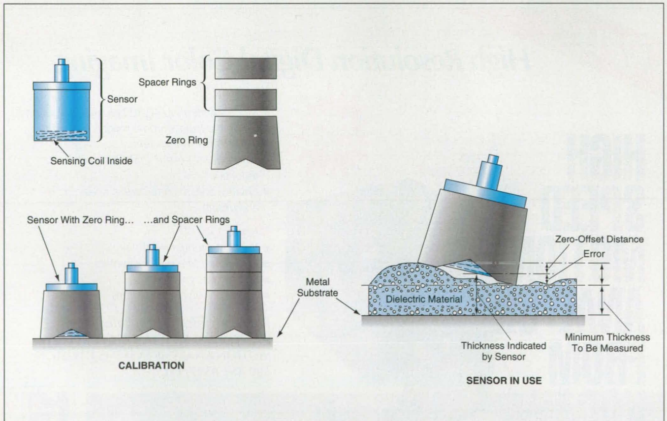
Figure 1. The Thickness Indicated by the Sensor differs from the minimum thickness that one seeks to read when the surface of the dielectric layer is uneven.
