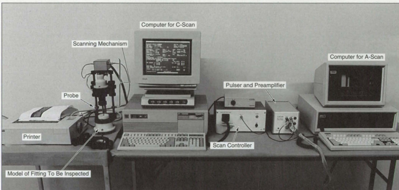
The Ultrasonic-Testing Apparatus is designed specifically for use in inspecting welds in tube fittings. The scanning mechanism is shown here attached to a model of a fitting on the table; in a real inspection, it would be attached to a fitting welded on the end of a tube.
