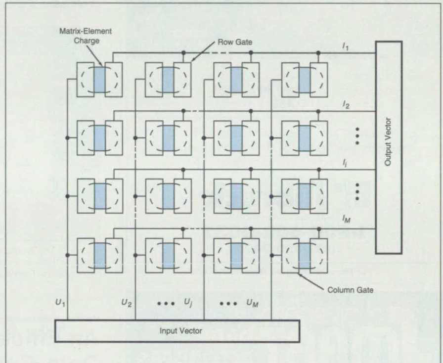
Figure 1. The CCD/CID Processor performs matrix-vector multiplication in one clock cycle.
