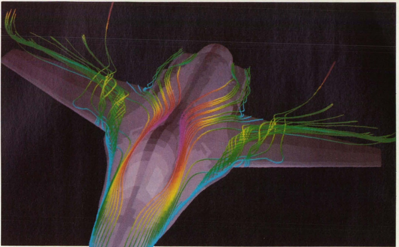
Showing only the most significant surfaces, this computational model simulates airflow around an F-16. To compute the Navier-Stokes equations, a grid is constructed around the aircraft's geometry. The equations are computed at each node (the intersecting lines) of the grid. Increasing the number of nodes gives a more accurate simulation.
