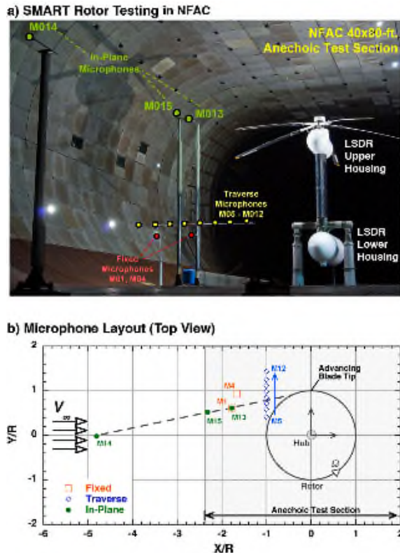
Figure 2. Boeing-SMART rotor: a) installation in wind tunnel, b) microphone layout.
