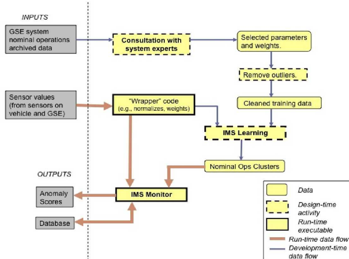
Figure 1. High-level architecture of IMS.
