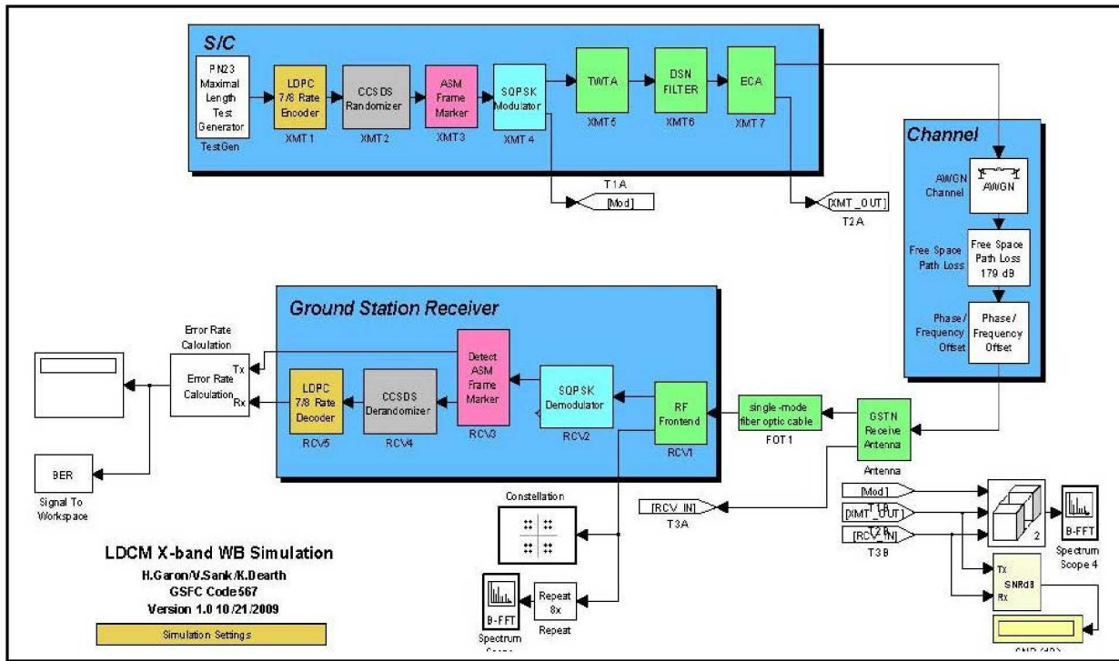
Figure 1. LDCM End-To-End Software Simulation.
