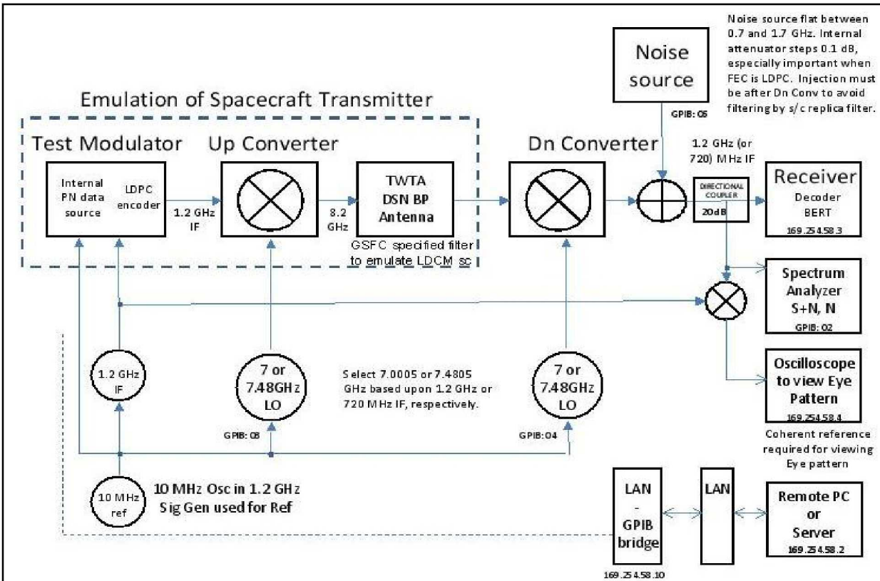
Figure 2. Block diagram of NASA/GSFC LDCM testbench.
