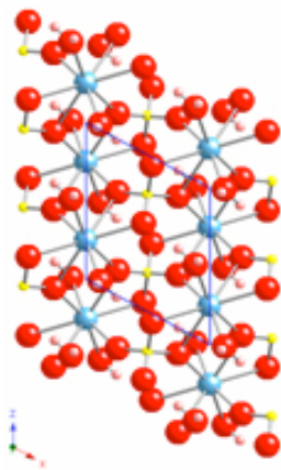
Figure 1: Model of the mineral gypsum ( \text{CaSO}_4 \cdot 2\text{H}_2\text{O} ). Note repetition of the structural elements.
