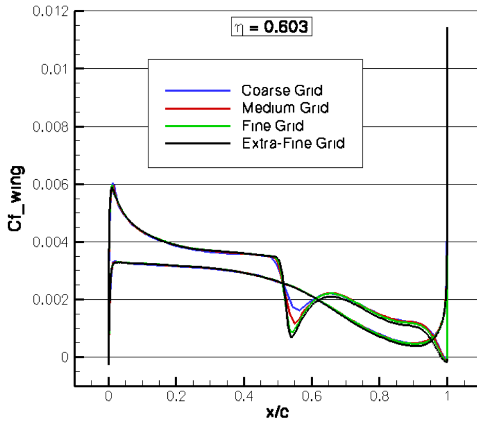
Figure 11. Grid convergence of CRM wing chordwise skin friction distribution at M_\infty = 0.85 , Re_c = 5 \times 10^6 .
