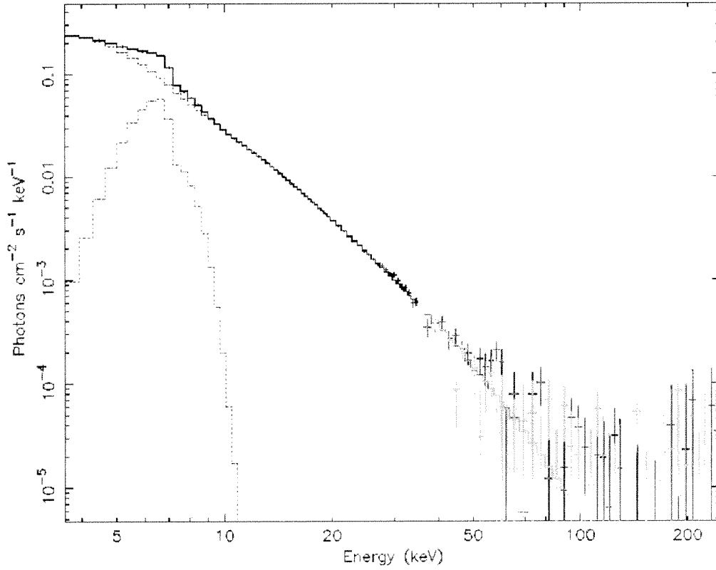
Fig. 3.— Example of one of our satisfactory model fits to the data as described in section 2. Here the spectral index is hard, \sim 1.5 , well below the saturation level but within the expected range. In this case the model fits the data at an acceptable level and the mass-estimation parameters are well defined.
