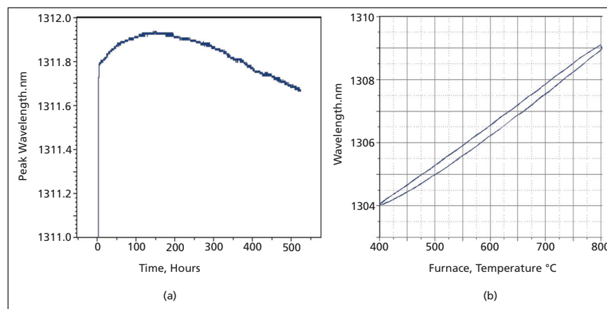
Figure 2. Performance Characteristics: (a) Wavelength stability of a sensor exposed to 1,000 °C for 500 hours and (b) wavelength readings as a function of temperature during thermal cycling from 400 to 800 °C.
