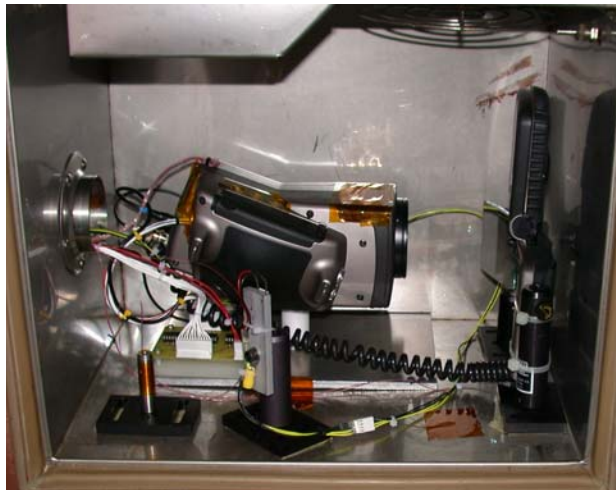
Figure 4. Tenney Oven Evaluation of the FLIR S60
