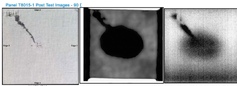
Figure 10a. Damaged RCC specimen: visible image, ultrasound image, processed IR image at 1100\text{W}/\text{m}^2
