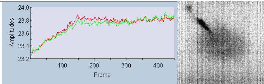
Figure 10b. Signal level per frame and processed IR image at 225 W/m 2
