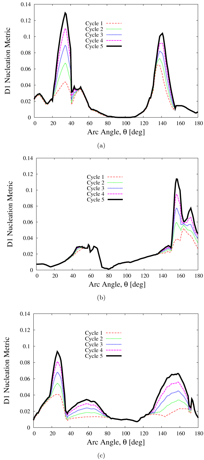
Figure 8. D_1 localization and accumulation along an arc with radius of 25% of crack dimension, a , for the three simulated grain Orientations (a) A (b) B (c) C.
