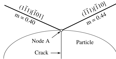
(d) Illustration of the 2 slip systems with the highest Schmid factor, m , in Orientation B
