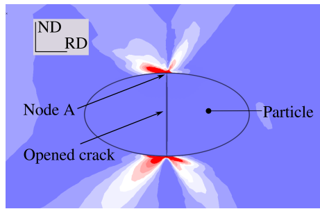
(c) D_1 metric color contour for Orientation B
