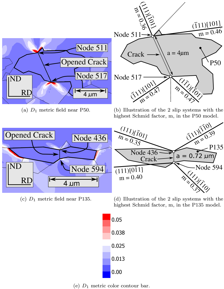
Figure 12. Comparison of (a) P50 and (b) P135 D_1 fields at first peak load.
