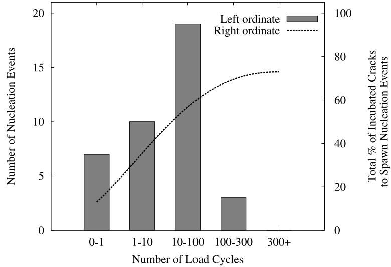
Figure 2. A histogram of the cycles at which nucleation events occurred for the AA 7075-T651 DEN specimen. Approximately 73% of the observed incubated cracks led to nucleated cracks into a surrounding grain.
