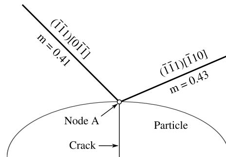
(f) Illustration of the 2 slip systems with the highest Schmid factor, m , in Orientation C
