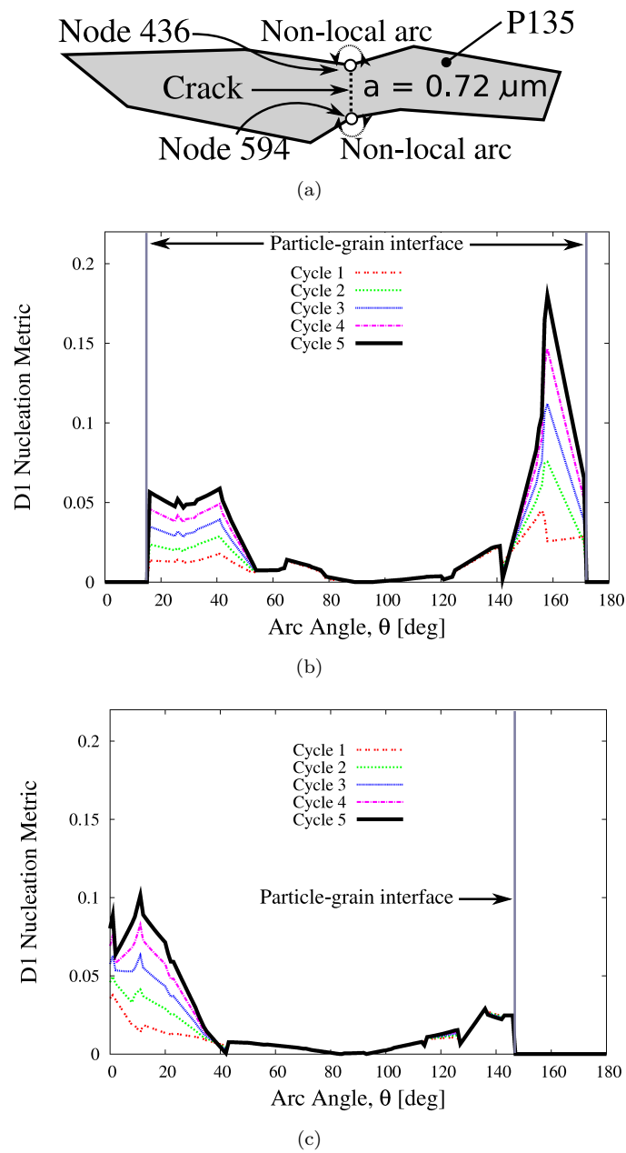
Figure 14. Accumulation of the D_1 metric within the P135 model at both crack front points that intersect the free surface, (a) P135 outline showing the non-local arc (b) Node 436 (c) Node 594. These data were extracted along a non-local arc with a radius of 25% of the crack dimension, a , 0.18 \mu\text{m} .
