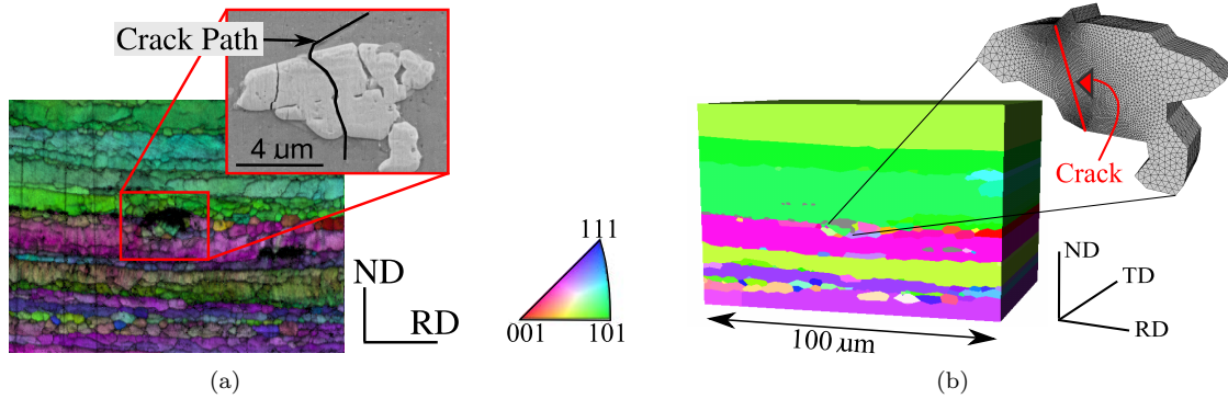
Figure 10. The P50 2.5-D finite element model, generated from experimental data, shown with inverse pole figure [100] color contour map. (a) Inverse pole figure with detail of \text{Al}_7\text{Cu}_2\text{Fe} particle region. (b) Corresponding finite element model with zoom on meshed, cracked particle.
