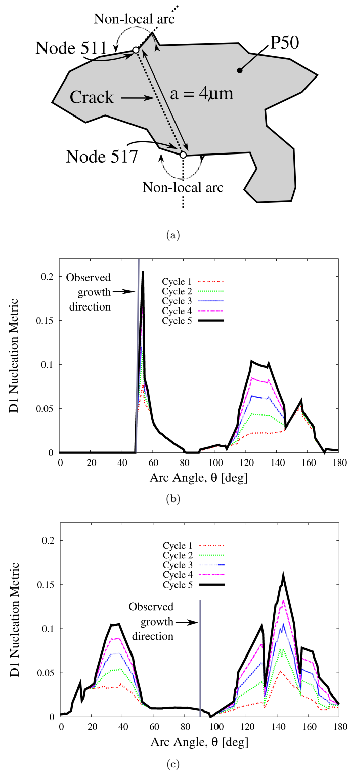
Figure 13. Accumulation of the D_1 metric within the P50 model at both crack front points that intersect the free surface, (a) P50 outline showing the non-local arc (b) Node 511 (c) Node 517. These data were extracted along a non-local arc with a radius of 25% of the crack dimension, a , 1.0\ \mu\text{m} .
