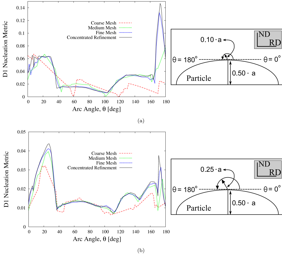
Figure 5. D_1 nucleation metric versus arc angle at four levels of mesh refinement for arc radii equal to (a) 10% and (b) 25% of the crack dimension, a . These results were taken from Orientation C. Note the difference in ordinates.
