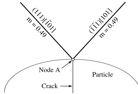
(b) Illustration of the 2 slip systems with the highest Schmid factor, m , in Orientation A.
