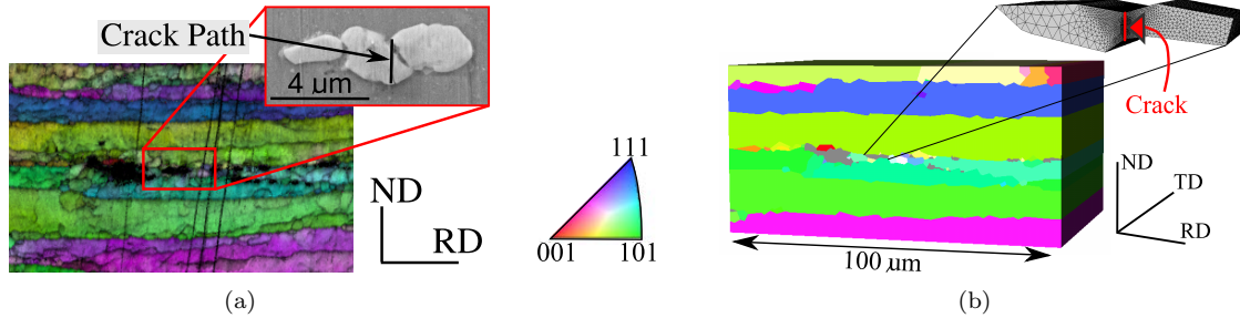
Figure 11. The P135 2.5-D finite element model, generated from experimental data, shown with inverse pole figure [100] color contour map. (a) Inverse pole figure with detail of \text{Al}_7\text{Cu}_2\text{Fe} particle region. (b) Corresponding finite element model with zoom on meshed, cracked particle.
